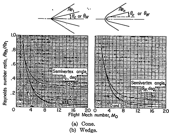
FIGURE 2.—Effect of blunting on Reynolds number near surface of cone and wedge. Ambient static temperature, 392.4° R.
