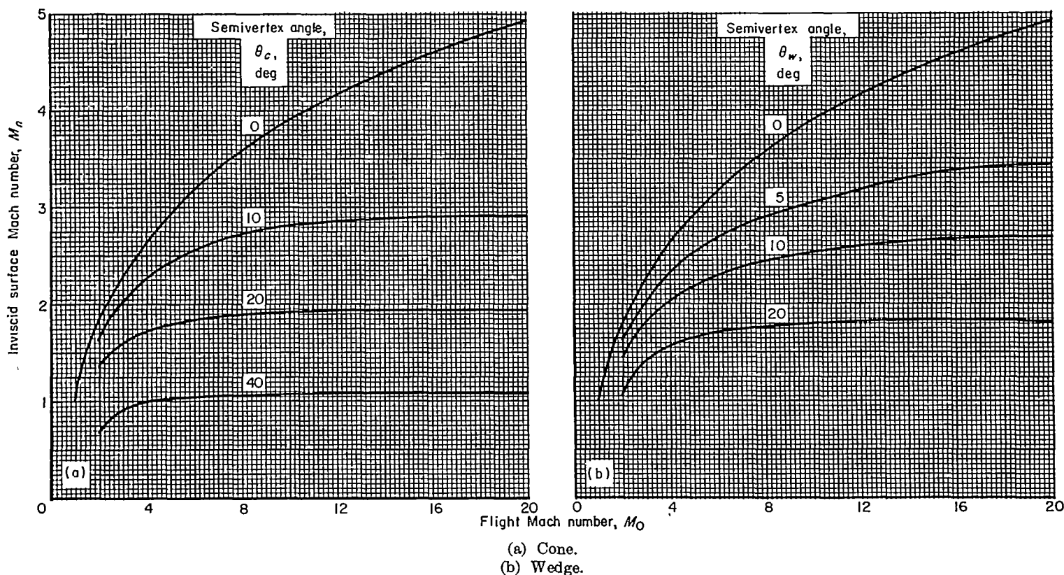
FIGURE 1.—Inviscid surface Mach number for blunted cone and wedge.
