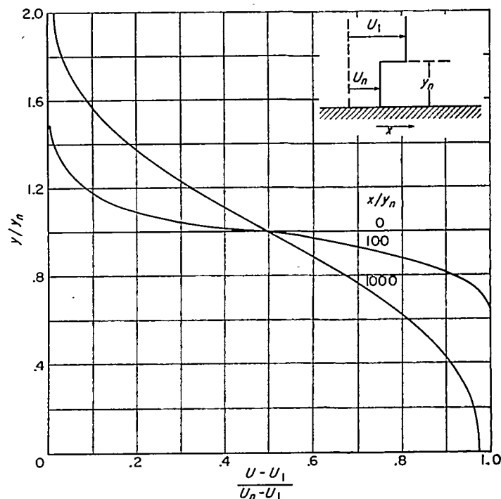
Figure 8.—Laminar diffusion of step velocity profile. Re_{y_n} = \frac{\rho_1 U_1 y_n}{\mu_1} = 10^4 .
