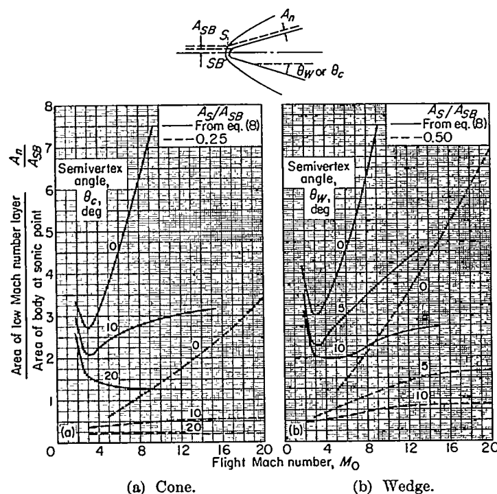
FIGURE 3.—Area of low Mach number layer for blunted cone and wedge.
