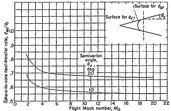
FIGURE 7.—Comparison of laminar heat-transfer rates for spherical and conical noses. Surface-to-ambient static-temperature ratio, 1.0.
