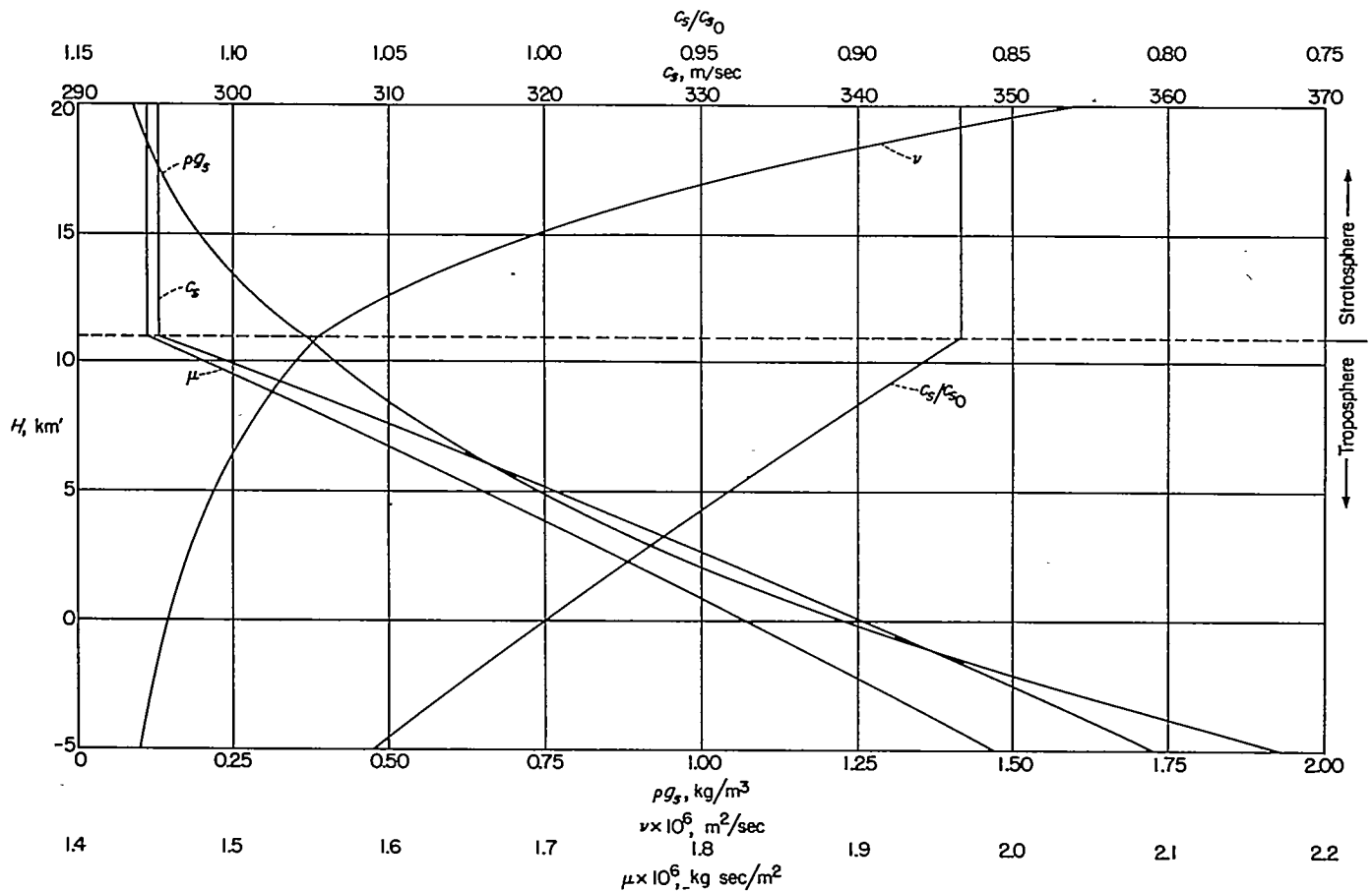
METRIC FIGURE II.—Specific weight \rho g_s , viscosity \mu , kinematic viscosity \nu , sound speed c_s , and sound-speed ratio c_s/c_{s0} against geopotential H .
