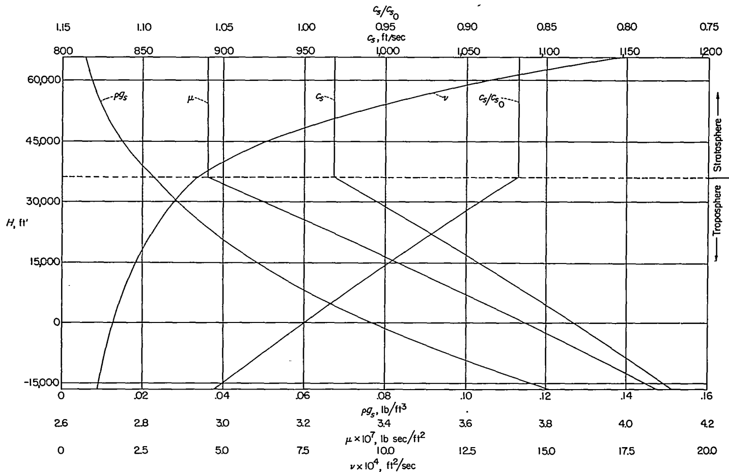
ENGLISH FIGURE II.—Specific weight \rho g_s , viscosity \mu , kinematic viscosity \nu , sound speed c_s , and sound-speed ratio c_s/c_{s0} against geopotential H .
