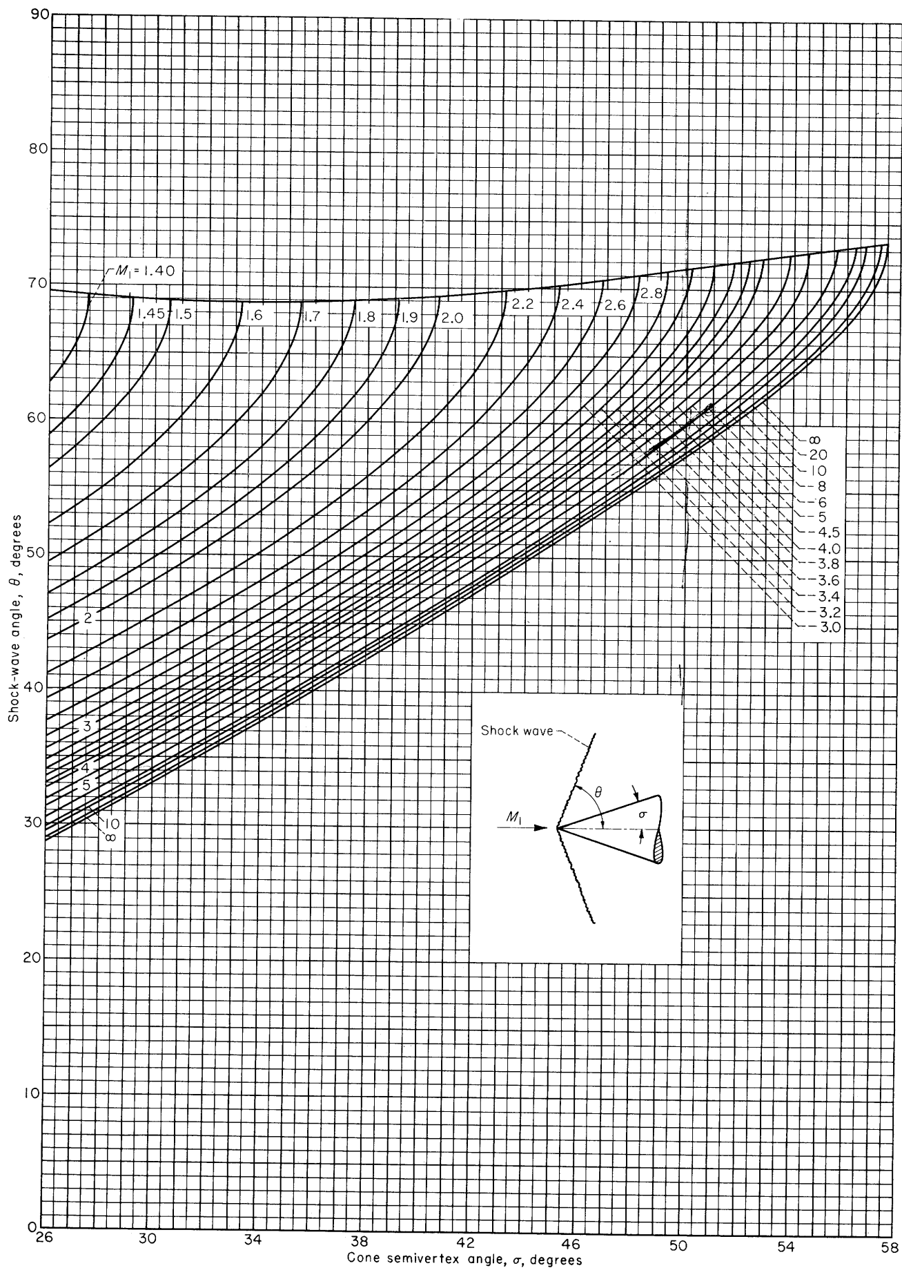
CHART 5.—Concluded
