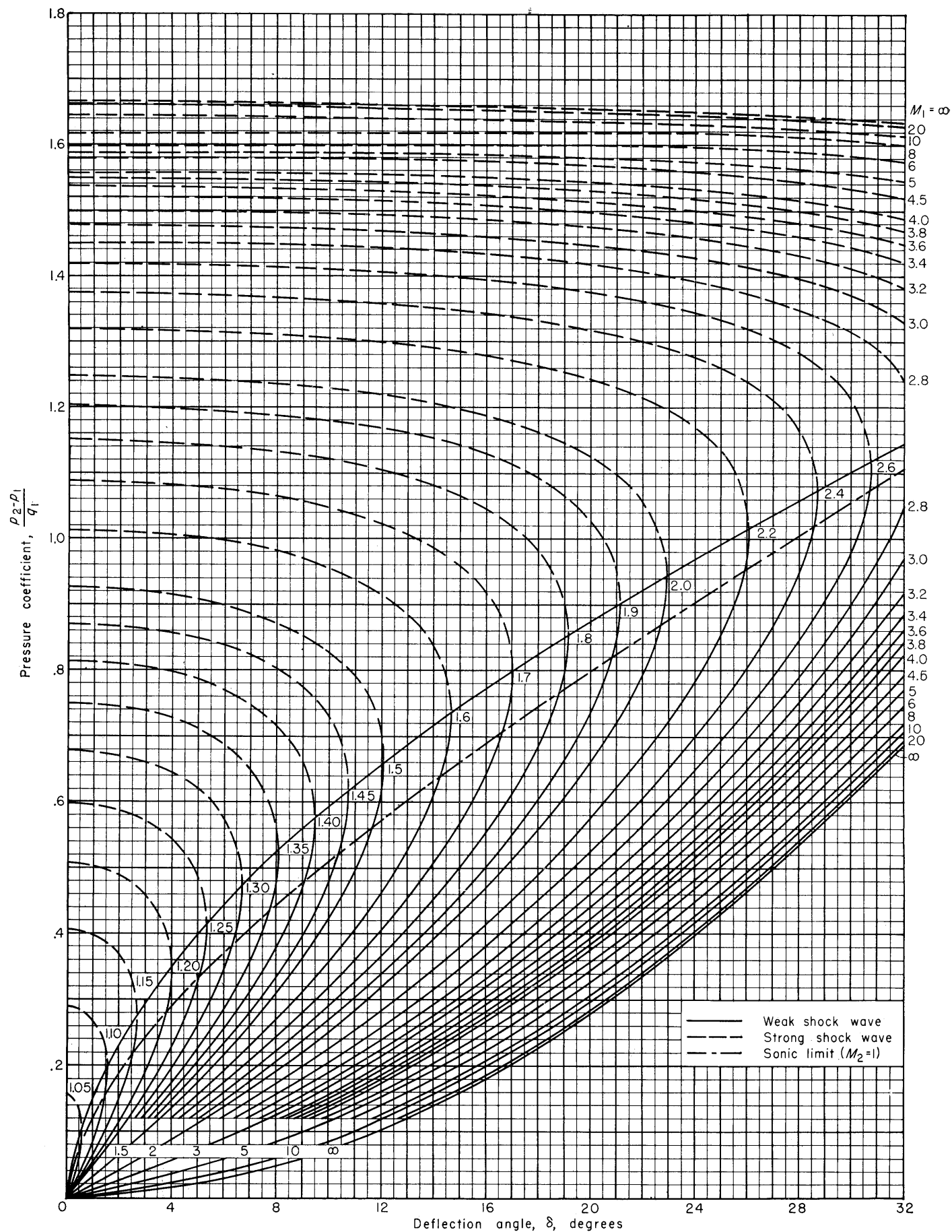
CHART 3.—Variation of pressure coefficient across shock waves with flow-deflection angle for various upstream Mach numbers. Perfect gas, \gamma = 7/5
