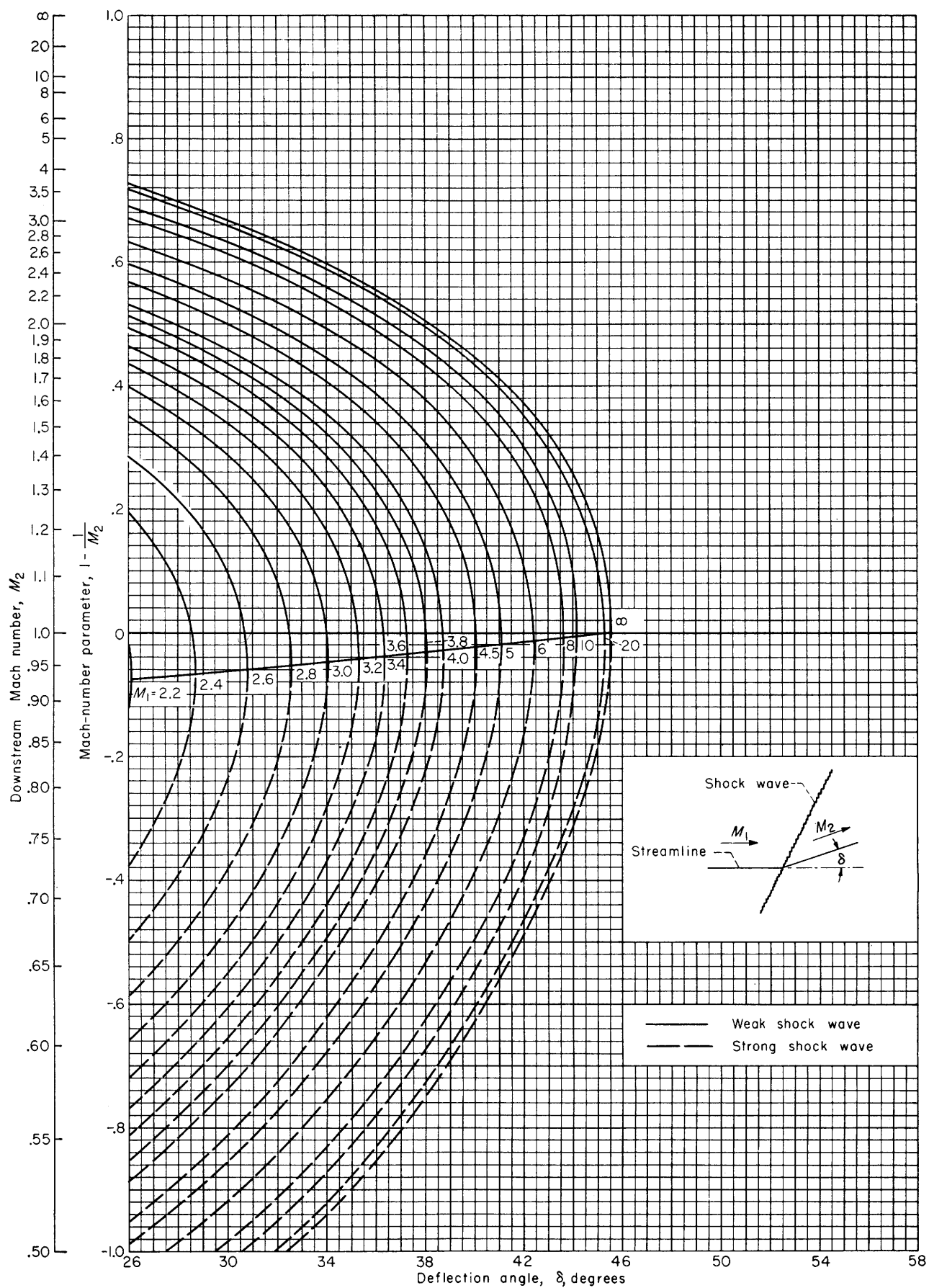
CHART 4.—Concluded
