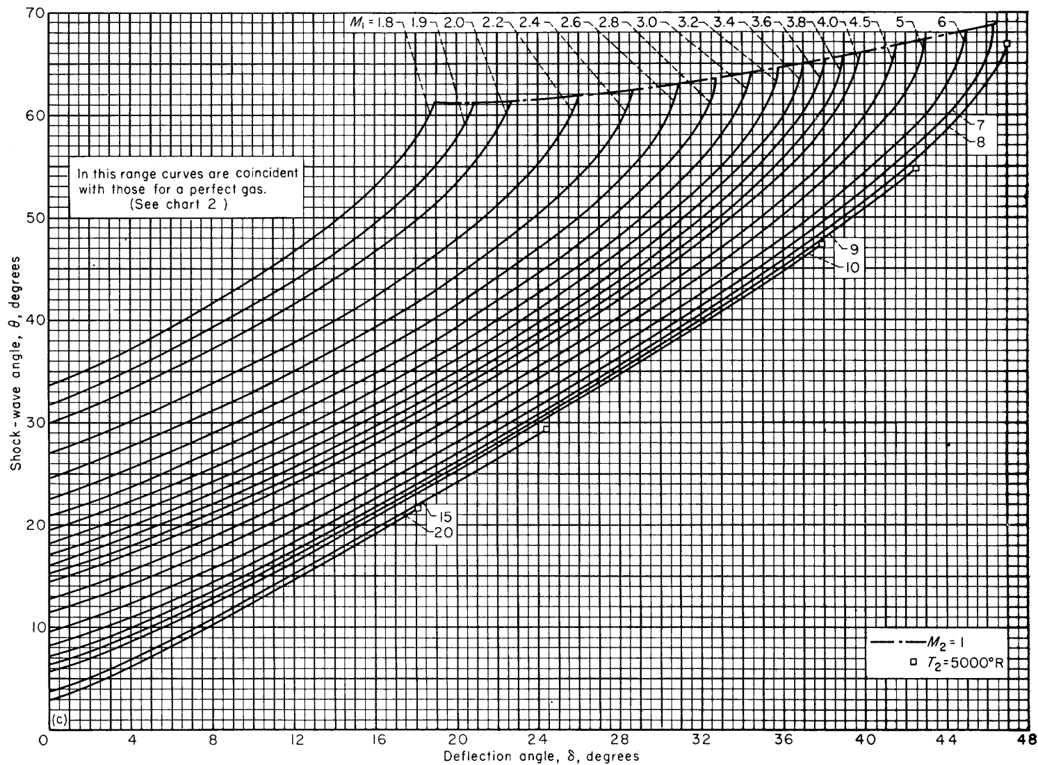
CHART 21.—Continued
