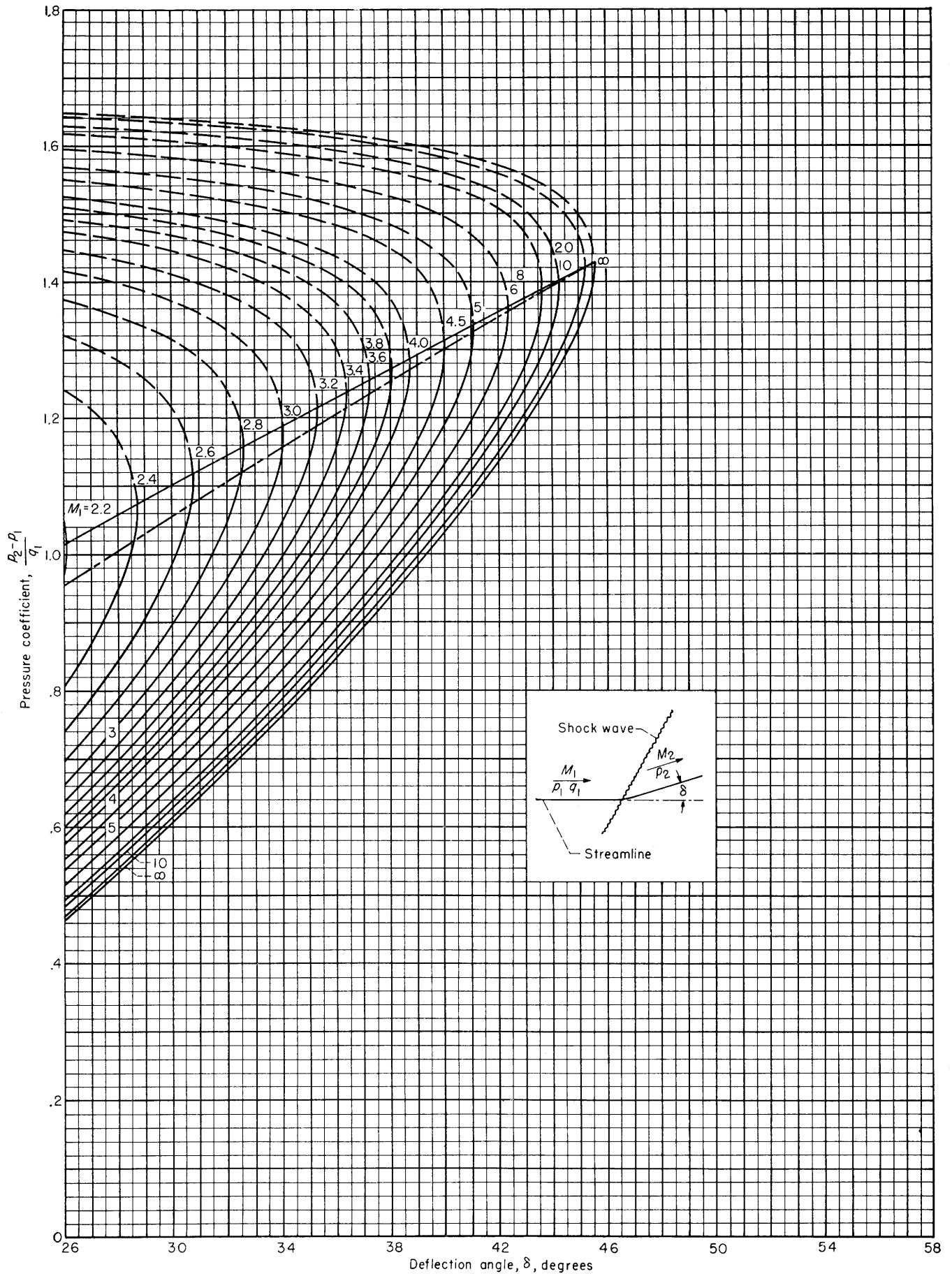
CHART 3.—Concluded
