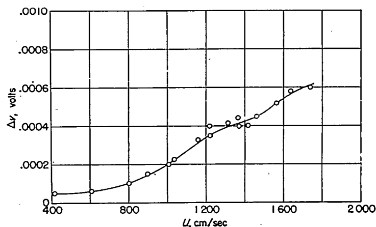
FIGURE 13.—Correction for deflection of flat plate.
