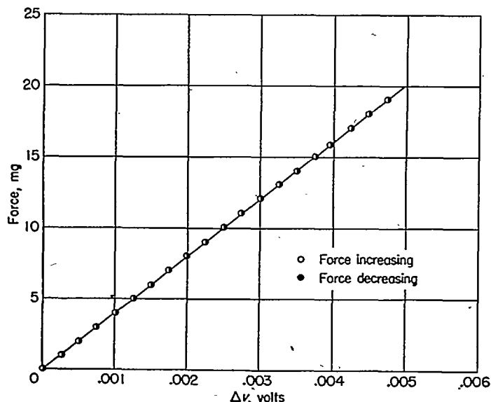
FIGURE 8.—Calibration of skin-friction instrument. Input, 5 volts at 20 kilocycles; 0.0005- by \frac{1}{4} -inch links; r_s = 39.25 \times \Delta , dynes per square centimeter.
