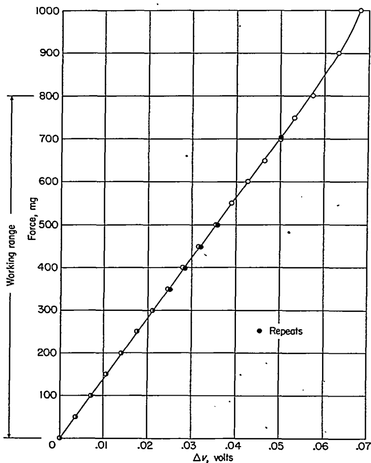
FIGURE 9.—Calibration curve of skin-friction instrument. 0.01- by \frac{1}{4} -inch steel links; r_s = 38.3 \times 10^6 \times \Delta , dynes per square centimeter.
