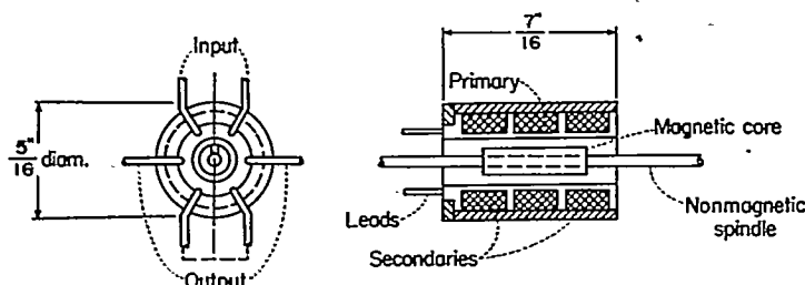
FIGURE 4.—Differential transformer.
