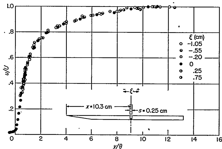
FIGURE 3.—Velocity profiles on flat plate with turbulent boundary layer and slot. Re_s \approx 4 \times 10^4 ; Re_\theta \approx 1000 .
