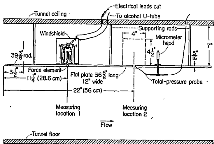
FIGURE 11.—Sketch of flat-plate installation in GALCIT 2 1/4 by 2 1/4-foot correlation tunnel.
