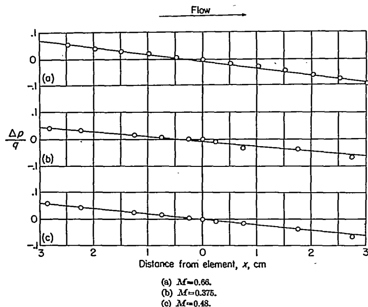
FIGURE 20.—Representative pressure distributions on flat plate with laminar boundary layer. Subsonic flow.
