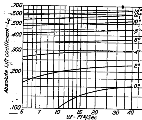
FIG. 4.—Variation of Lift coefficient with V_L Re-plot of figure 19, B. A. C. A. R. & M. No. 450. (See Fig. 1.)
