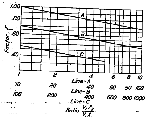
FIG. 8.—Evaluation of F = \left( \frac{V_{2L}}{V_{1L}} \right)^{-0.18}
