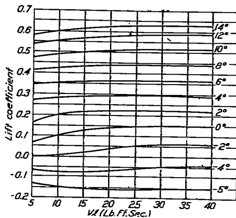
FIG. 1.—Correction to lift coefficient for scale effect. Reproduction of figure 19, B. A. C. A. R. & M. No. 450.
