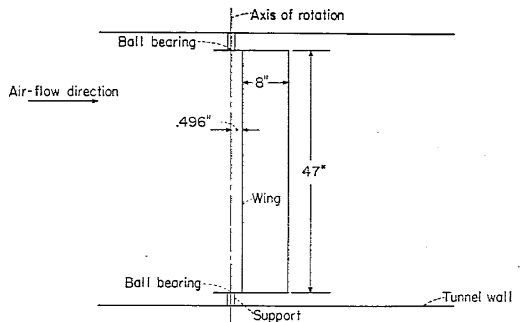
FIGURE 6.—Diagram of model and model installation. Inertia of system about axis of rotation I_a = 0.0948 foot-pound-seconds square per foot; natural frequency of system \omega_n = 22.99 .
