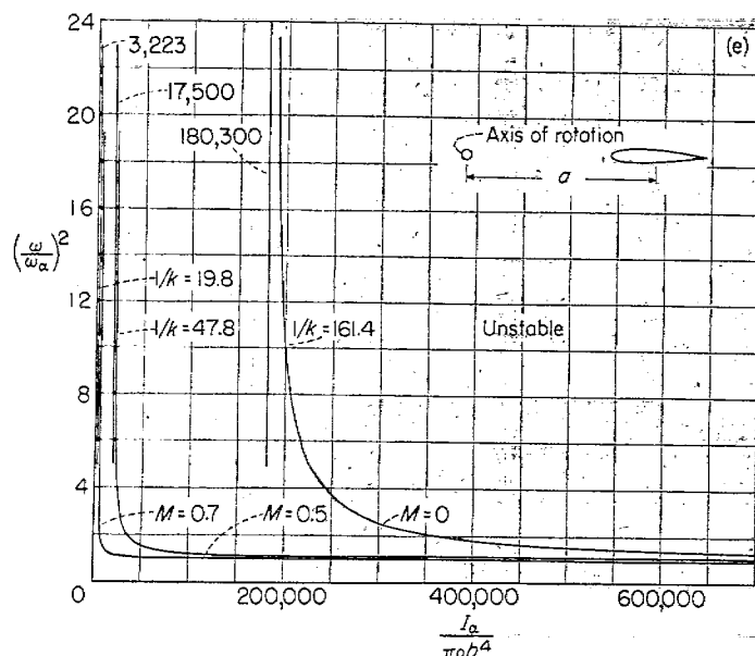
(e) \alpha = -4.0 . FIGURE 2.—Continued.
