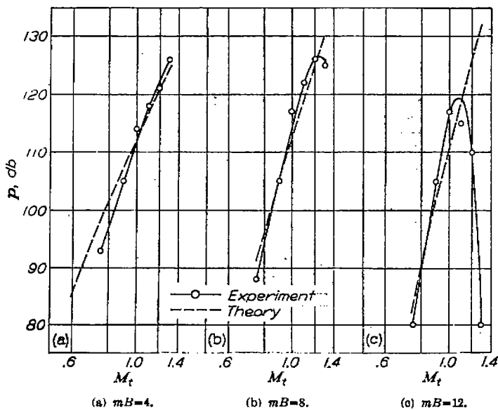
FIGURE 10.—Sound pressure in decibels as a function of tip Mach number for three harmonics of a two-blade propeller. \beta_{0,11}=15^\circ ; \theta=90^\circ ; and r=30 feet.
