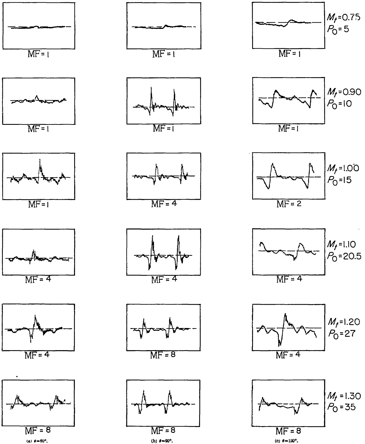
FIGURE 5.—Cathode-ray oscillograph pictures of sound-pressure wave forms at various azimuth angles and propeller tip Mach numbers. \beta_{0.75} = 13^\circ ; r = 30 feet; B = 2 .
