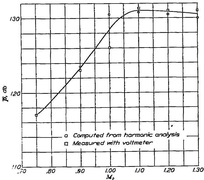
FIGURE 7.—Effect of tip Mach number at constant power on the over-all sound pressure in decibels. \theta=90^\circ ; B=2 ; P_H=30 ; distance from the center of rotation is equal to 7.5 diameters.
