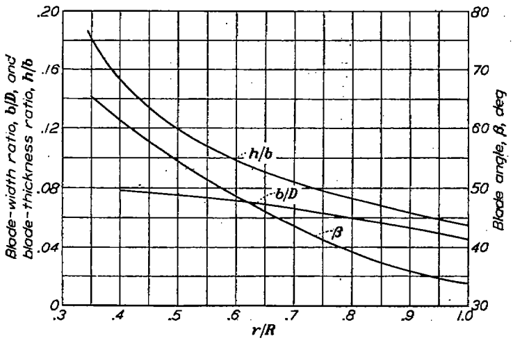
FIGURE 1.—Blade-form curves for test propeller.
