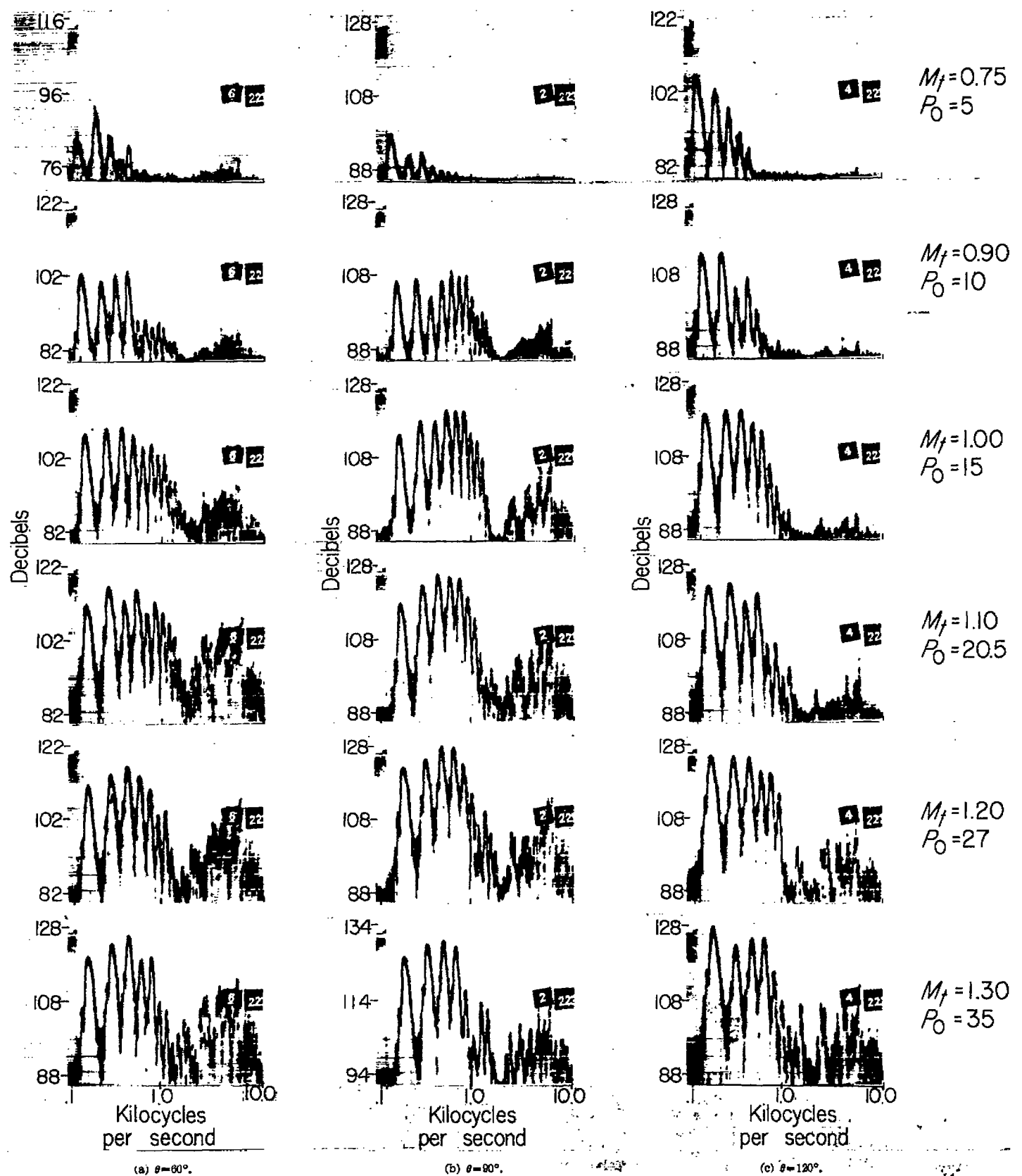
FIGURE 4.—Panoramic Sonic Analyzer sound spectrums at various azimuth angles and propeller tip Mach numbers. B_1 r_1 = 18^\circ ; r = 30 feet; B = 2 . ( P_0 is defined as hp per sq ft of disk area.)
