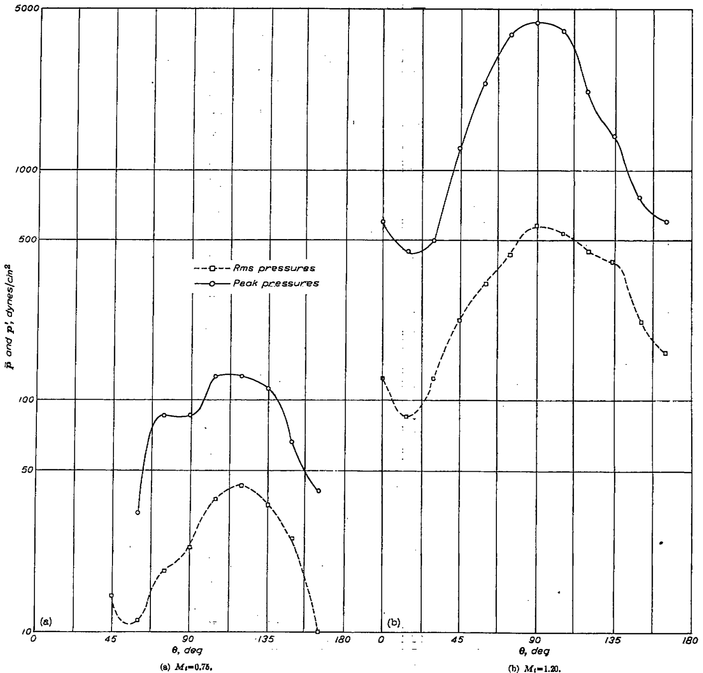
FIGURE 6.—Root-mean-square and peak sound pressures in dynes per square centimeter as a function of azimuth angle for a two-blade propeller. \beta_{0.75} = 15^\circ ; s = 30 feet.
