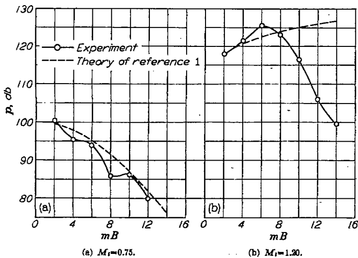
FIGURE 9.—Sound pressure as a function of order of the harmonic. B=2 ; r=30 feet; \beta_{0,11}=15^\circ ; \theta=90^\circ .
