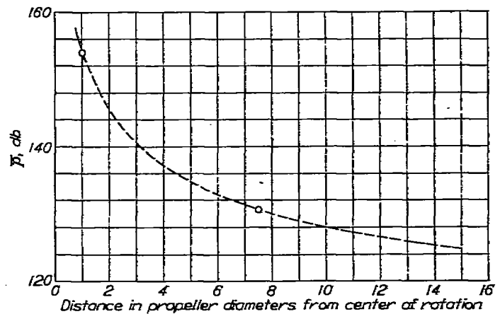
FIGURE 8.—Sound pressure as a function of distance for a two-blade propeller. \beta_0=15^\circ ; \theta=90^\circ ; M_t=1.20 ; P_H=30 .
