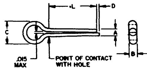
EXTENDED PRONG SQUARE CUT (PLAN) (SEE NOTE 2)
