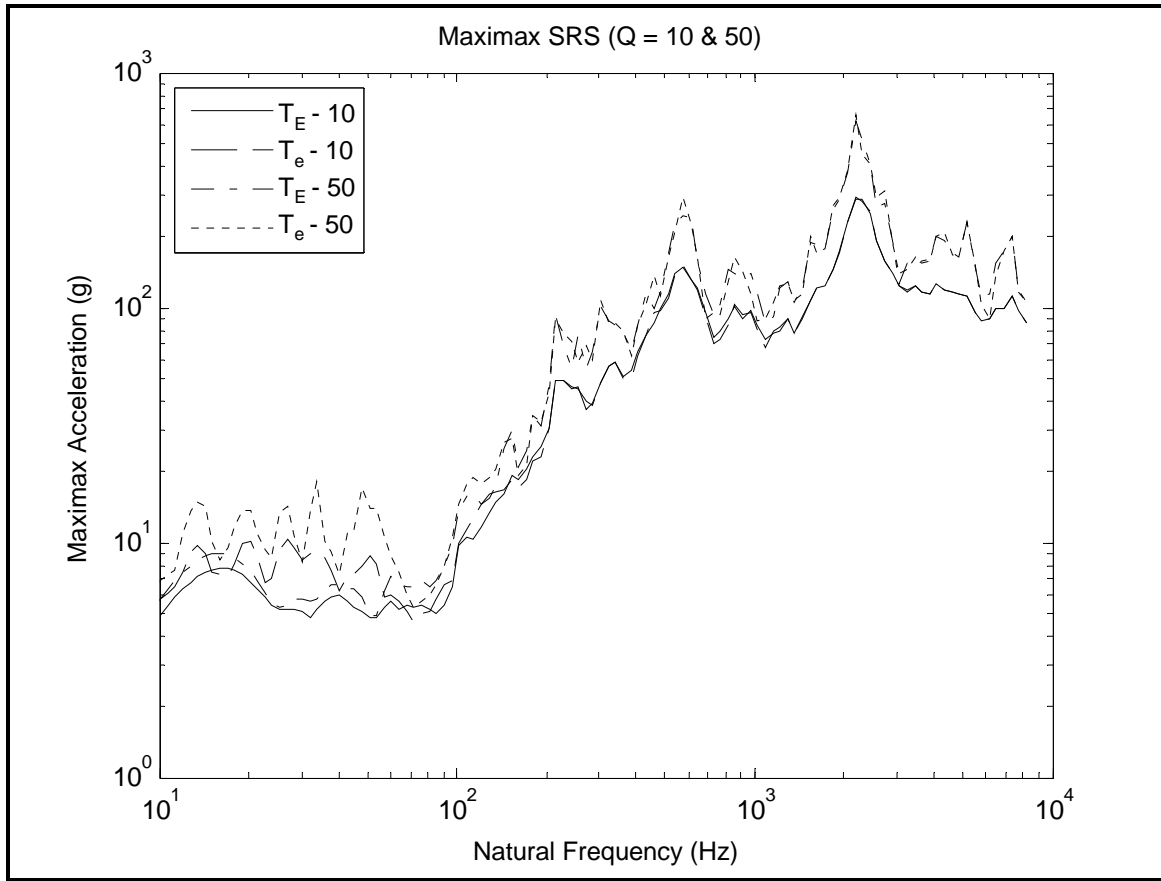
Figure 516.6-5. Maximax Acceleration SRS over T_E and T_e for Dynamic Quality Factor Q 's of 10 and 50.
