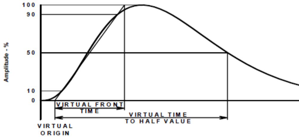
FIGURE 6. Standard current impulse waveshape.
