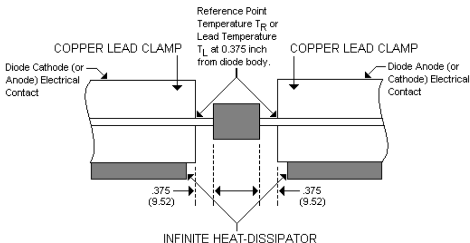
FIGURE 4081-2. Axial-leaded mounting arrangement.
