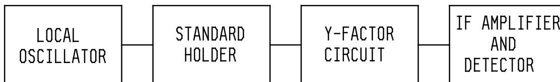
FIGURE 4121-2. Y-factor method.
