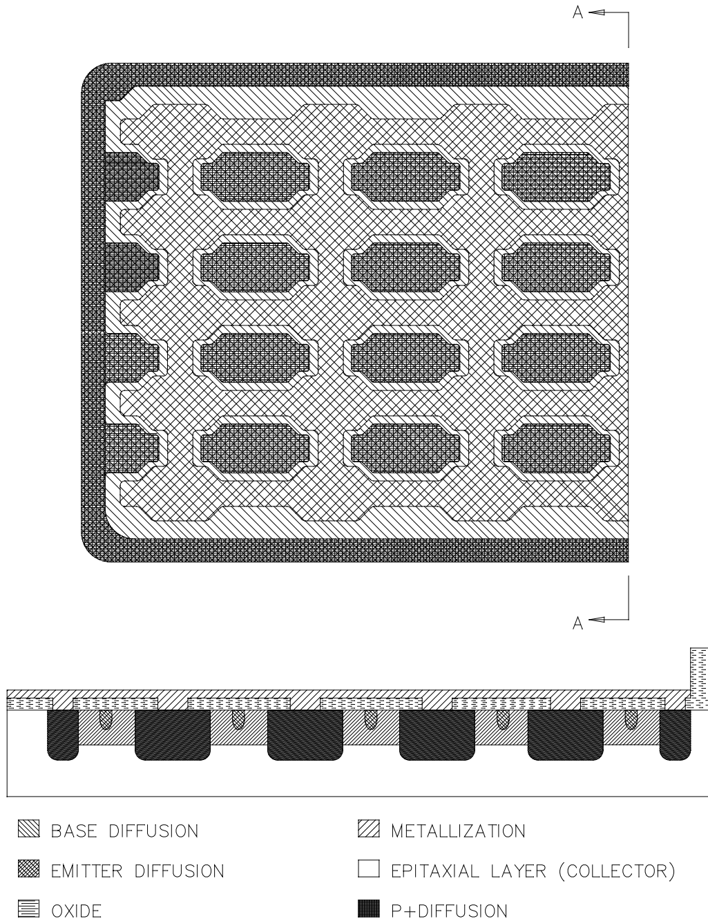
FIGURE 2070-5. Mesh geometry.
