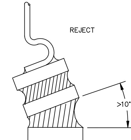
FIGURE 2074–G4. Element tilt.
