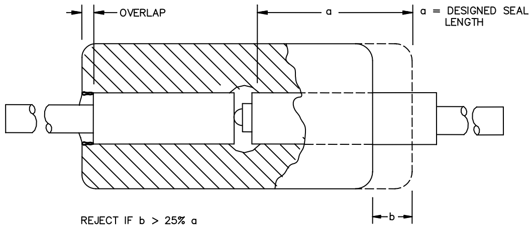
FIGURE 2074-C2. High seal .
