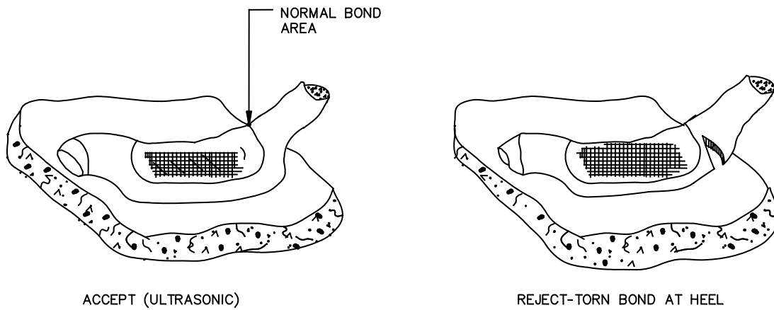
FIGURE 2069-2. Torn bonds.
