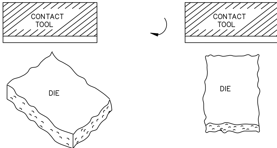
FIGURE 2017-2. Rotational capability.
