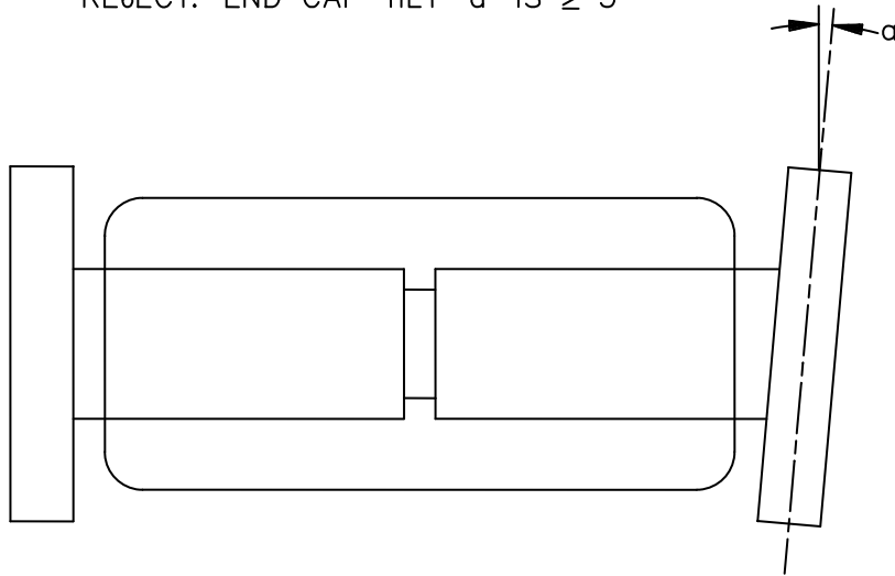
FIGURE 2074-D5. Tilt.
