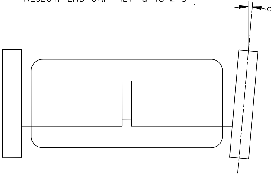
FIGURE 2074-D11. End-cap tilt.
