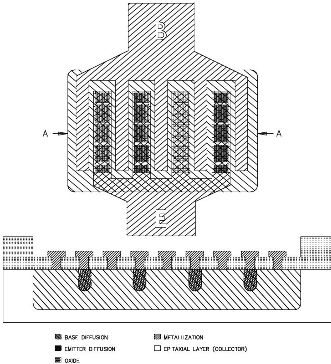
FIGURE 2070-6. Interdigitated geometry.
