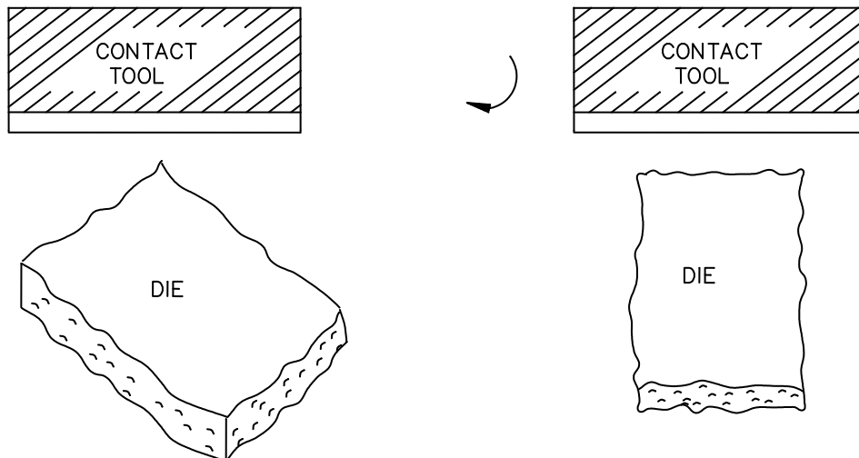
FIGURE 2017-2. Rotational capability.
