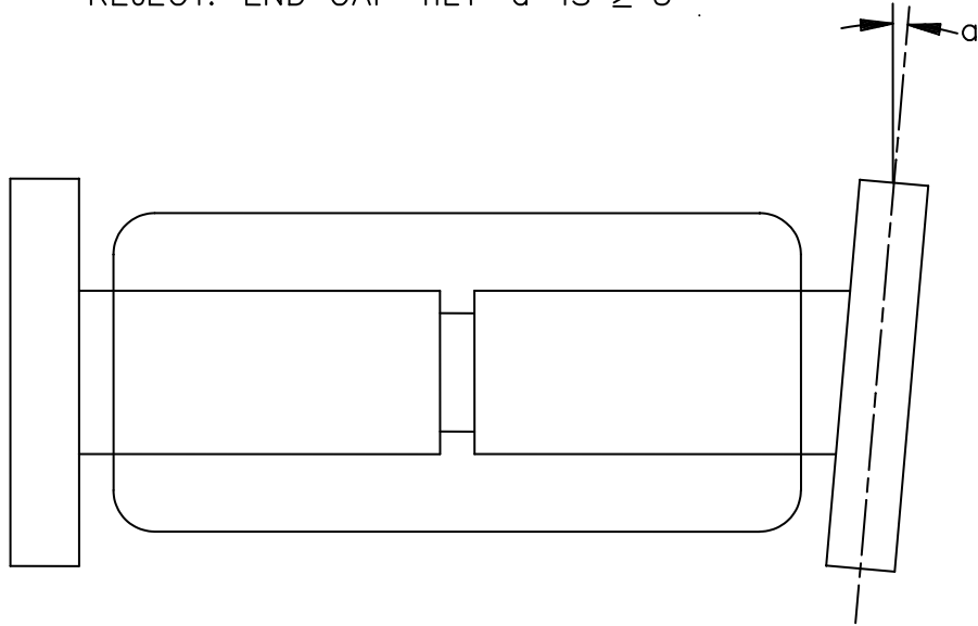
FIGURE 2074-D11. End-cap tilt.
