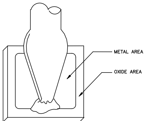
FIGURE 2074-B5. Solder overflow.
