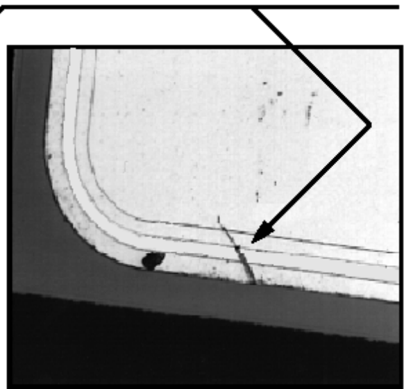
FIGURE 2078-1. Metallization scratches and voids.
