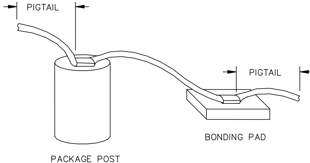
FIGURE 2078-8. Pigtail length.
