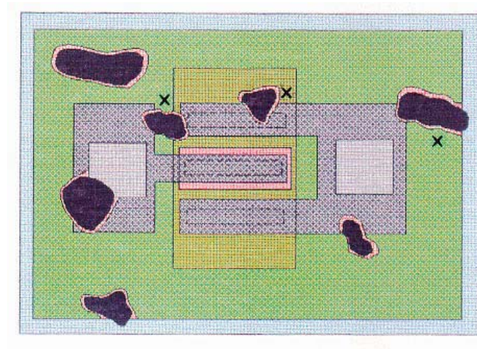
FIGURE 2072-42. Glass-embedded foreign particles on the die that bridge paths or junctions.
