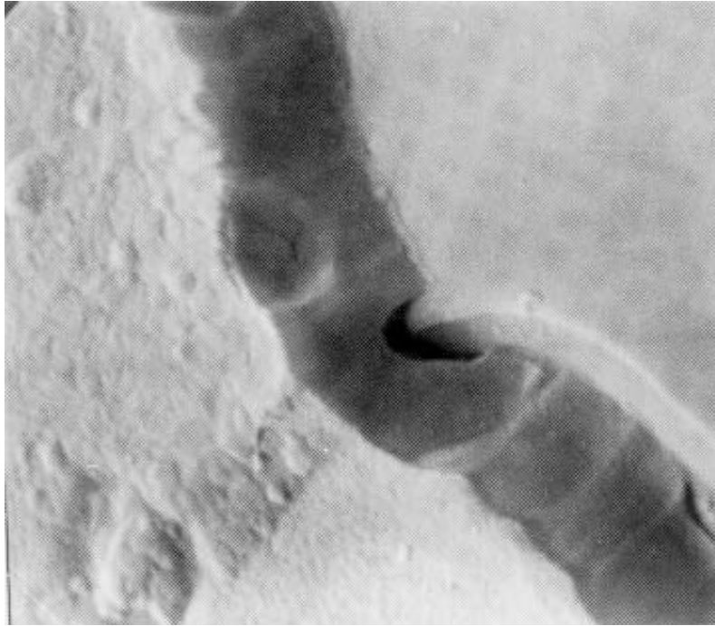
FIGURE 2077-8. Tunnel/cave at oxide step at 10,000X (accept).
