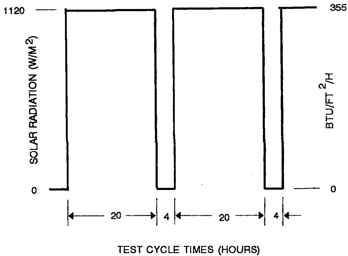
FIGURE C10-2. Two Steady State Cycles
