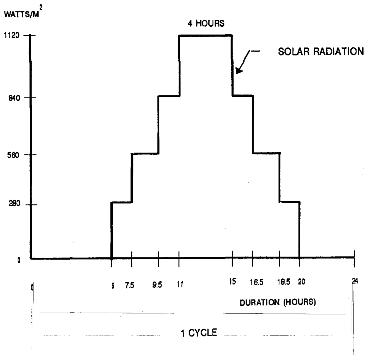
FIGURE C10-1. Simulated Solar Radiation Cycle C10-7
