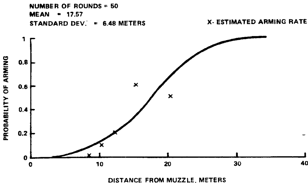
Figure D2-1. Estimated Probability of Arming Versus Distance from Muzzle (Probit Method).
