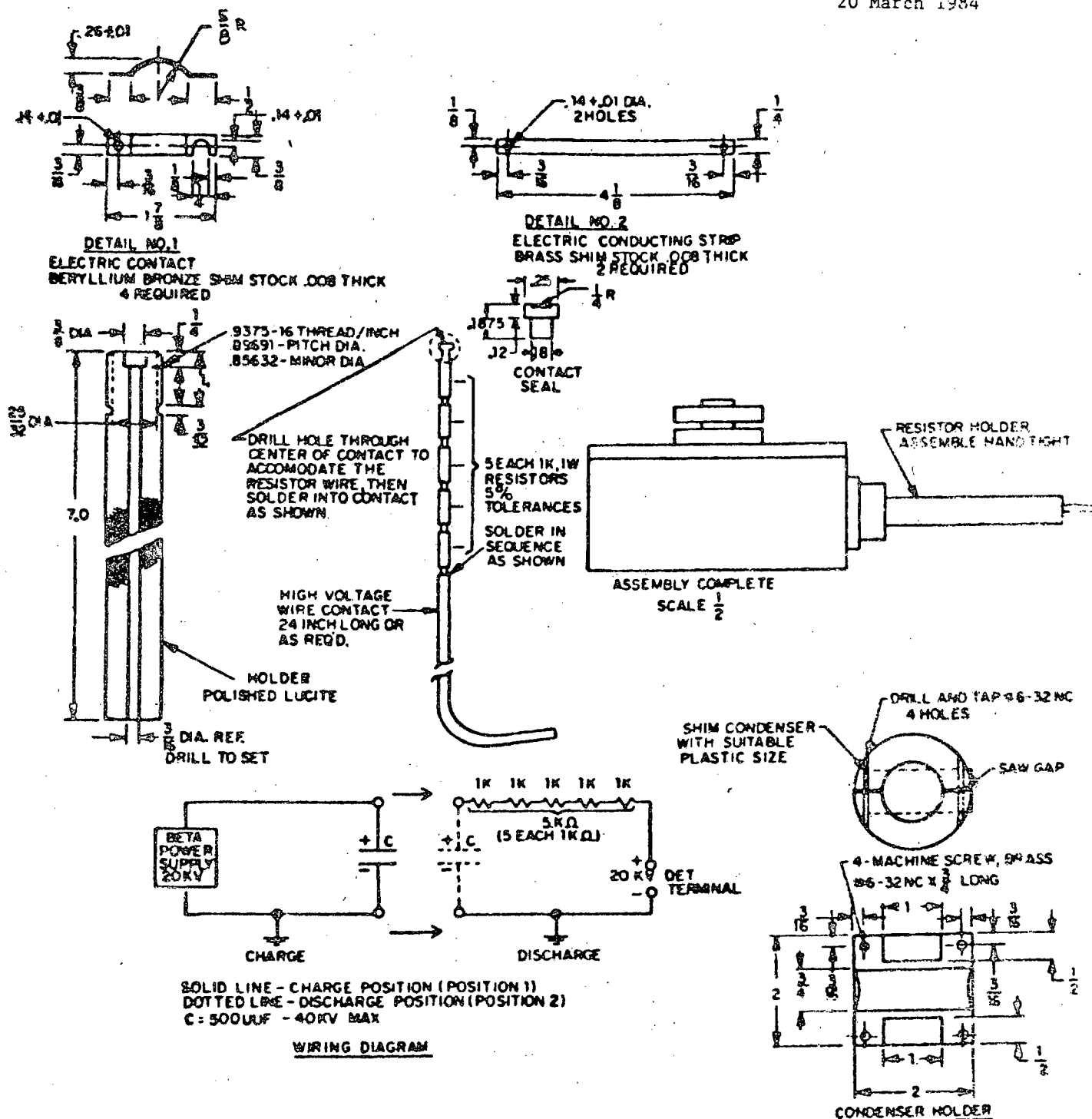
FIGURE 7. Wiring diagram and condenser holder.
