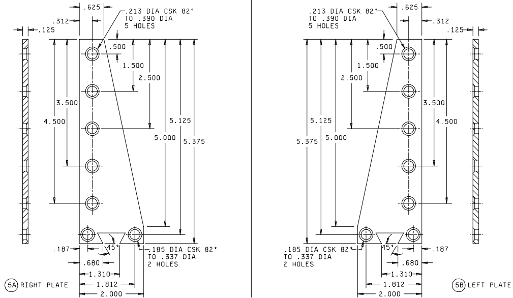
FIGURE 7. RF-dc insertion loss measuring equipment assembly - Continued.
