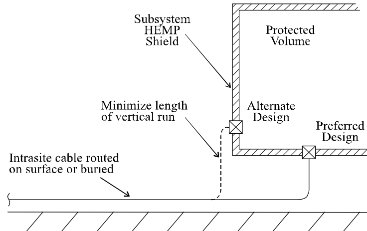
FIGURE 2. Penetration entry area placement.
