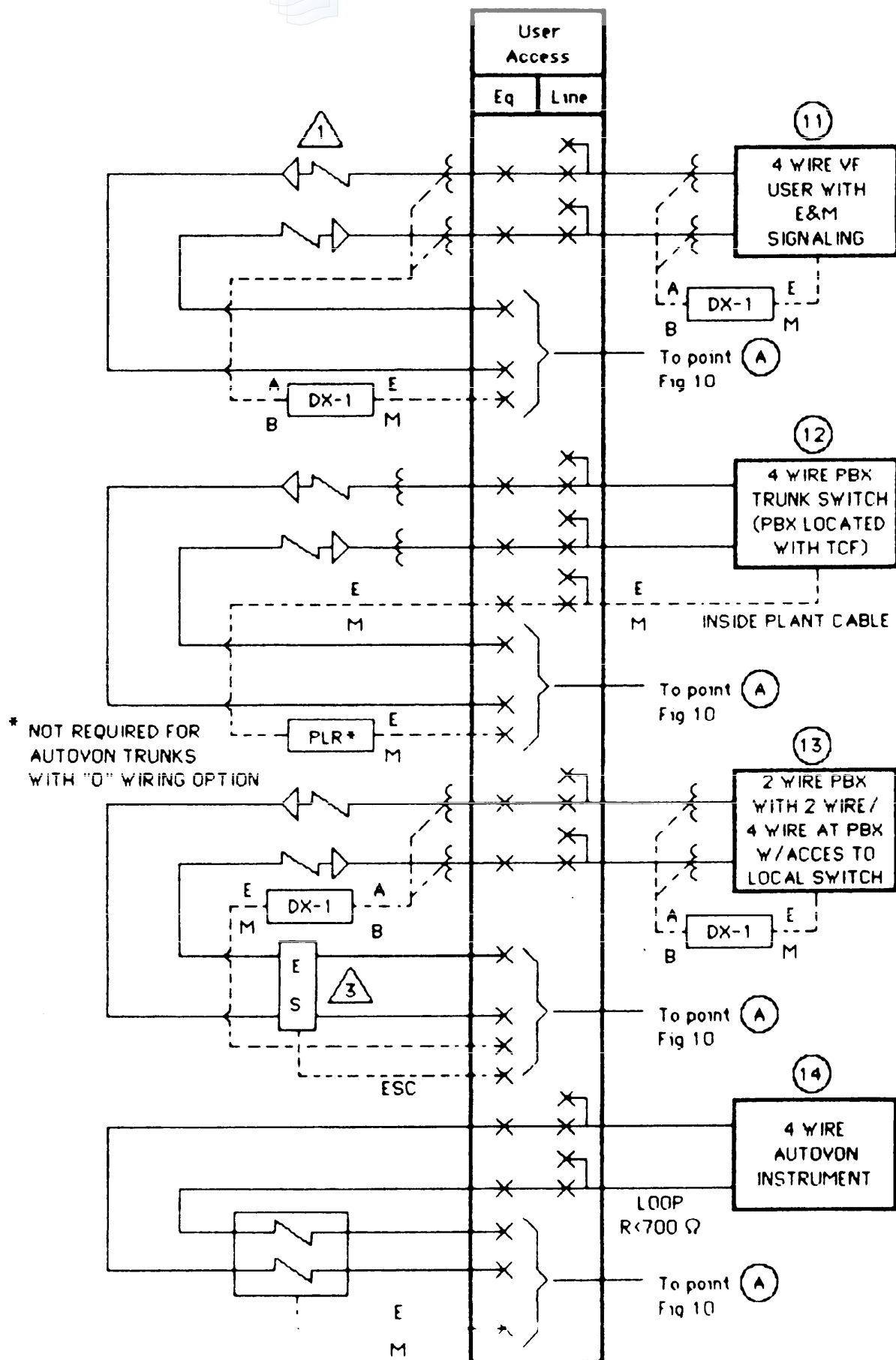
FIGURE 9 AUTOVON users collocated with TCF and AUTOVON switch
