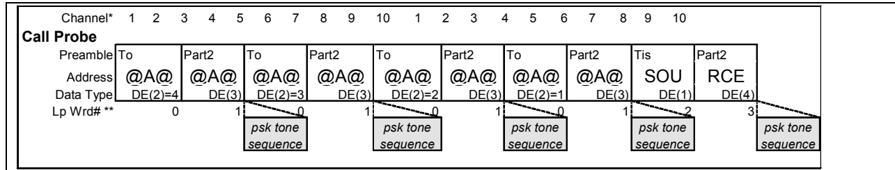
FIGURE A-55. Example AllCall frame format.
