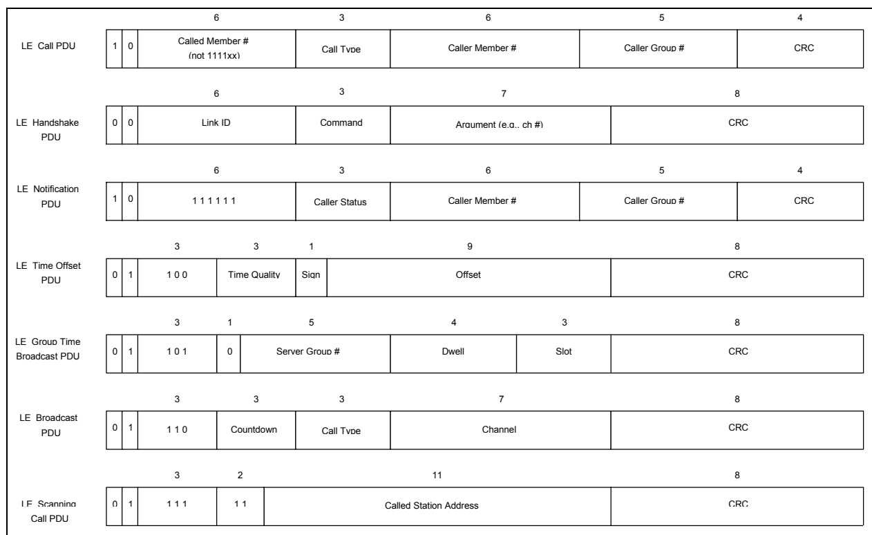
FIGURE C-17. 3G-ALE PDUs.
