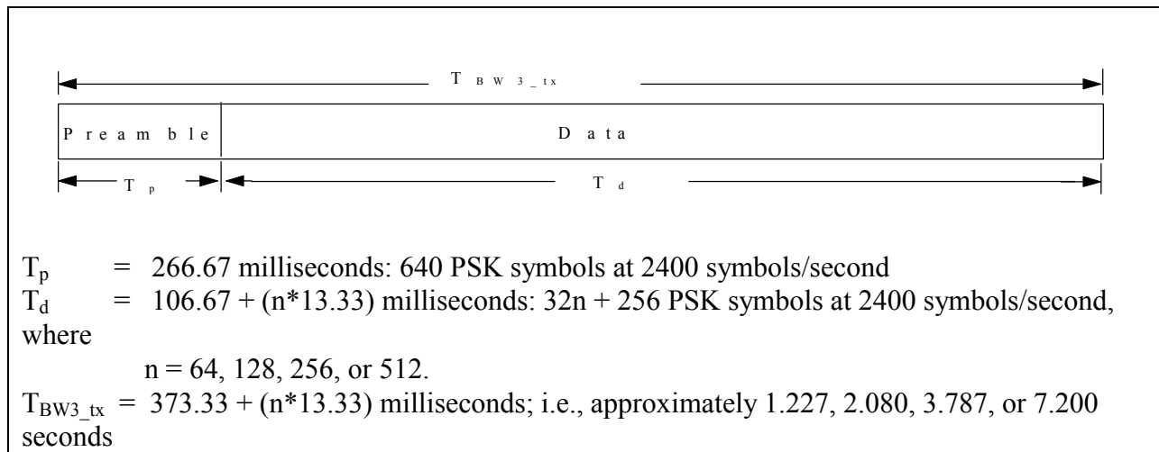
FIGURE C-13. BW3 timing.
