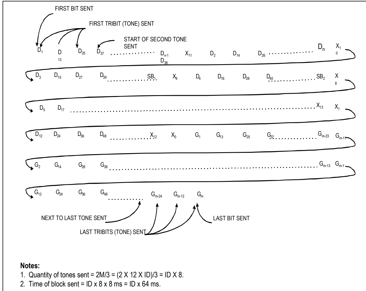
FIGURE A-51. DBM example.
