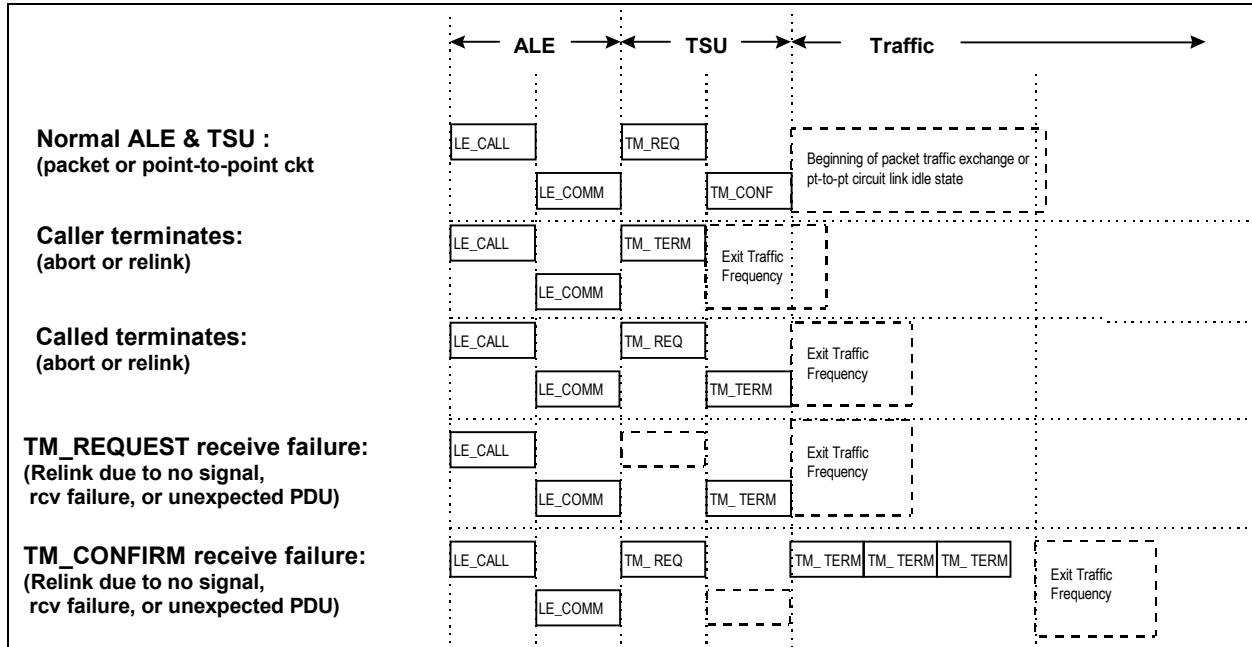
FIGURE C-40. ALE/TSU scenarios: packet and point-to-point circuit links.
