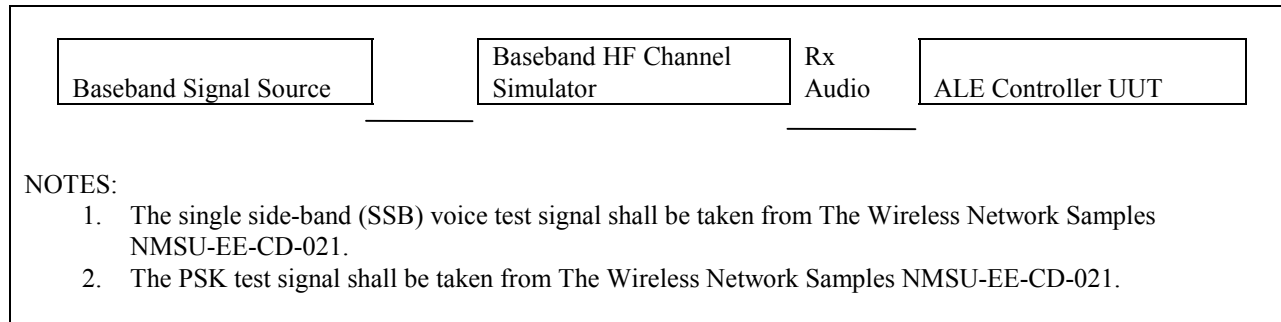
FIGURE A-2. Occupancy detection test setup.
