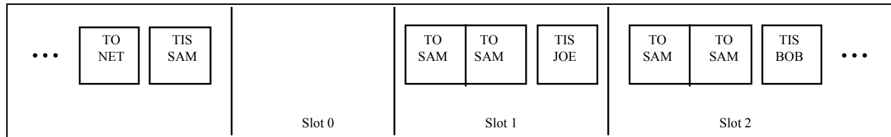
FIGURE A-32. Slotted responses.
