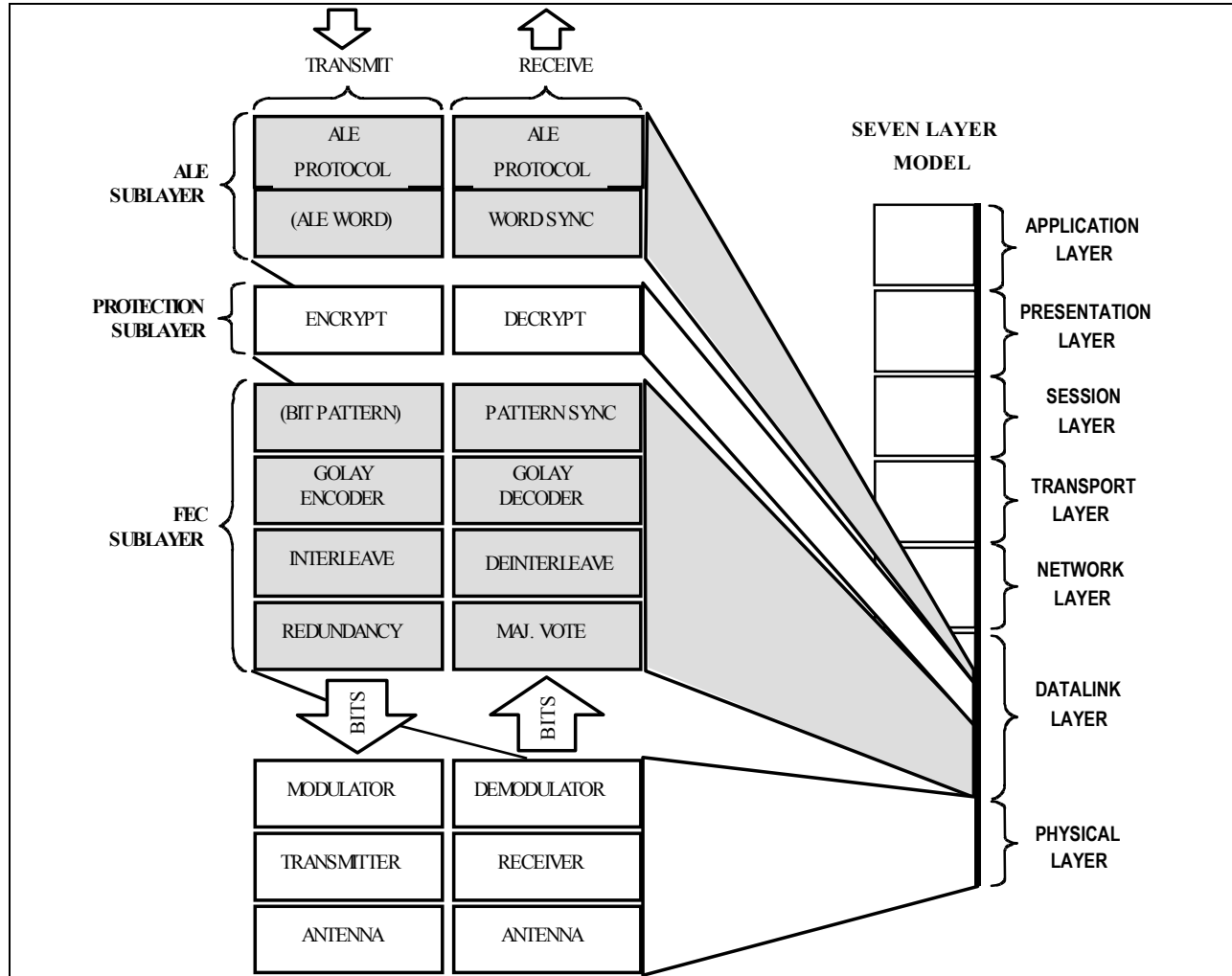
FIGURE A-1. Data link with ALE and FEC sublayers.
