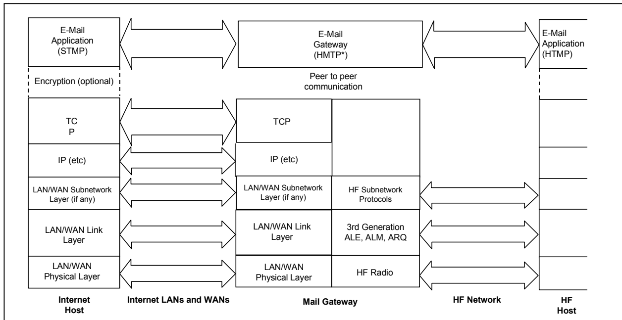
FIGURE E-3. Application-layer mail gateway.
