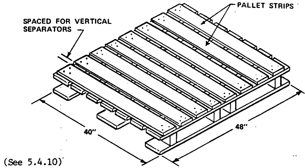
FIGURE 46. Pallet strips.
