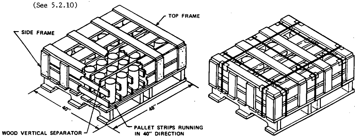
FIGURE 15. Load type X (unstrapped and strapped).
