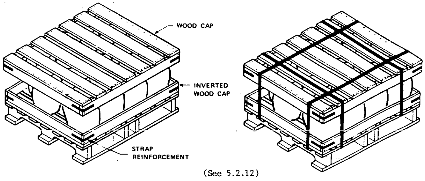
FIGURE 17. Load type XII (unstrapped and strapped).
