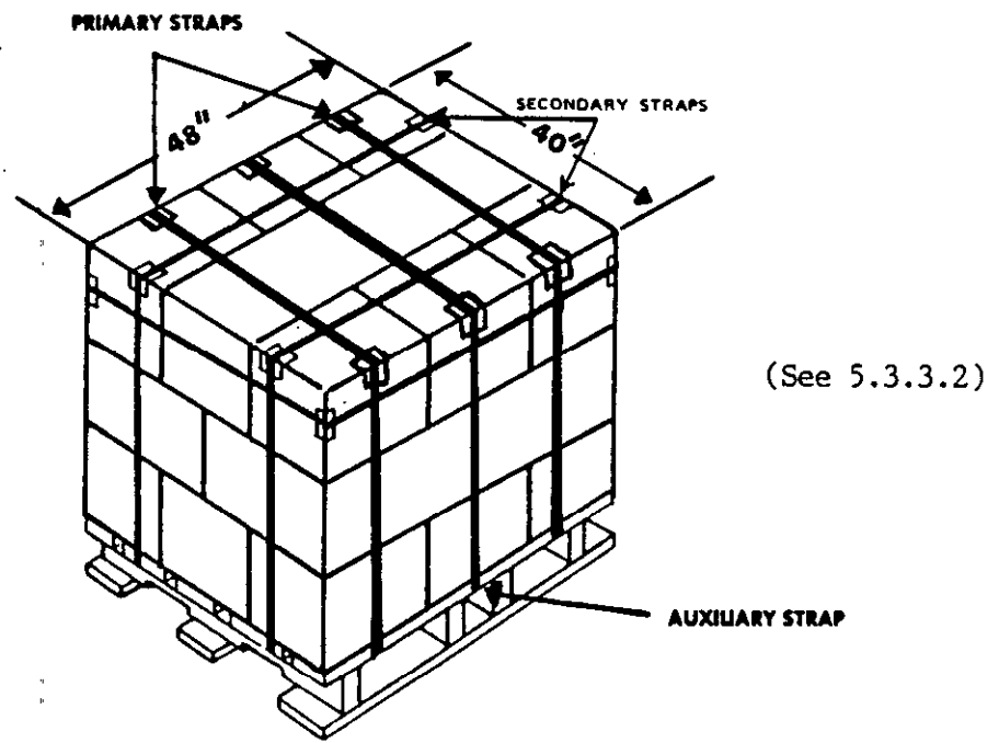
FIGURE 35. Bonding method D (tie-down straps).
