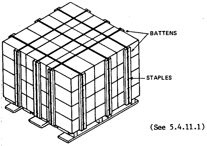
FIGURE 47. Cross-strap battens.
