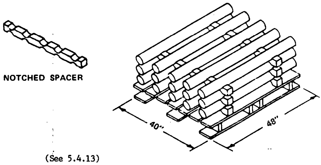
FIGURE 49. Notched spacers.
