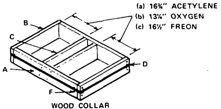
WOOD COLLAR
