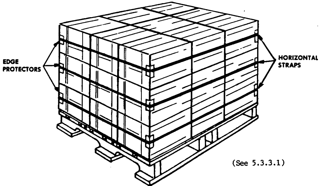
FIGURE 29. Bonding method C (each layer).
