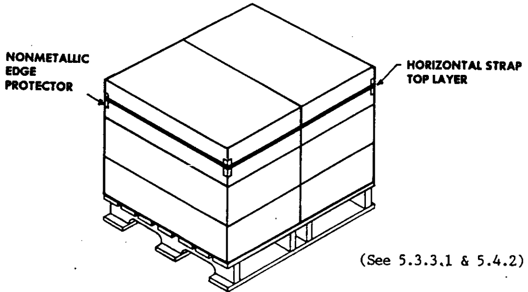
FIGURE 28. Bonding method C (top layer or single layer).
