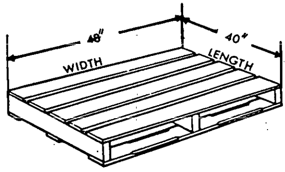
TYPE I (2-WAY ENTRY)
