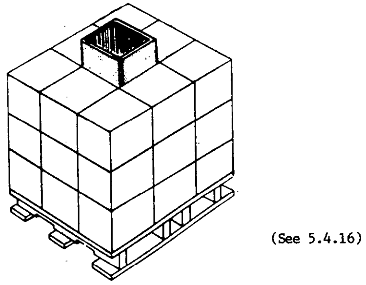
FIGURE 50. Chimney filler.
