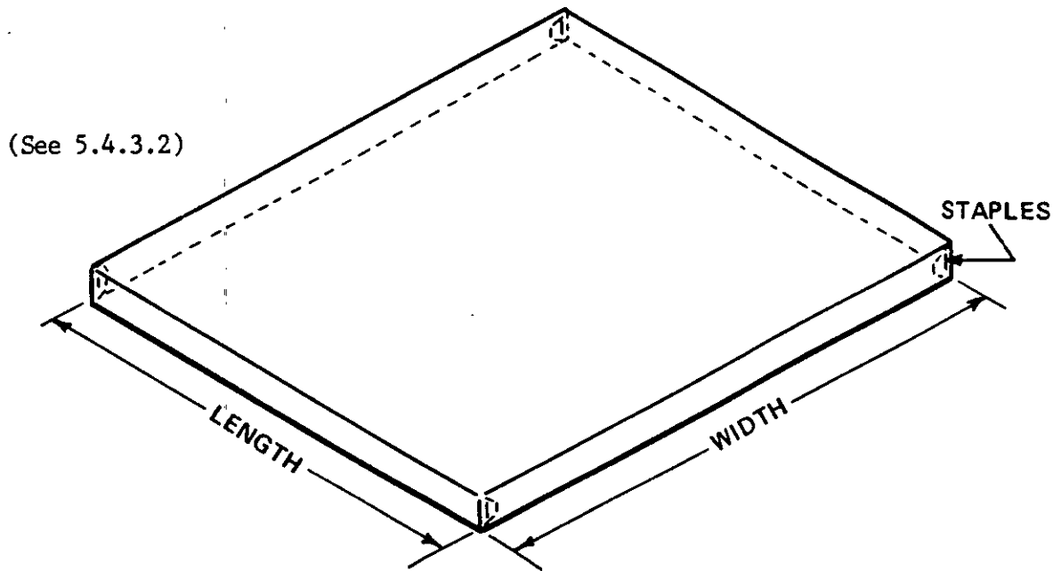
FIGURE 39. Fiberboard cap (one piece construction).
