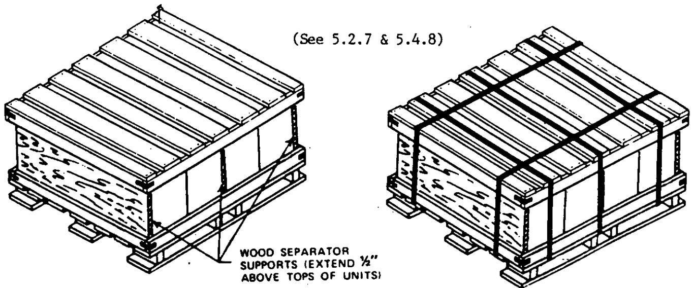
FIGURE 12. Load type VII (unstrapped and strapped).
