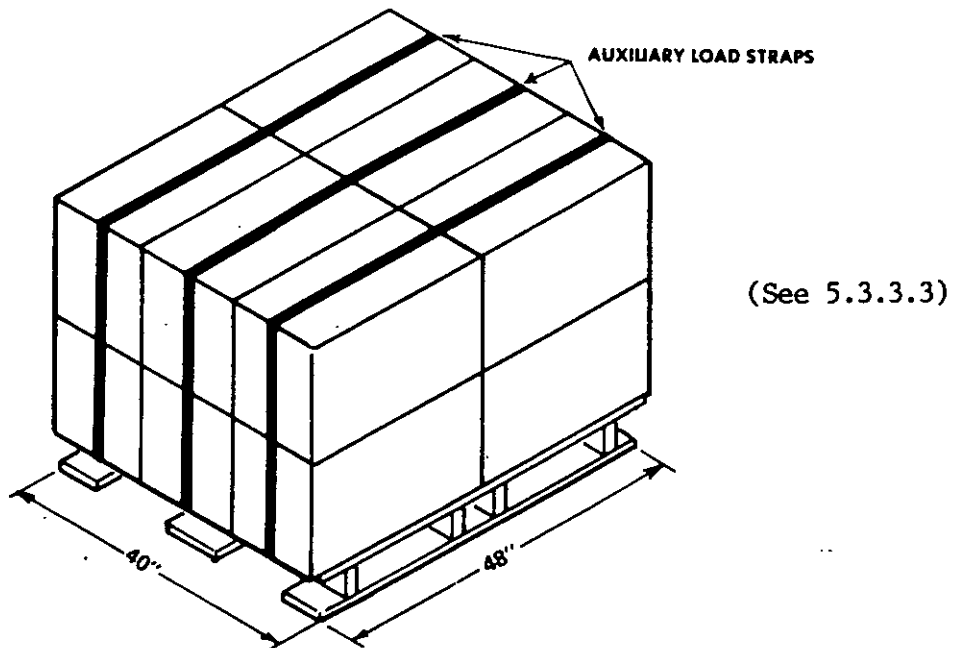
FIGURE 36. Bonding method E (auxiliary load straps).
