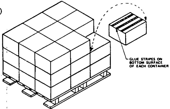
FIGURE 26. Bonding method A (glue stripes).
