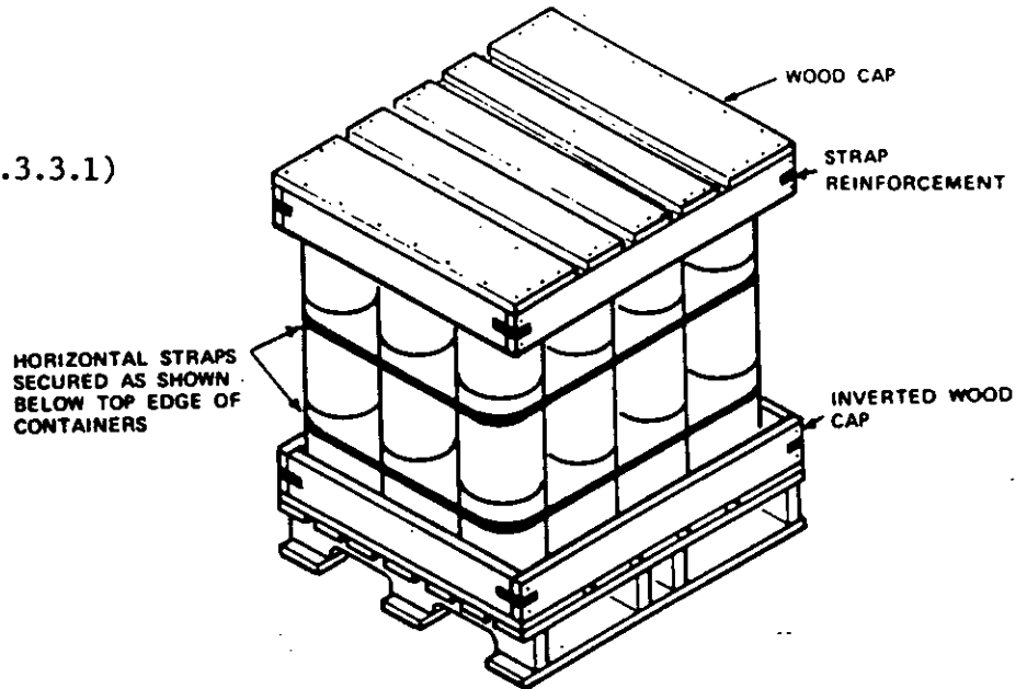
FIGURE 30. Bonding method C (each layer except top layer).
