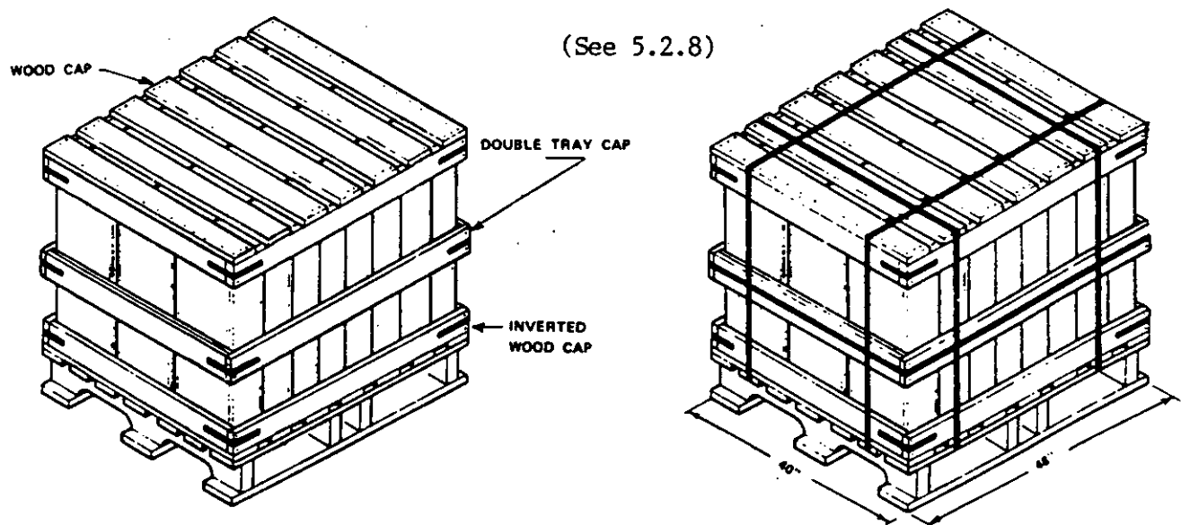
FIGURE 13. Load type VIII (unstrapped and strapped).
