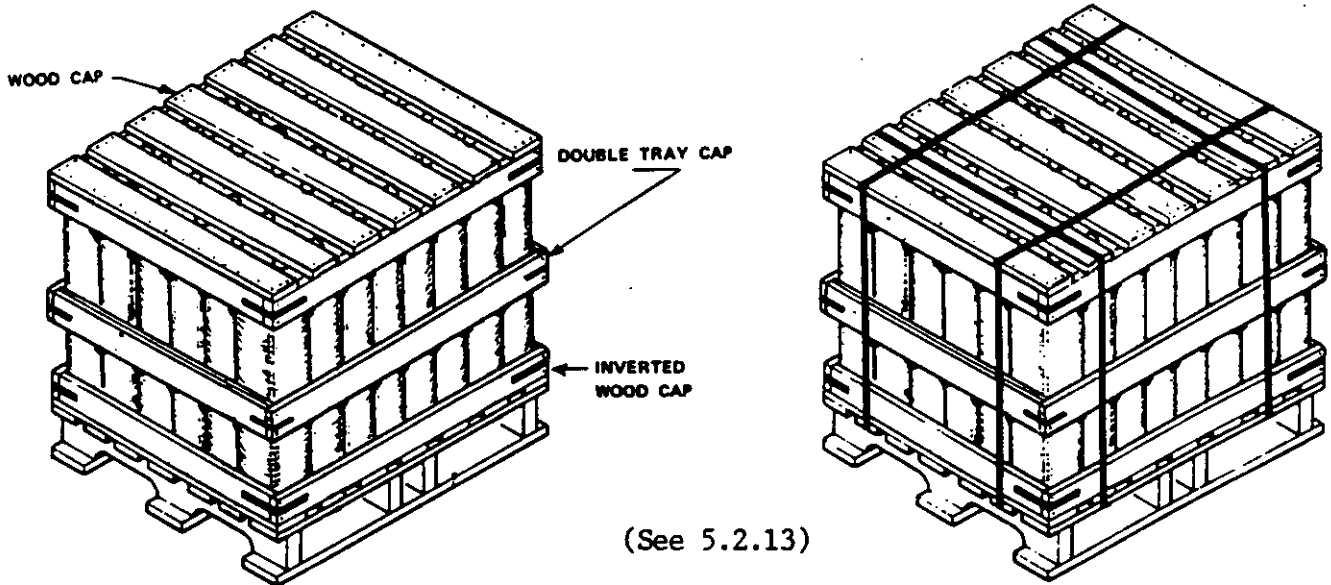
FIGURE 20. Load type XIII (unstrapped and strapped).
