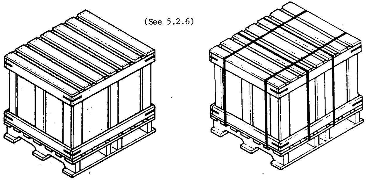
FIGURE 10. Load type V (unstrapped and strapped).
