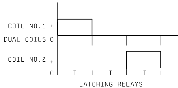
FIGURE 6. Pickup or latch / reset, hold, and dropout sequencing.
