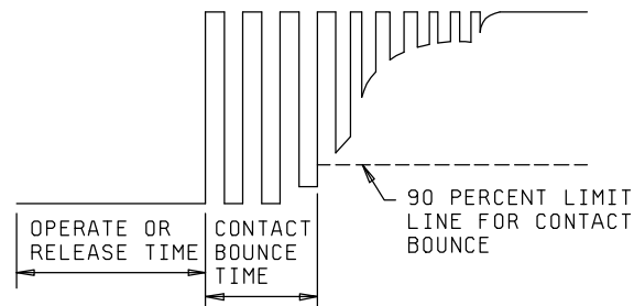
FIGURE 7. Typical circuit for operate and release time and contact bounce with typical traces.
