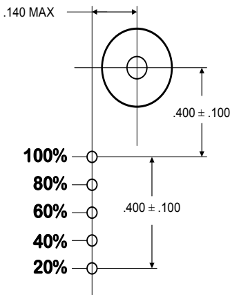
FIGURE 3. State of charge indicator dimensions FIGURE 3 NOTE: All dimensions are in inches.
