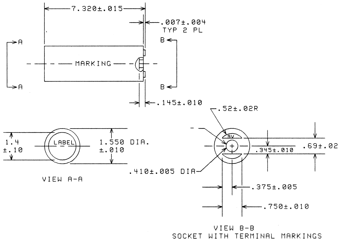
Figure 1. Battery dimensions.
