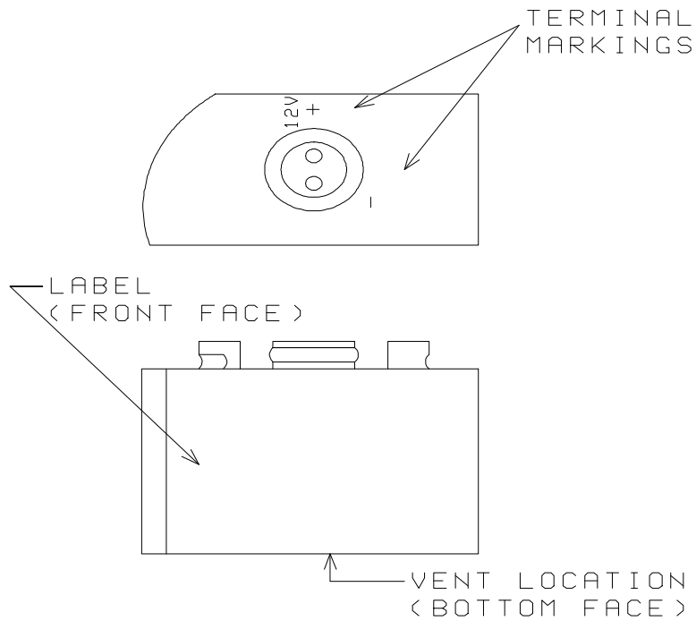
Figure 2. Terminal markings.
