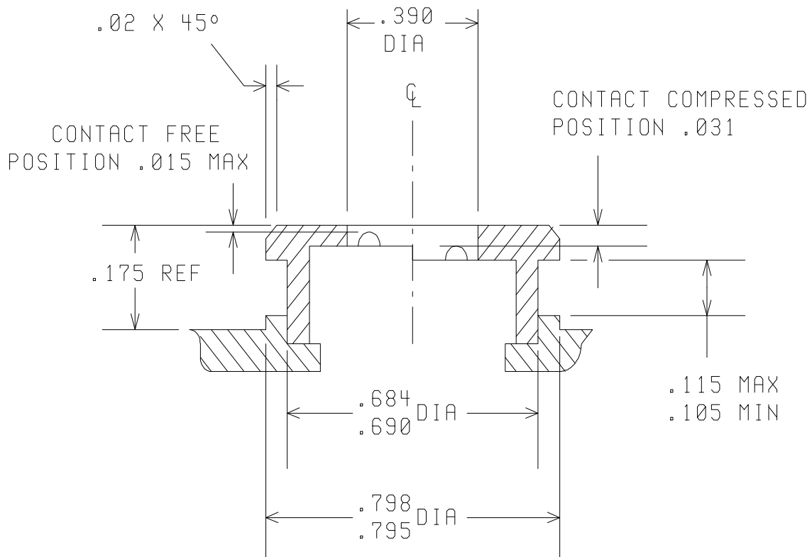
Figure 3. Contact Configuration.
