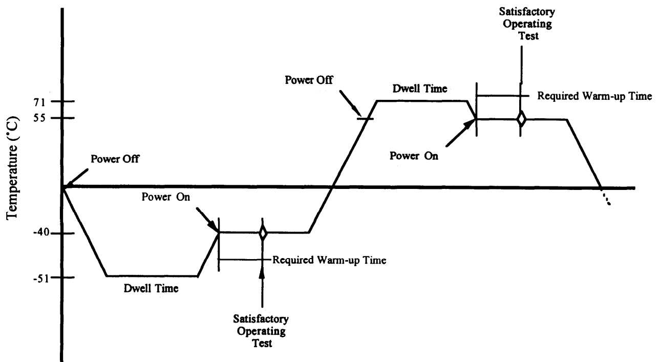
Fig. 2 —One cycle of the temperature screening curve
