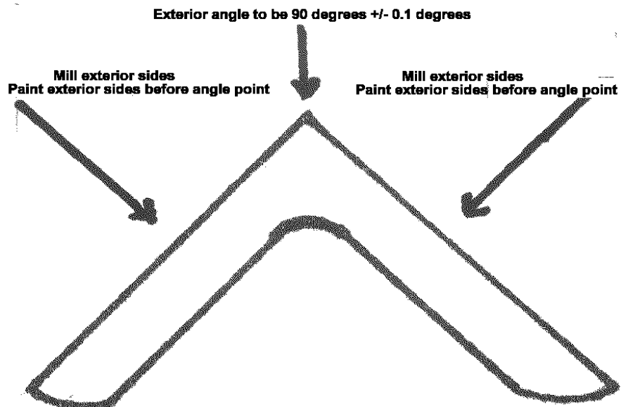
FIGURE 3. Structural angle milling and painting.
