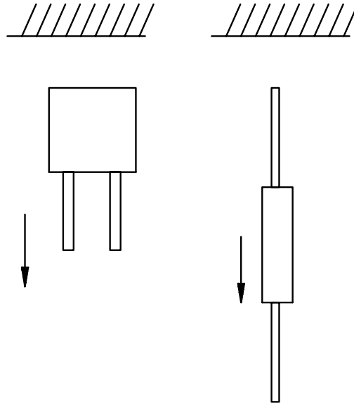
FIGURE C-1. Lead-pull direction.
