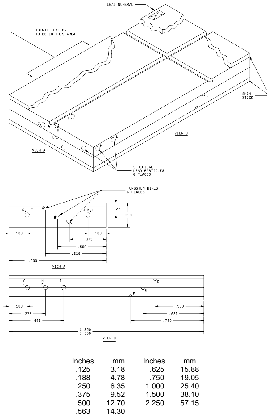
FIGURE D-1. Penetrameter.
