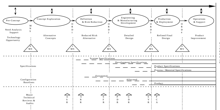
Figure 1-1: System Life Cycle
