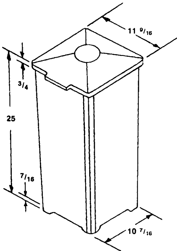
FIGURE 9. Typical refuse container.
