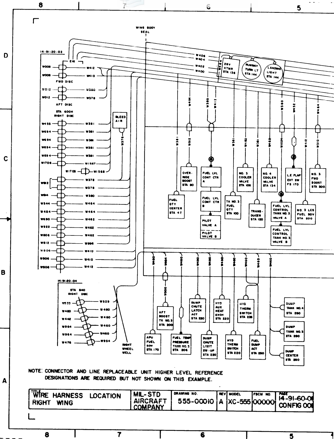
FIGURE 33. WIRE HARNESS LOCATION DIAGRAM (SHEET 1 OF 2)
