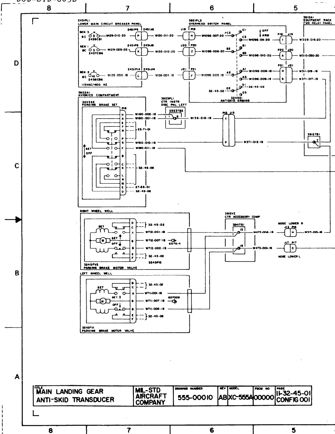
FIGURE 18. POINT TO POINT INTERCONNECT DIAGRAM (SHEET 1 OF 2)
