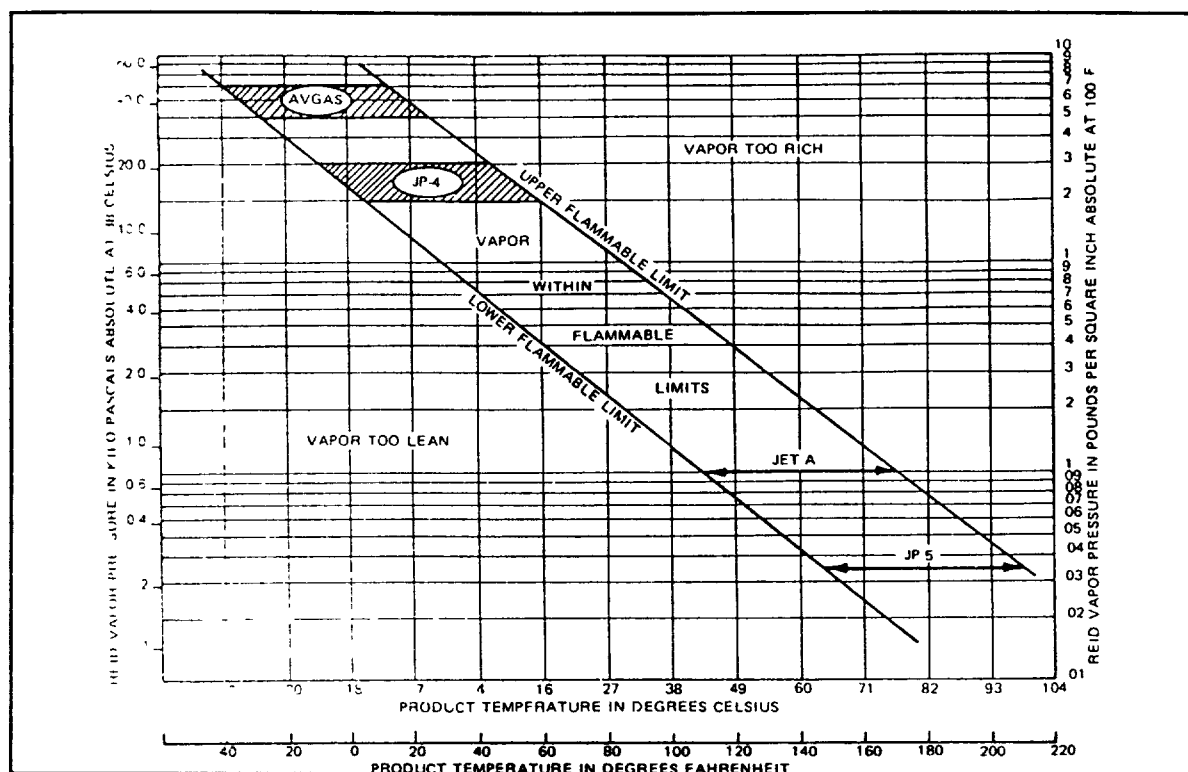
Figure 6-1. Relationship Between Temperature, Rvp, and Flammable Limits of Petroleum Products at Seat Level
