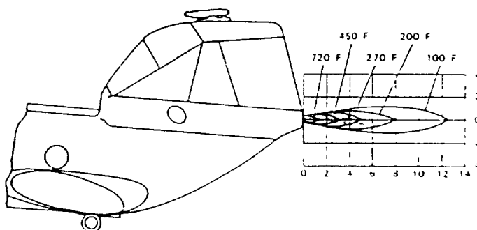
APU EXHAUST WAKE PROFILE – FEET
