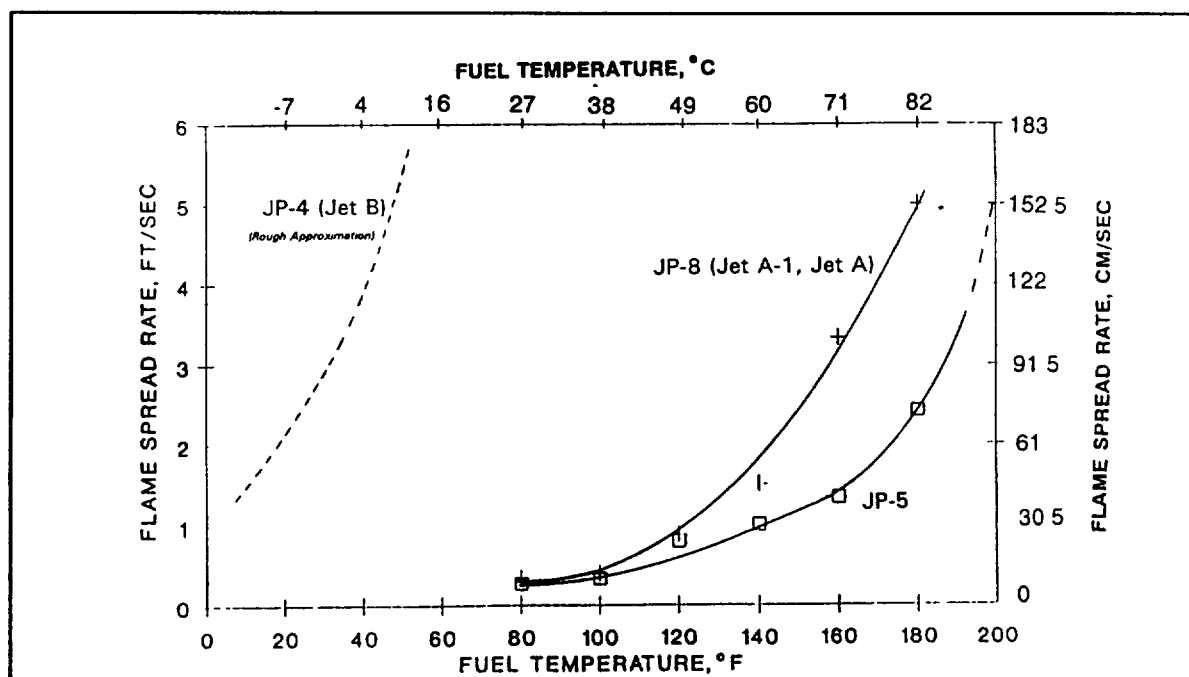
Figure 6-2. Flame Spread Rate Versus Fuel Temperature.
