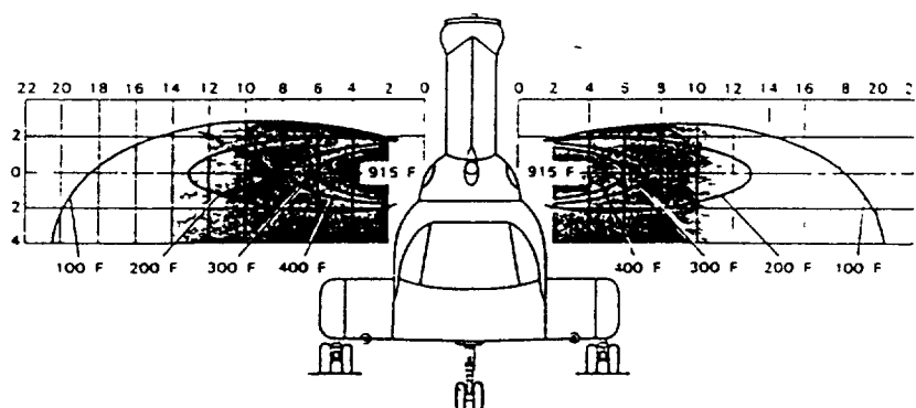
ENGINE EXHAUSE WAKE PROFILE – FEET
