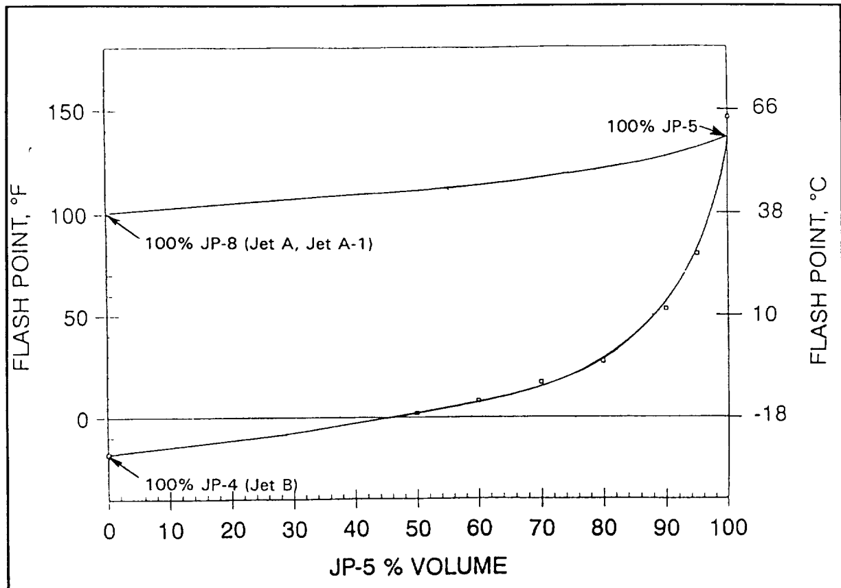
Figure 6-3. Flash Point of Turbine Fuel Mixtures.
