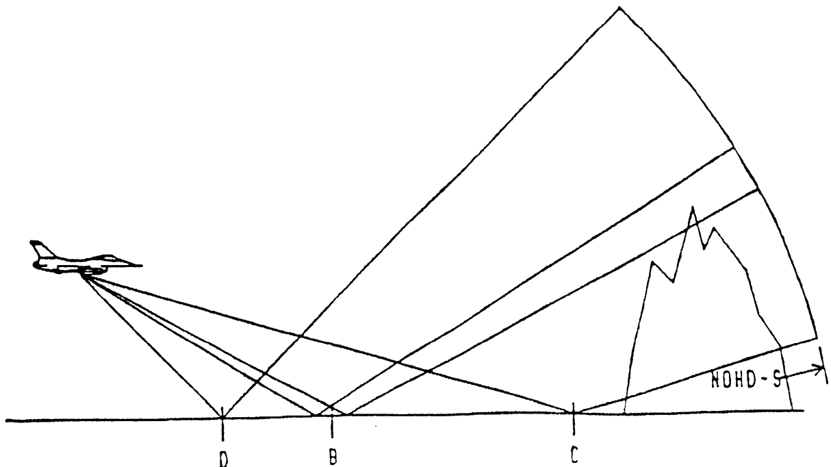
Figure E-12. Reflections from still water within LSDZ
