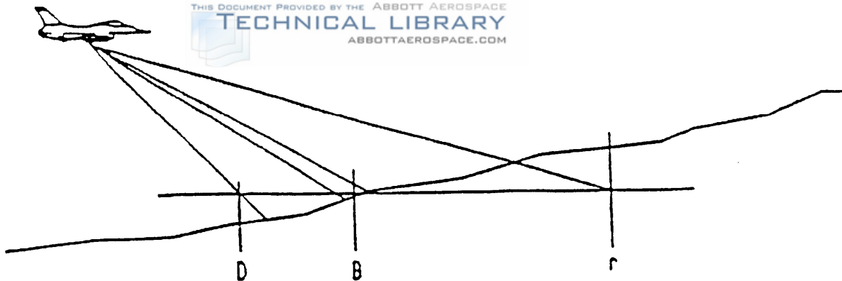
Figure E-7. LSDZ with rising terrain
