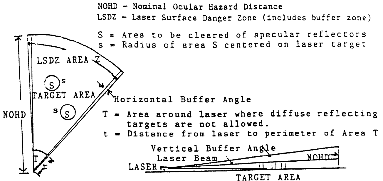
LSDZ FROM GROUND FIRED LASER - WITHOUT NATURAL BACKSTOP
