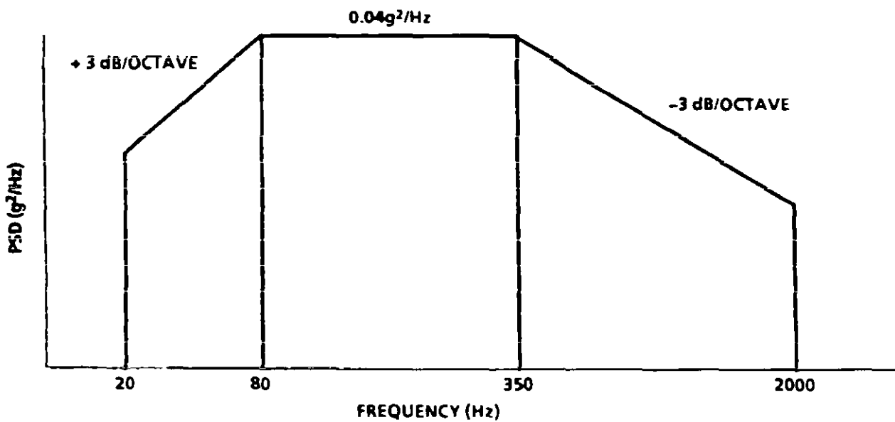
FIGURE 5. Vibration stress.
