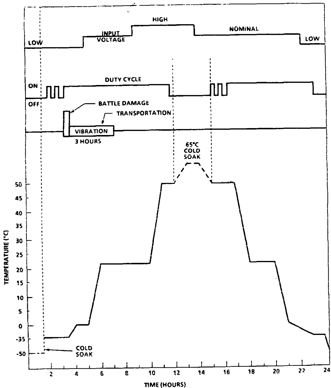
FIGURE 55. Submarine profile .
