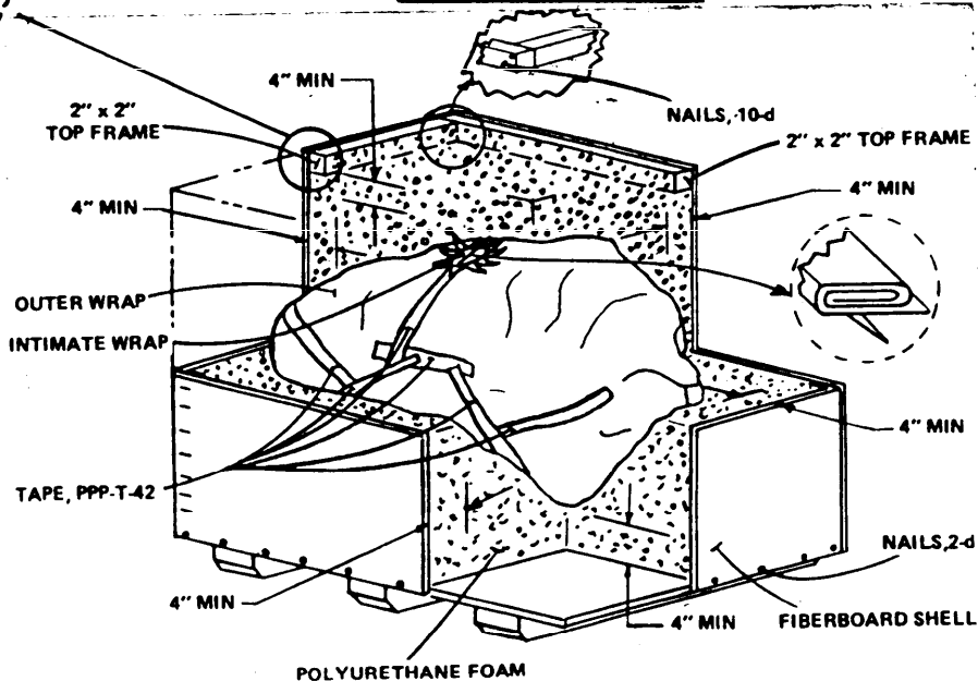
FIGURE 12. Encapsulated pack (design 4).
