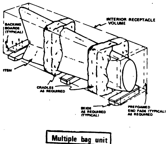
FIGURE 7. Foam-in-bag.
