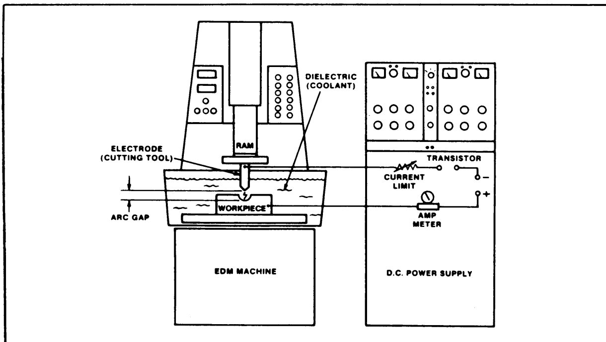
Figure A-5. Electrical Discharge Machining (Elox Division/Colt Industries)
