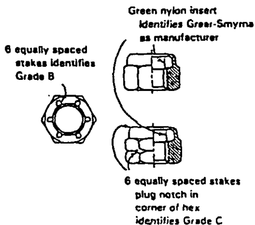
NYLON INSERT
