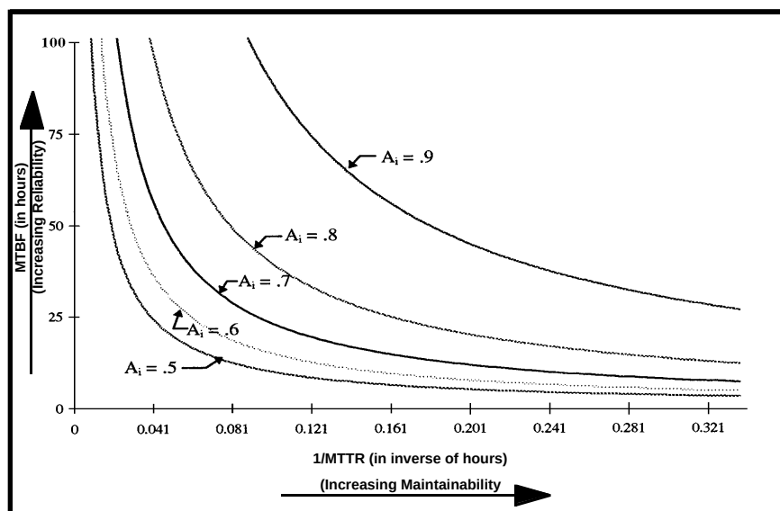
FIGURE 1. Different Combinations of MTBF and MTTR Yield the Same Inherent Availability.
