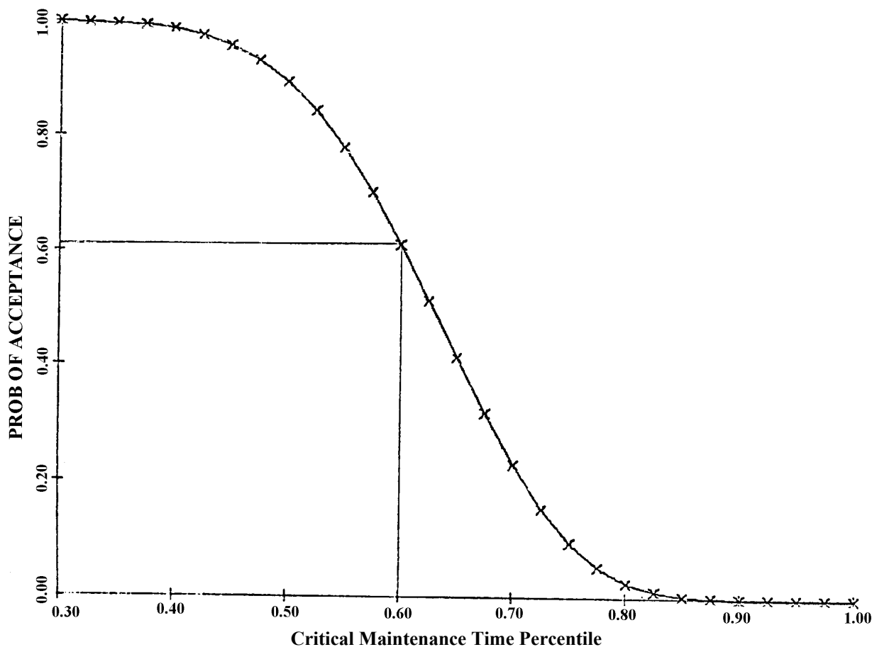
FIGURE B-6: OC Curve for Test Method 3.
