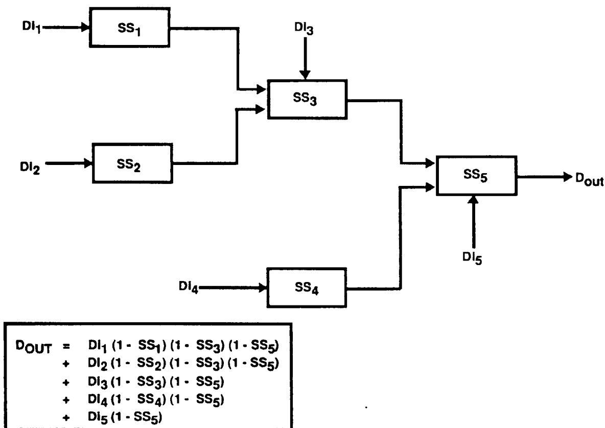
Figure 5.1: Sample Multi Level ESS Flow Diagram
