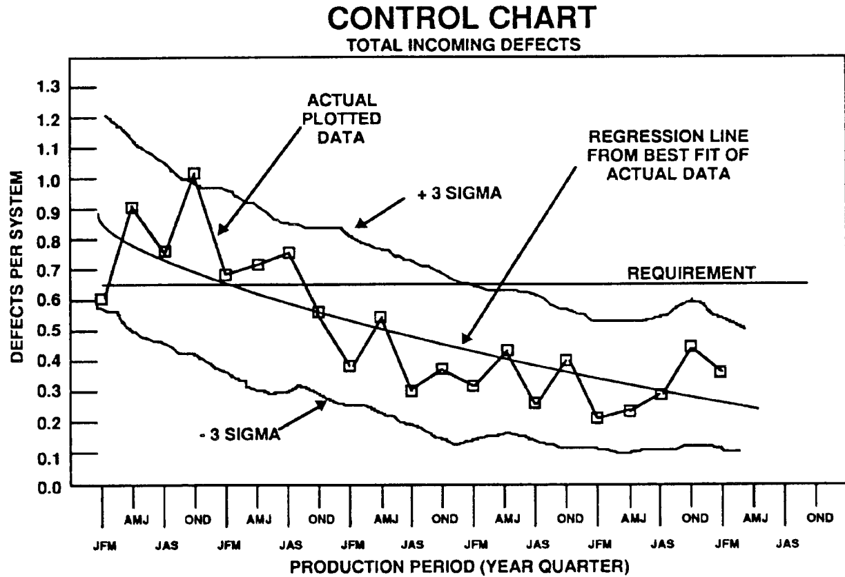
Figure 5-13: Sample SPC Chart
