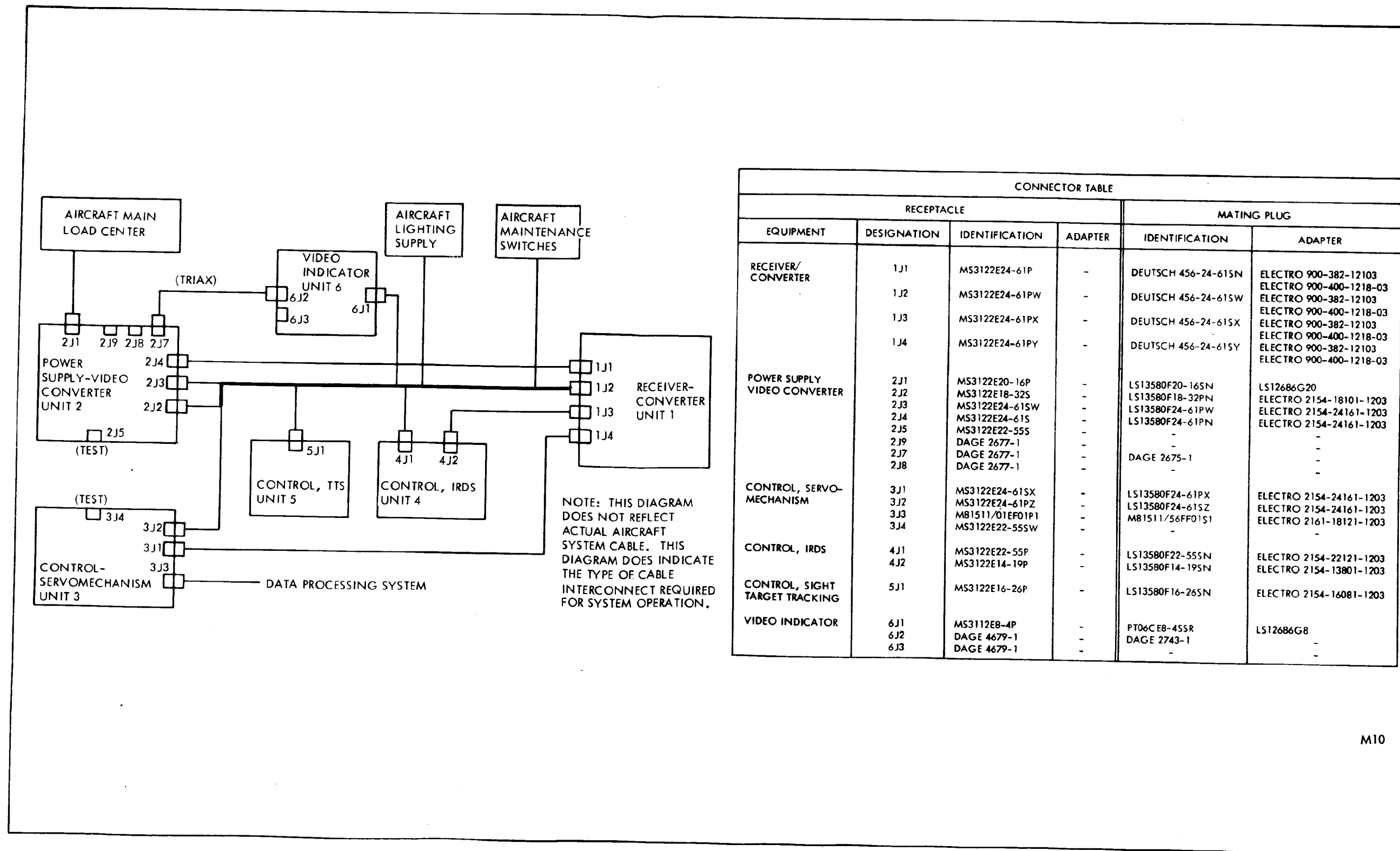
FIGURE 10. IRDS interconnecting block diagram.
