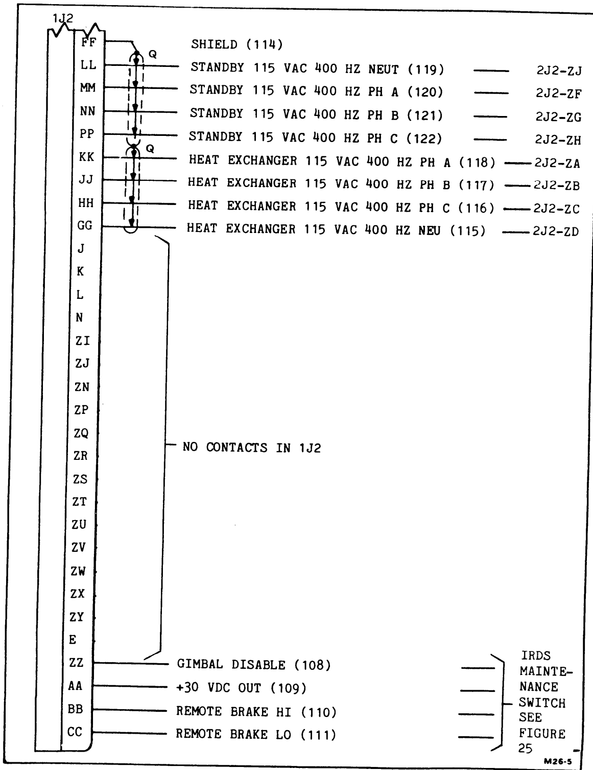
FIGURE 26. IRDS interconnecting diagram. (sheet 5 of 27)
