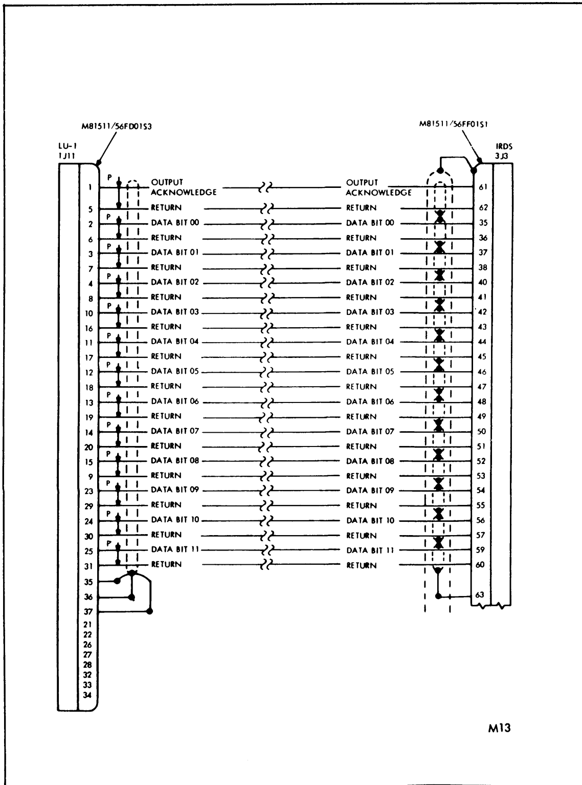
FIGURE 13. LU-1 DOM/IRDS CONTROL SERVOMECHANISM INTERFACE (P-3C).
