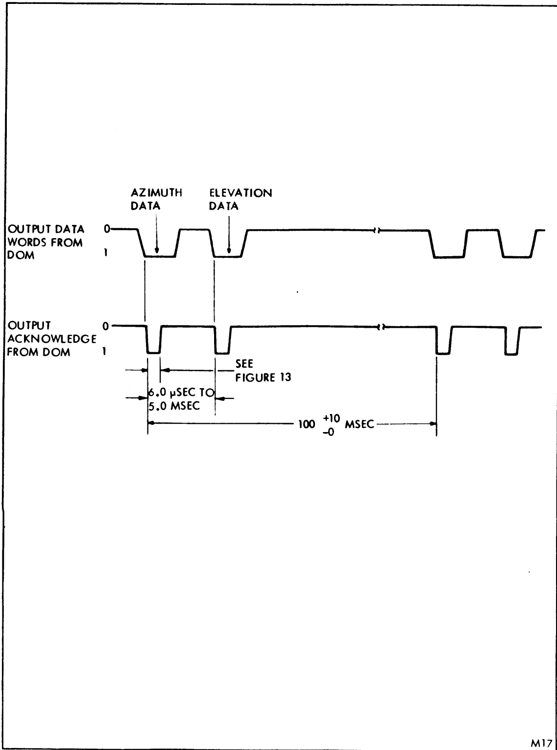
FIGURE 17. DOM/IRDS data update timing requirements.
