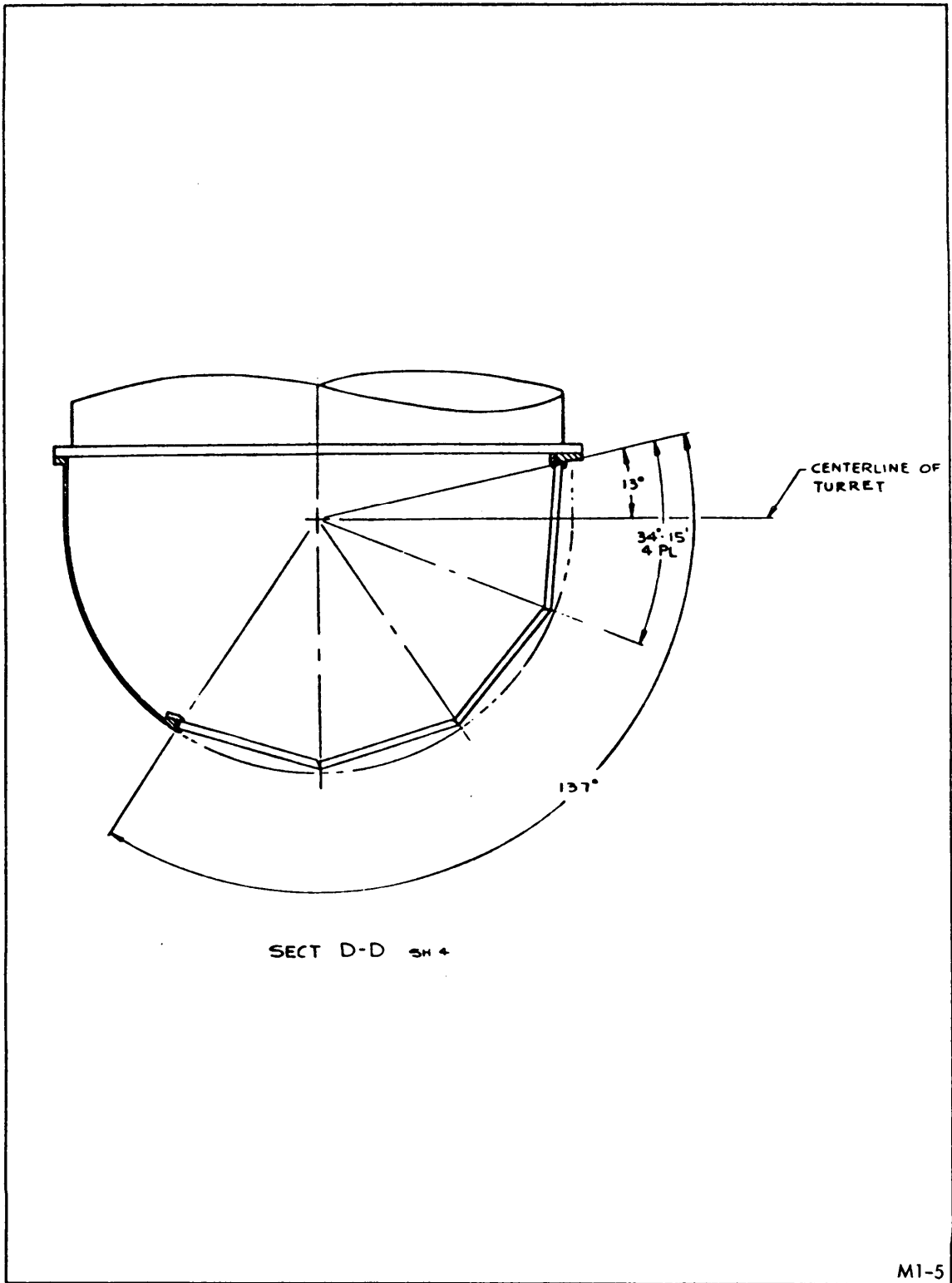
FIGURE 1. Receiver converter, outline drawing. (sheet 5 of 5)
