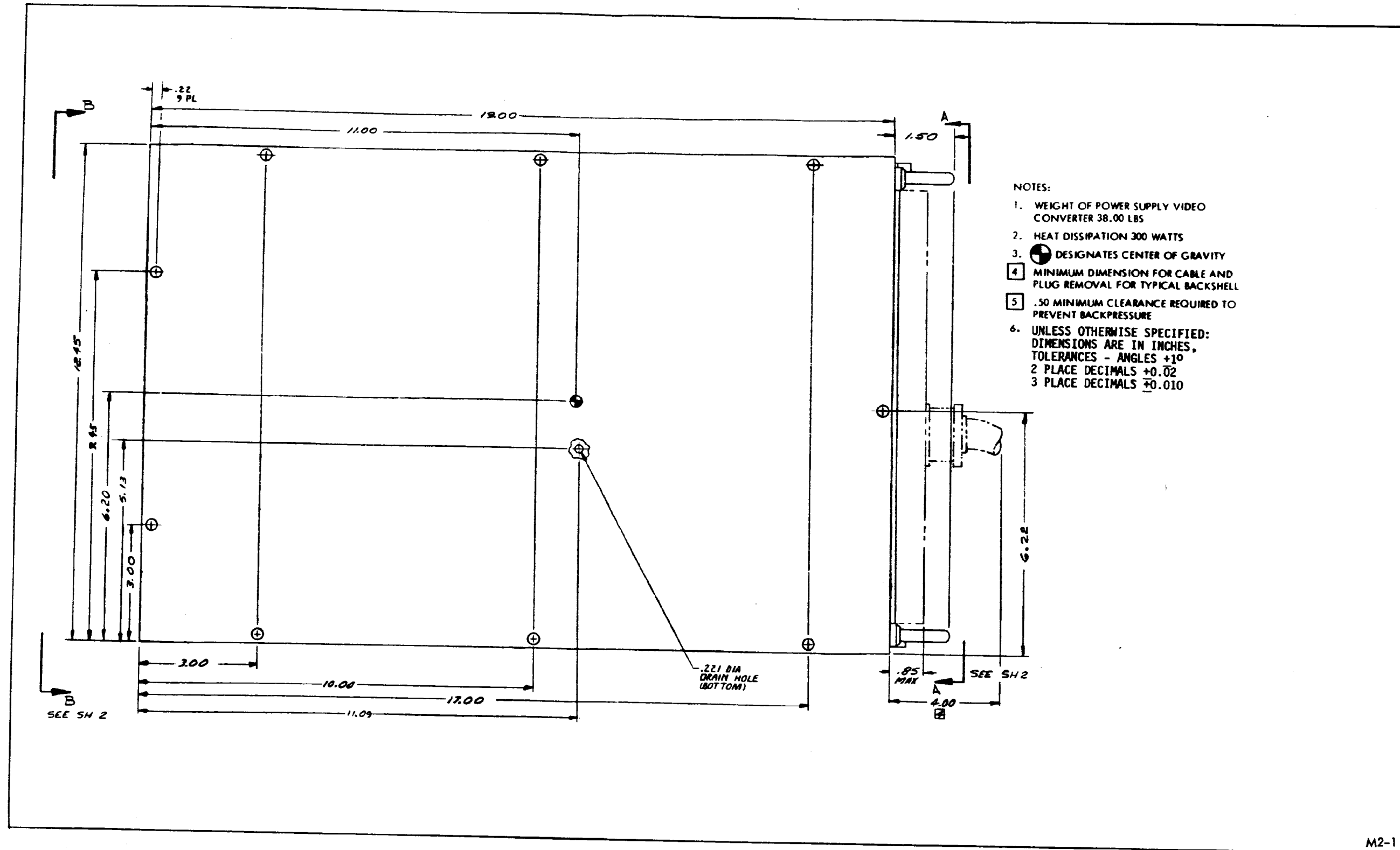
FIGURE 2. Power supply/video converter, outline drawing. (sheet 1 of 2)
