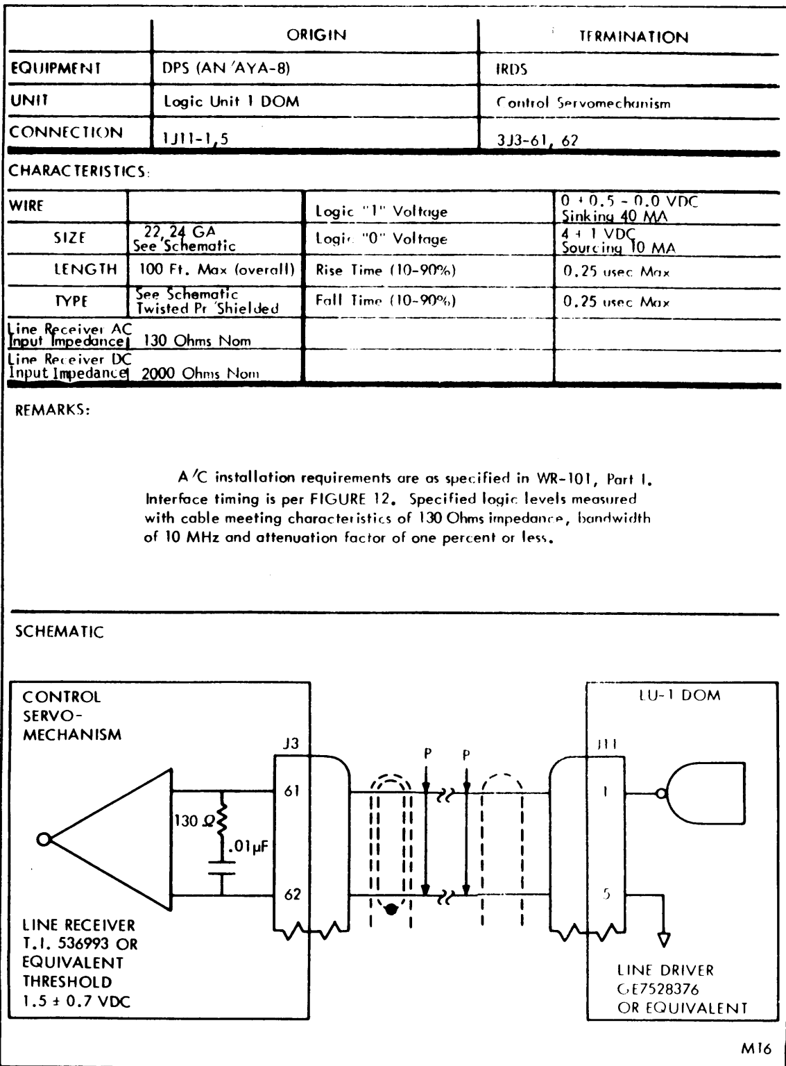
FIGURE 16. Output acknowledge signal characteristics.
