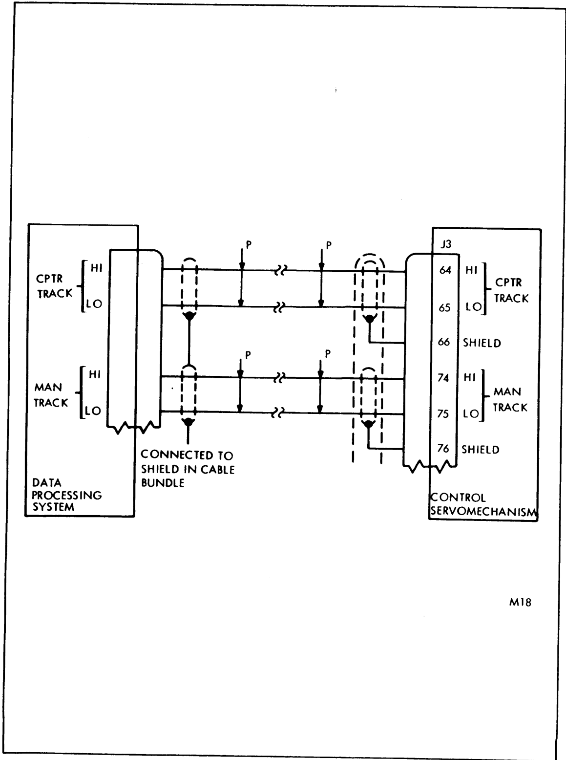
FIGURE 18. IRDS/data processing system status logic interface (P-3C).
