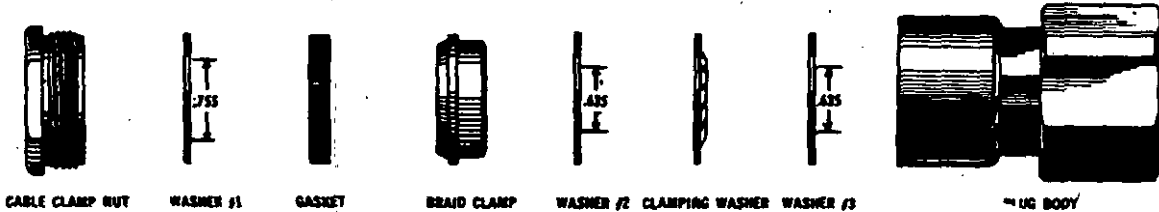
CABLE CLAMP NUT WASHER #1 GASKET BRAID CLAMP WASHER #2 CLAMPING WASHER WASHER #3 PLUG BODY
