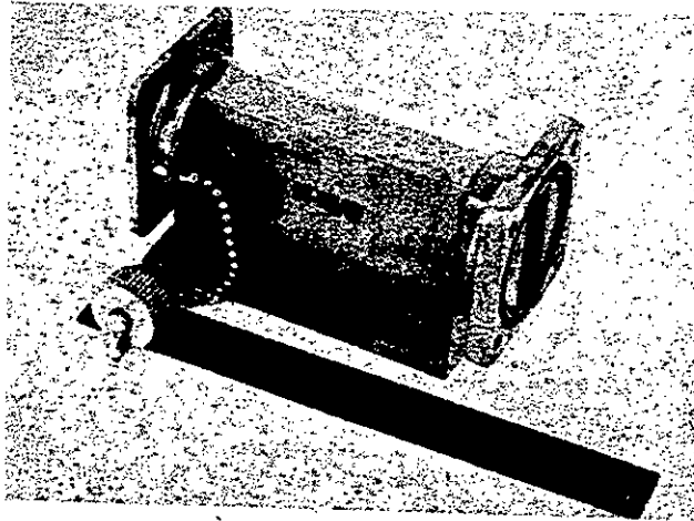
TYPICAL UNIDIRECTIONAL COUPLER
