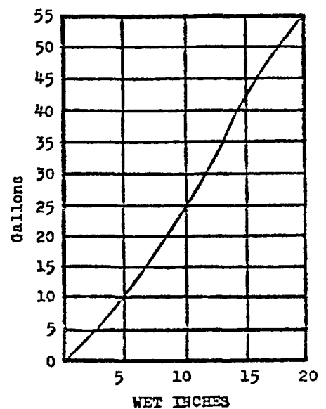
HORIZONTAL DRUM
