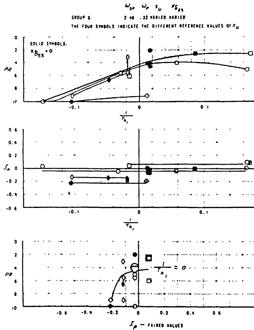
FIGURE 125. Landing approach (T-33, AFFDL-TR-66-2).
