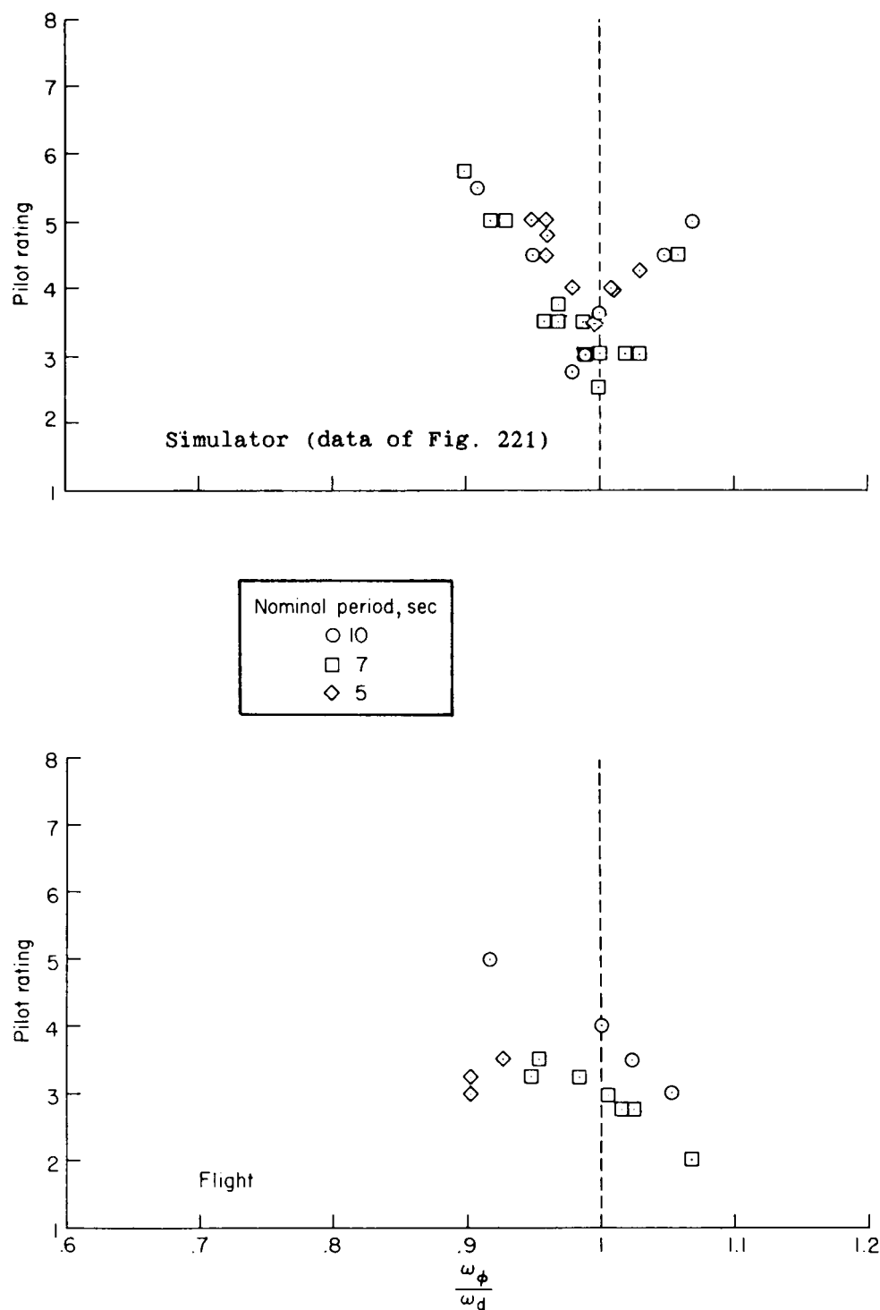
FIGURE 222. Variation of pilot rating with \omega_{\psi}/\omega_d for moving-base simulator and flight data \zeta_d \approx 0.15 (NASA-TN-D-3910).
