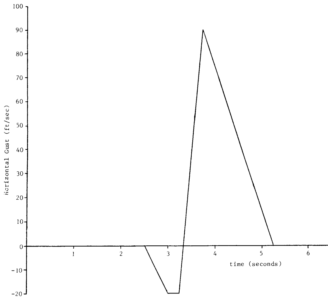
FIGURE 264. Earth-axis winds.
