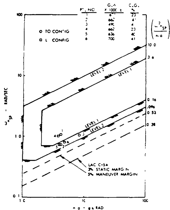
a) C-5A Category C flight data.
