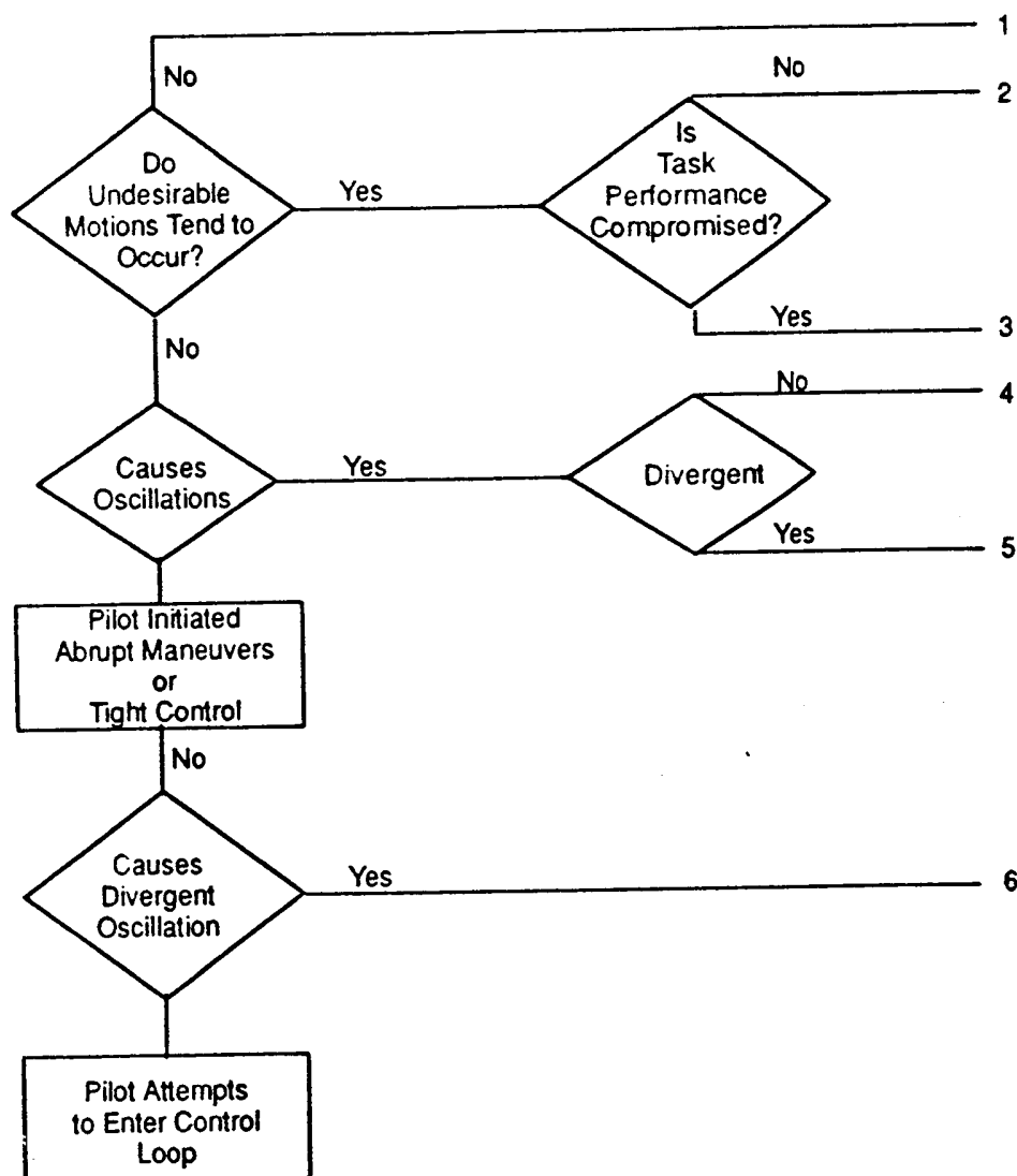
FIGURE 12. PIO tendency classification from AFWAL-TR-81-3118.
