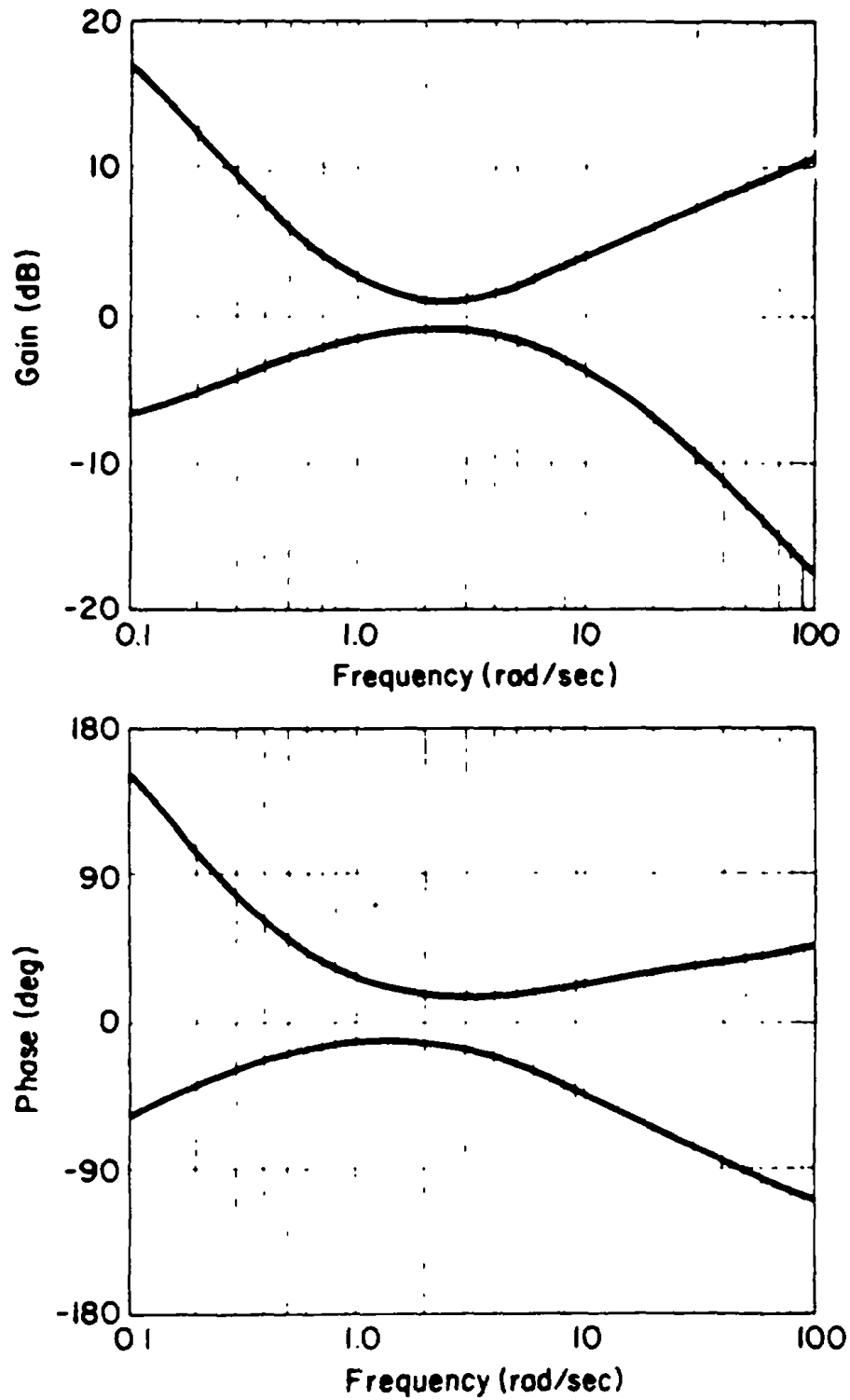
FIGURE 15. Envelopes of maximum unnoticeable added dynamics (AFWAL-TR-82-3064).
