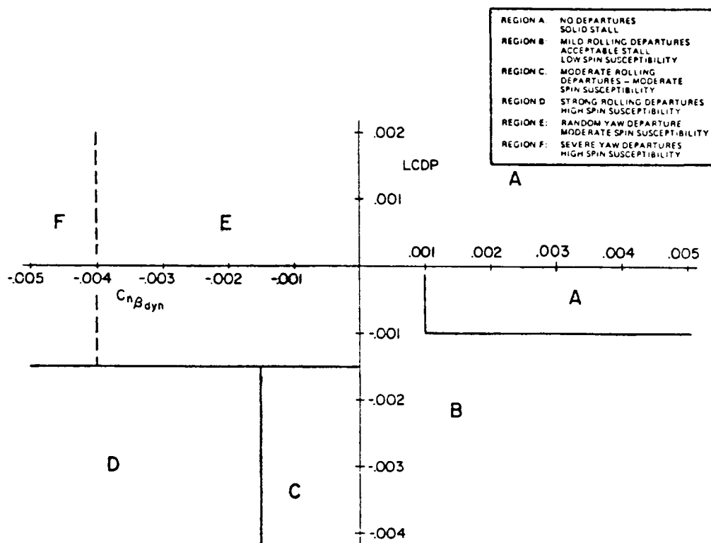
FIGURE 259. Departure and spin susceptibility criterion suggested by ASD-TR-72-48 and AFWAL-TR-80-3141.
