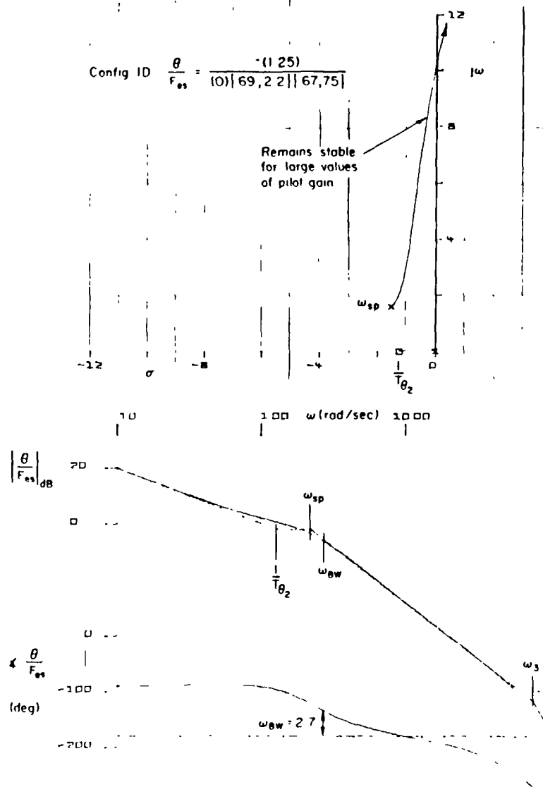
FIGURE 61a. Level 1/2 system of Neal-Smith (1D): \omega_{BW} = 2.7 rad/sec, mean PR = 4.1.
