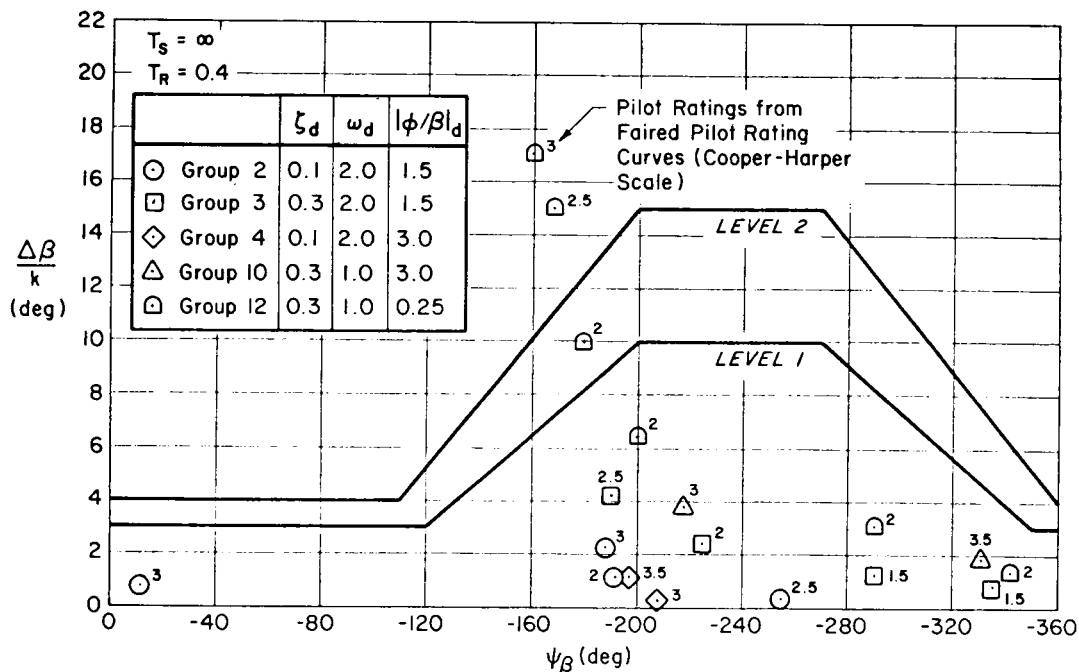
FIGURE 242. \Delta\beta_{\max}/k versus \psi_\beta for configurations that meet Level 1 p_{\text{osc}}/p_{\text{av}} , \zeta_d , and \zeta_d\omega_d criteria (from AFFDL-TR-70-145).
