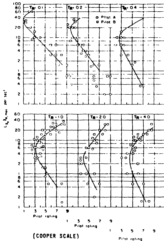
FIGURE 138. Variation of pilot opinion with L_{\delta_a} \delta_{a, \text{max}} for constant values of T_R as obtained from the stationary flight simulator (from NASA Memo 1-29-59A).
