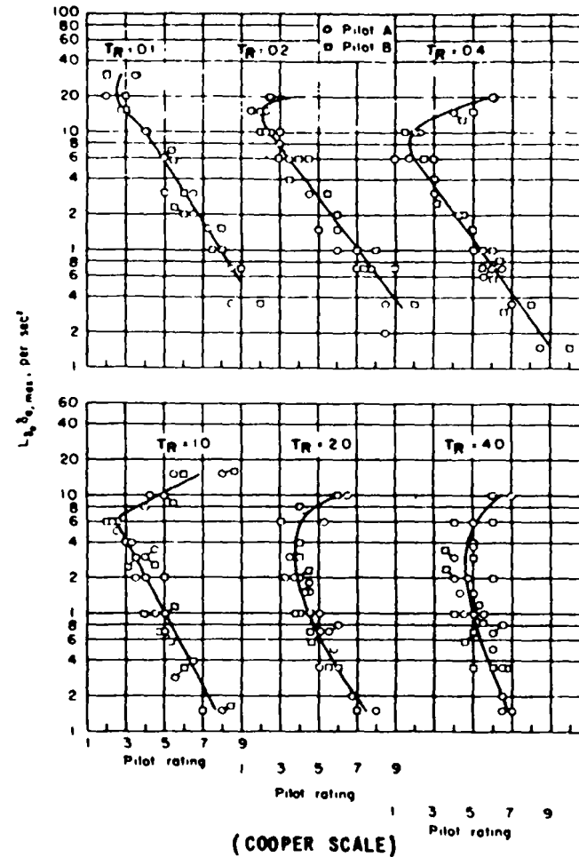
FIGURE 139. Variation of pilot opinion with L_{\delta_a} \delta_{a, \text{max}} for constant values of T_R as obtained from the moving flight simulator (from NASA Memo 1-29-59A).
