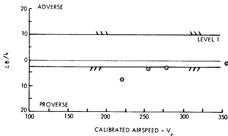
FIGURE 244. Sideslip excursion data for Class III aircraft in Category B Flight Phases (from AFFDL-TR-78-171)
