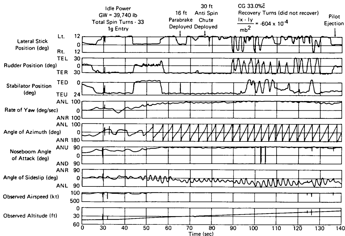
FIGURE 261. Left flat spin, F-4B (from AFFDL-TR-70-155).
