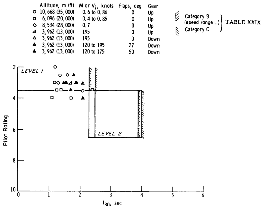
FIGURE 176. Time to bank, 300 for CV-990 (NASA-TN-D-681 1).
