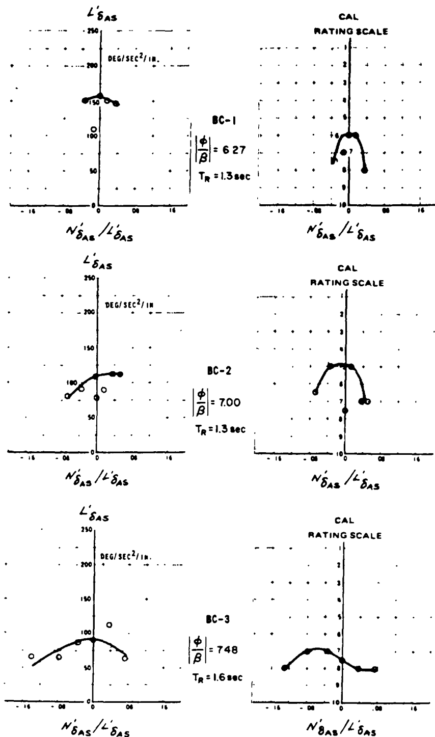
FIGURE 137. Pilot ratings and optimum aileron sensitivity (Medium |\phi/\beta|_d , Long T_R ) (from AFFDL-TR-67-98).
