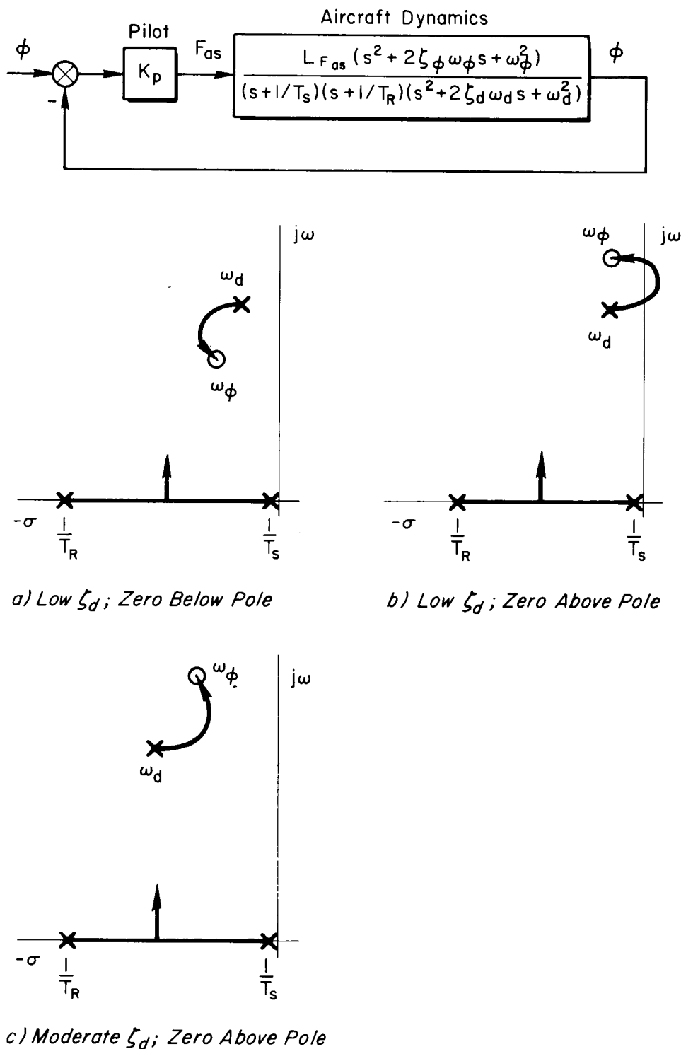
FIGURE 158. Effect of relative pole/zero location on piloted control of bank angle.
