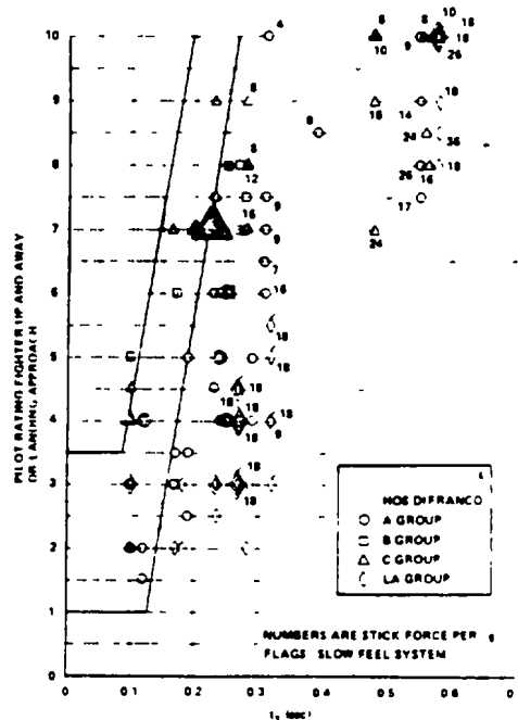
FIGURE 55. Pilot rating correlation with effective time delay (AFFDL-TR-68-90 data).
