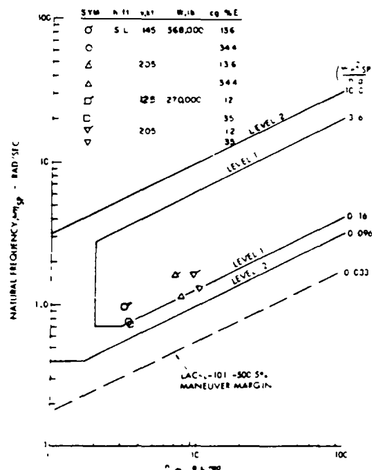
d) L-1011 landing configuration.
