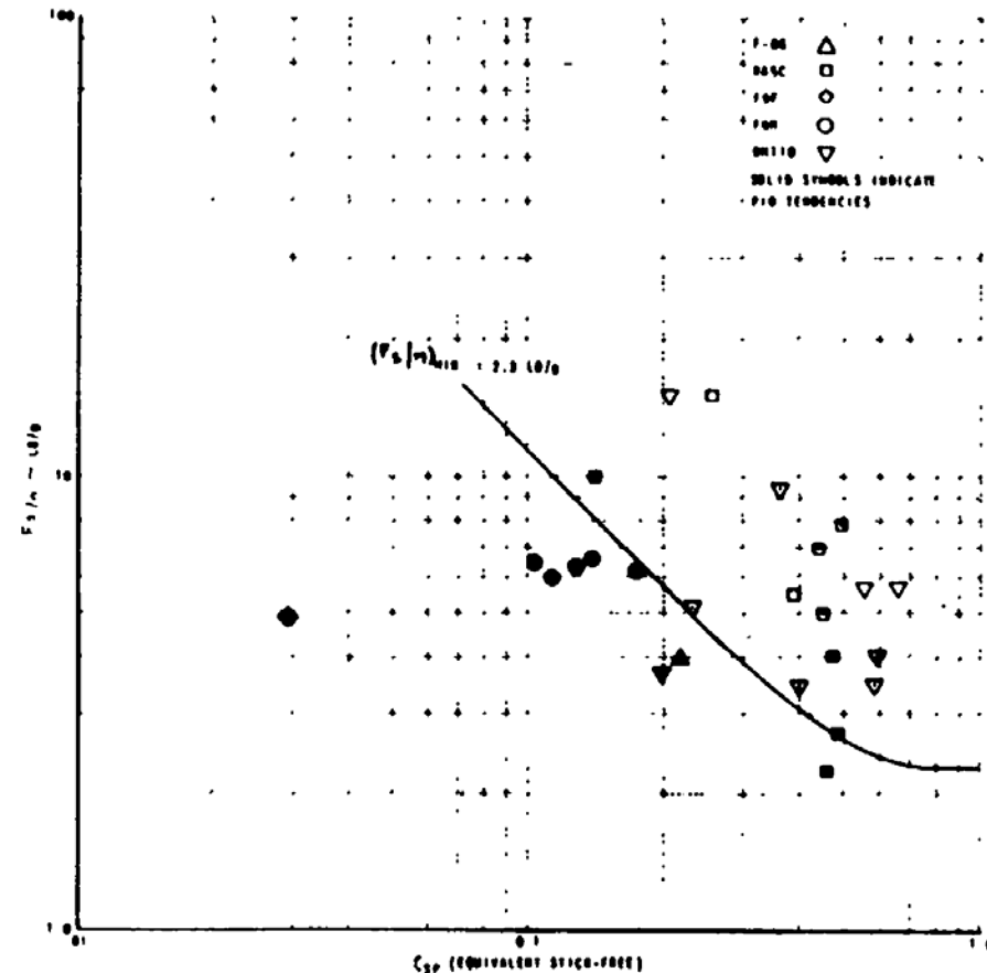
FIGURE 120. PIO characteristics of airplanes described in AGARD-CP-17.
