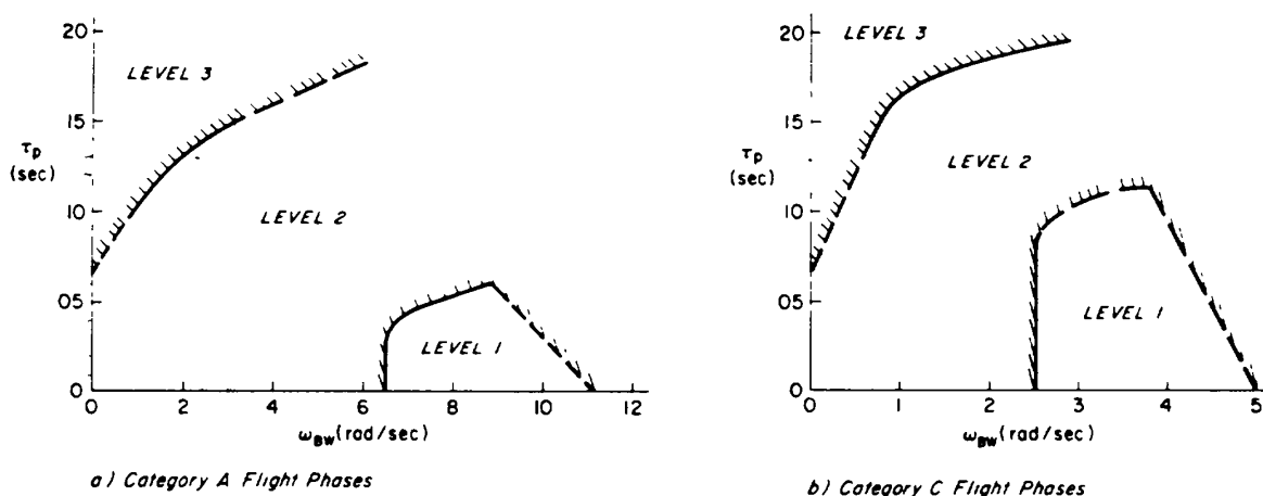
FIGURE 57. Bandwidth requirements.
