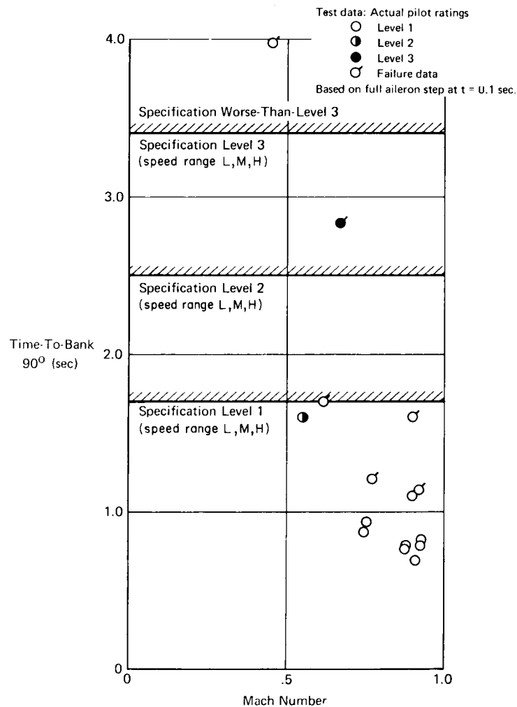
FIGURE 177. F-4 roll control effectiveness, time-to-bank 90°, CR configuration (from AFFFDL-TR-70-155).
