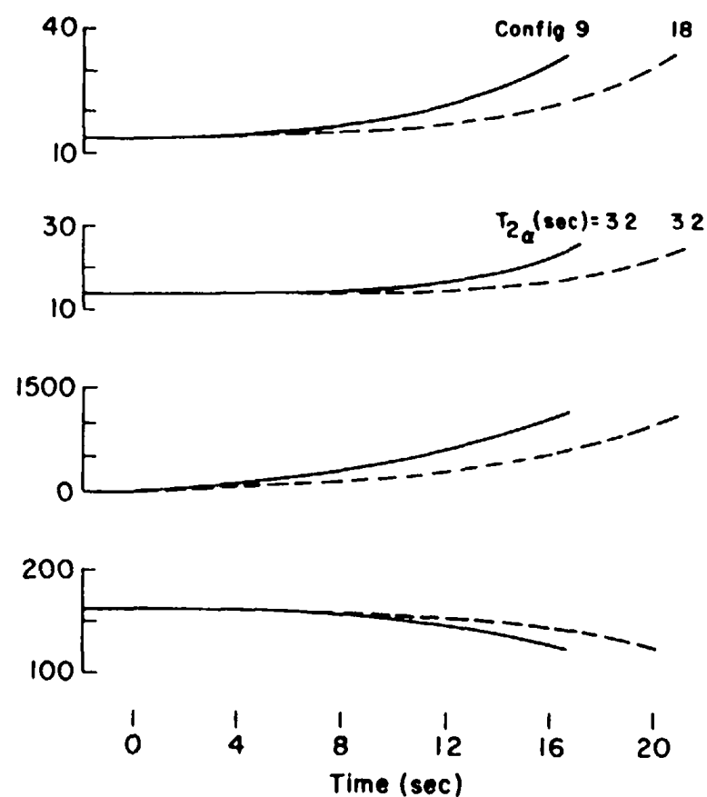
b) Effect of Increased Pitch Damping with Same T_2 . ( C_{mq} + C_{m\dot{\alpha}} ) for Config 18 was 5 Times That of Config. 9
