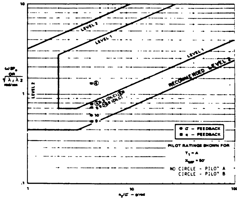
c) Short aft tail, x_{mp} = 50 ft
