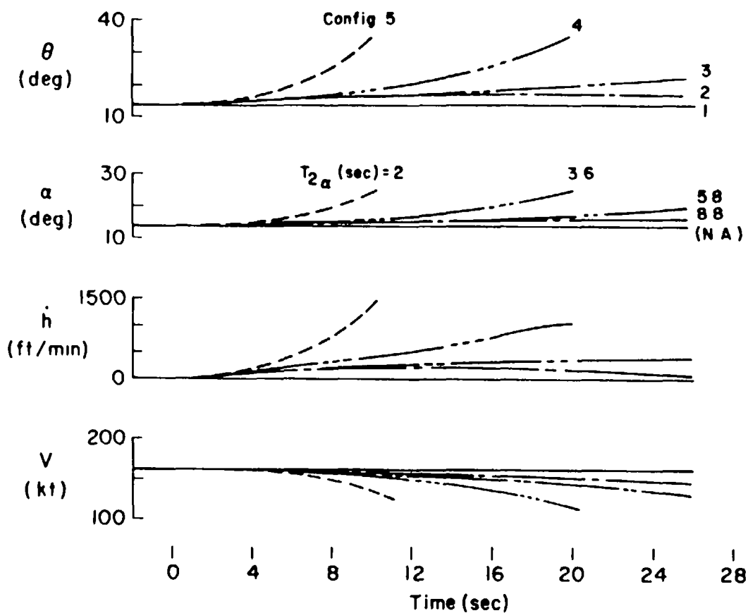
a) Comparison of Linear C_m(\alpha) Configurations 1-5
