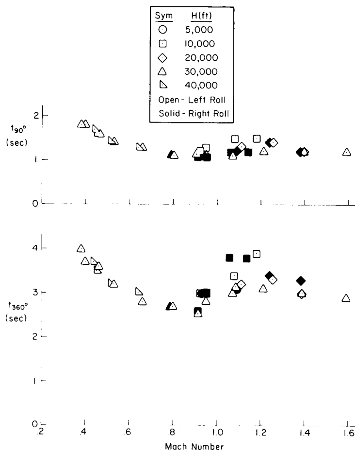
FIGURE 186. YF-16 rolling performance in cruise configuration; AFFTC-TR-75-15.
