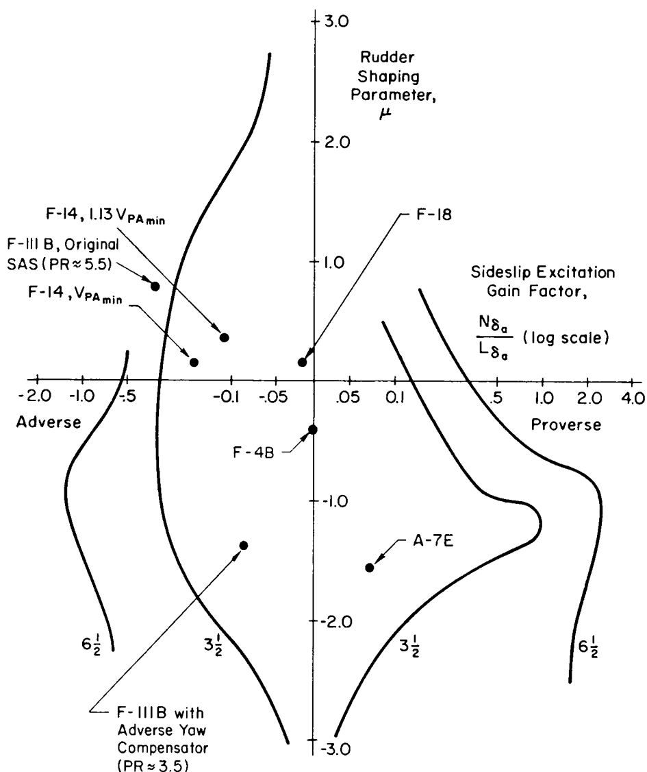
FIGURE 254. Required aileron-rudder sequencing for several operational aircraft, SAS/CAS ON (from Systems Technology, Inc., TR-1090-1).
