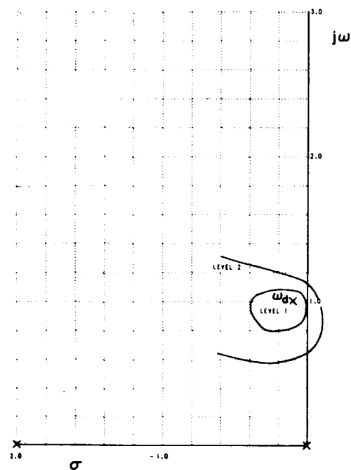
c) \omega_d = 1.0 \text{ rad/sec} ; \zeta_d = 0.1
