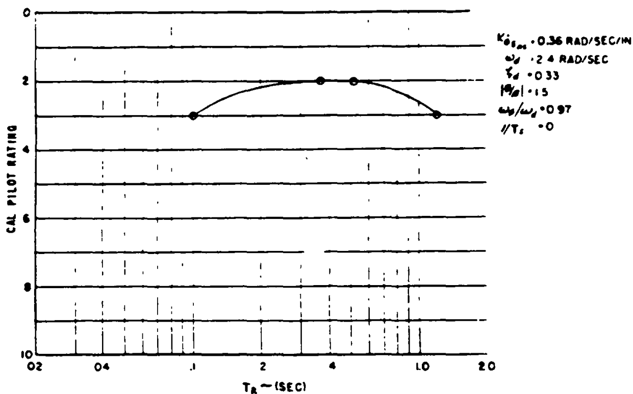
FIGURE 143. Pilot rating versus roll mode time constant (from WADD-TR-61-147).
