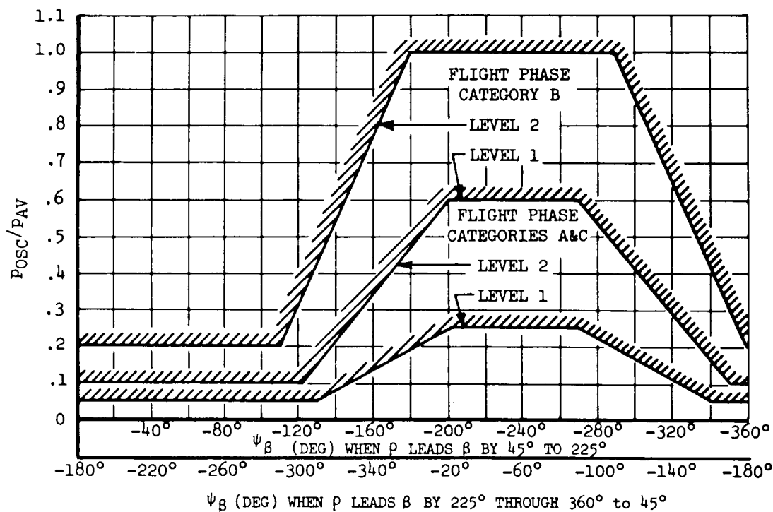
FIGURE 156. Roll rate oscillation limitations.
