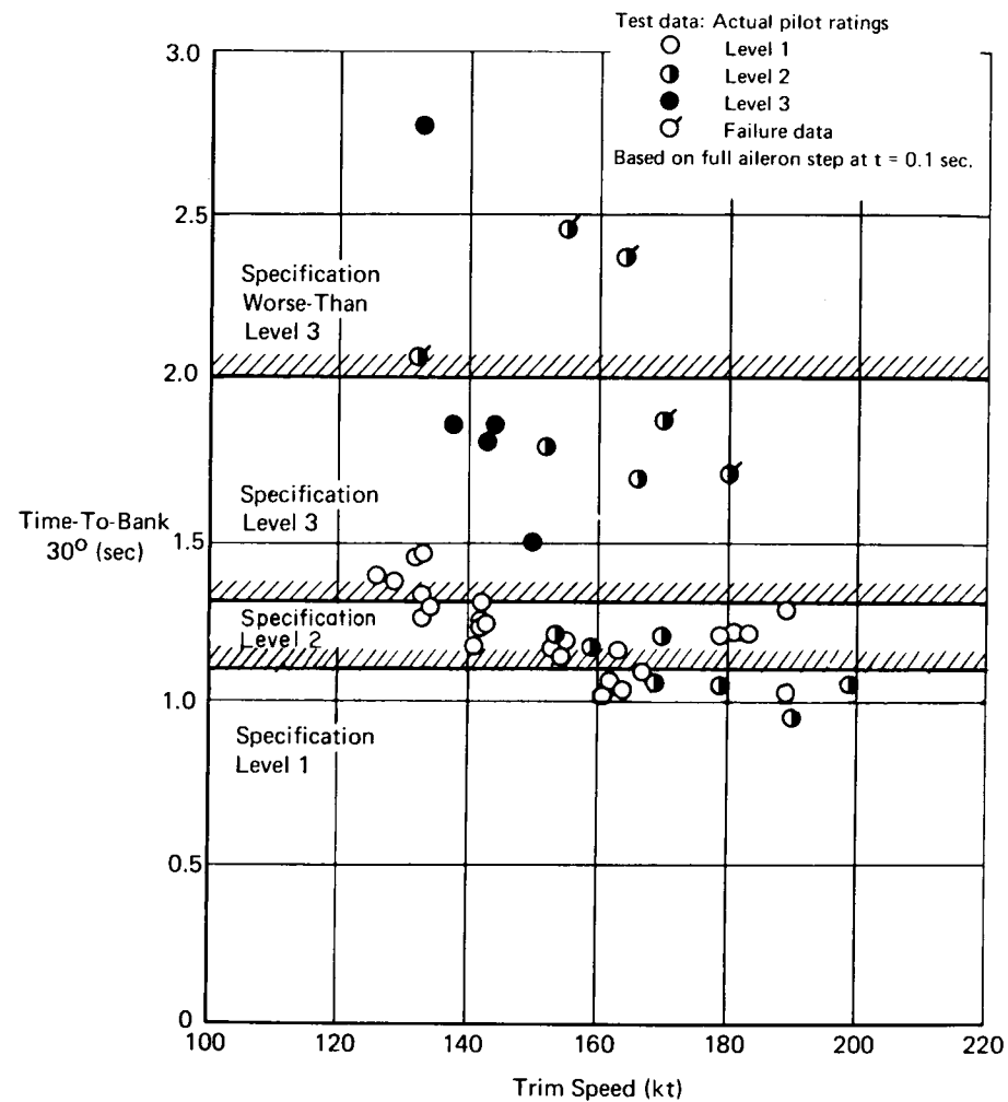
FIGURE 178. F-4 roll control effectiveness, time-to-bank 90°, CR configuration (from AFFFDL-TR-70-155).
