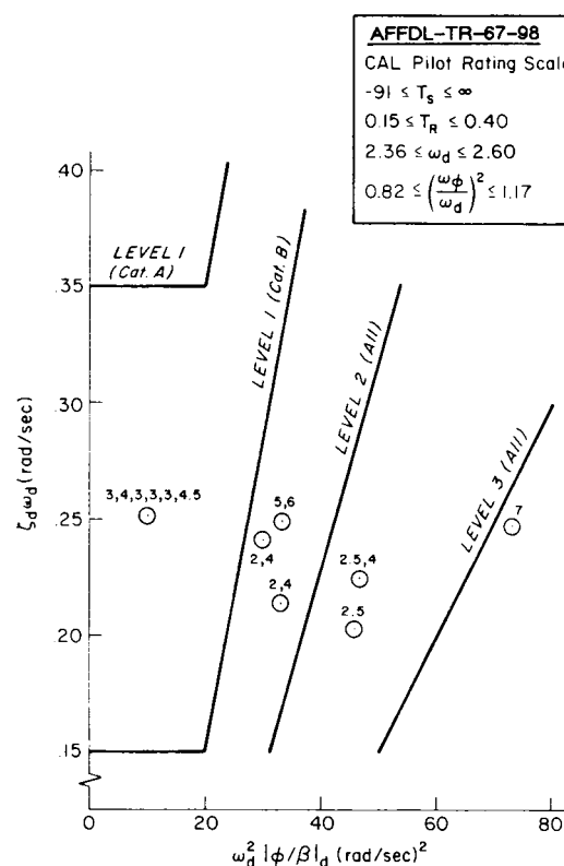
FIGURE 216. Dutch roll data from in-flight simulation of AFFDL-TR-67-98.
