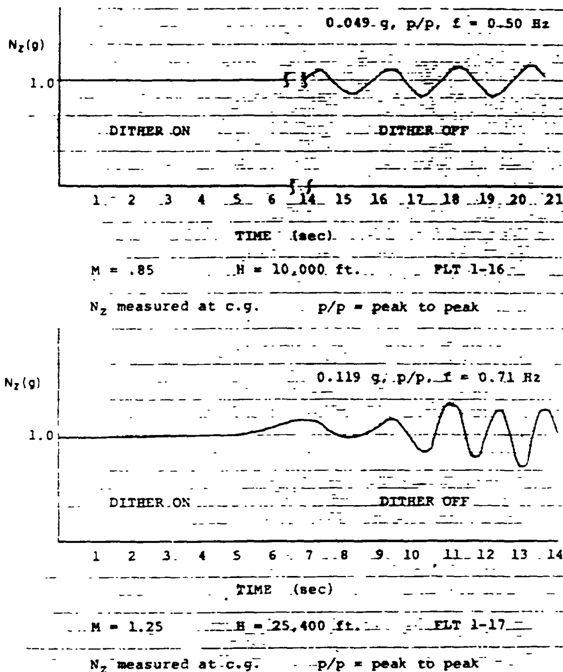
FIGURE 94. Effect of dither on B-1 limit cycle oscillations (from AFFTC-TR-79-2).
