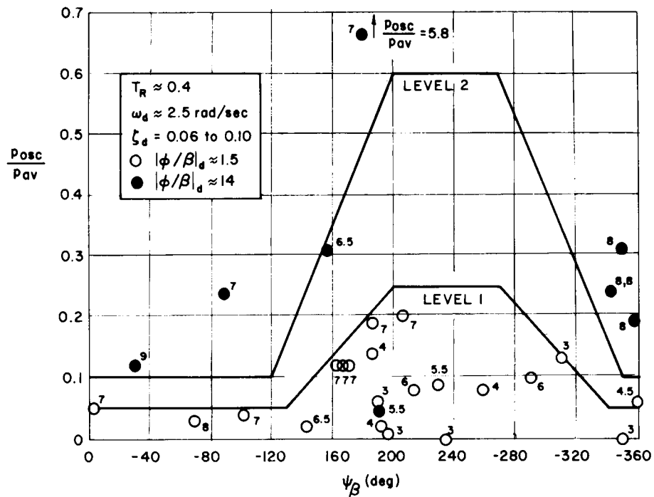
FIGURE 162. Flight phase Category A data, large and small |\phi/\beta|_d (from AFFDL-TR-67-98).
