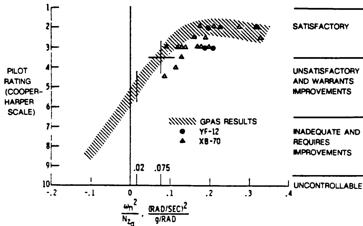
FIGURE 50. Comparison of YF-12 and XB-70 handling qualities evaluation with the GPAS results (NASA-CR-159236).
