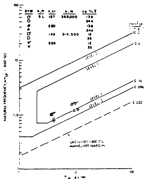
c) L-1011 power approach configuration.
