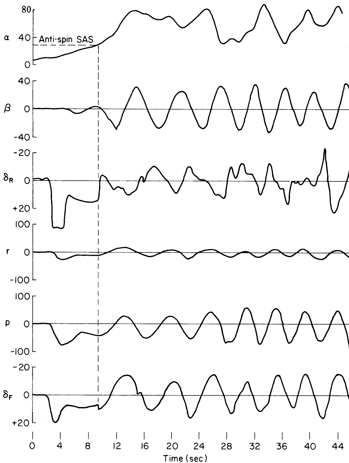
FIGURE 255. Time history of aft-c.g. deep stall encountered by F-16B
