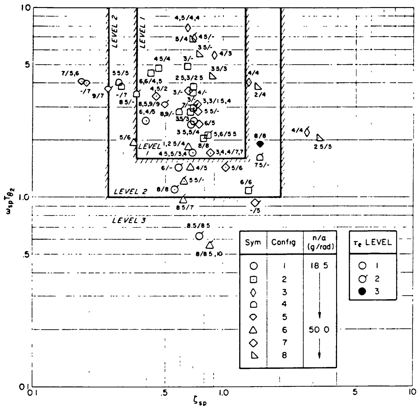
FIGURE 44. Comparison of Neal-Smith LOES characteristics with \omega_{sp} T_{\theta_2} vs \zeta_{sp}
