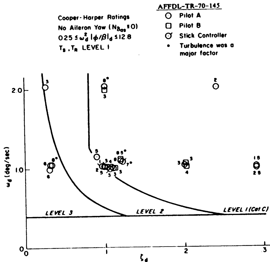
FIGURE 220. Dutch roll data from In-flight simulation of Class II-L airplanes in landing approach (T-33; AFFDL-TR-70-145).
