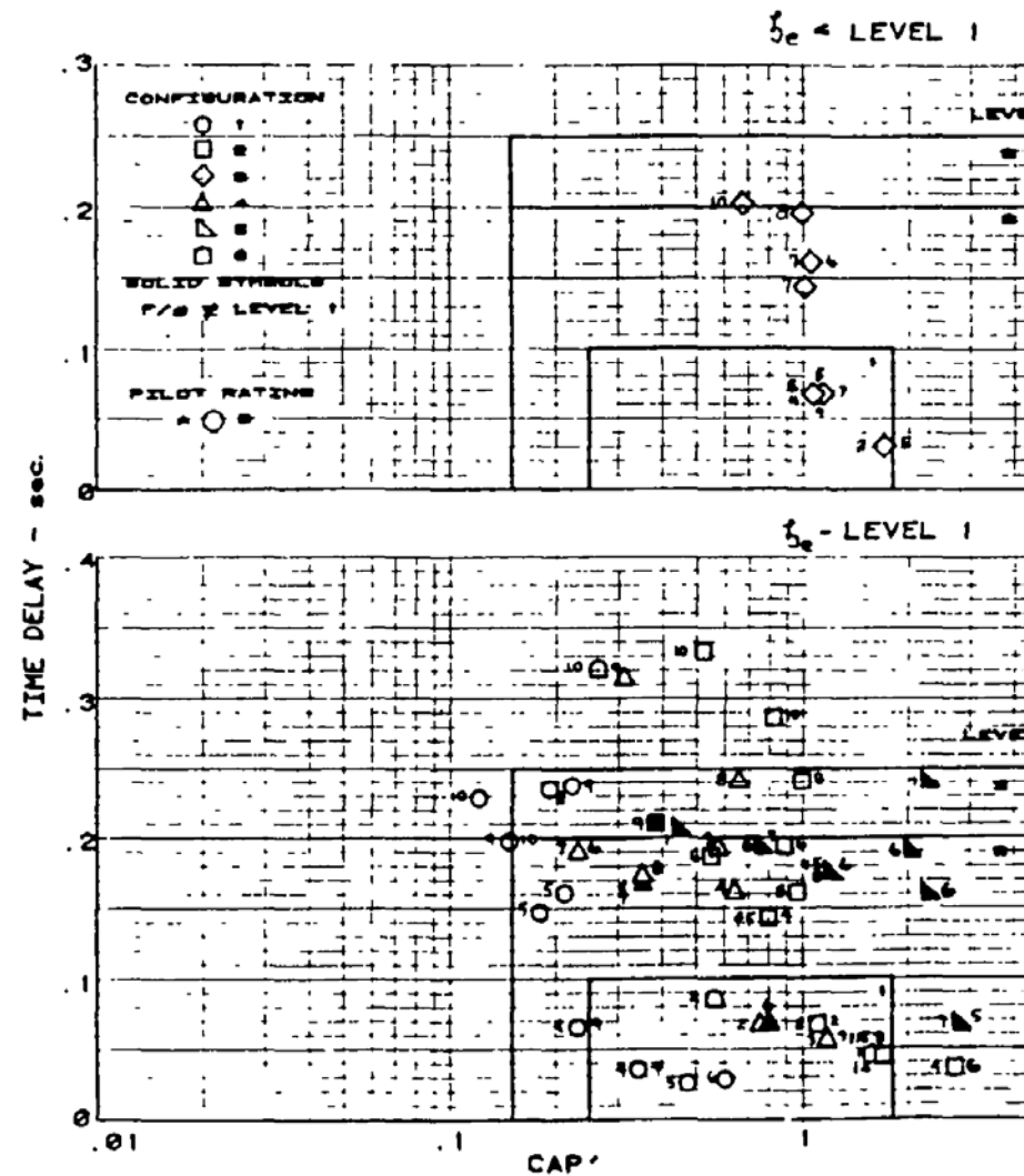
FIGURE 23. Time delay versus CAP' - LAHOS data (from
