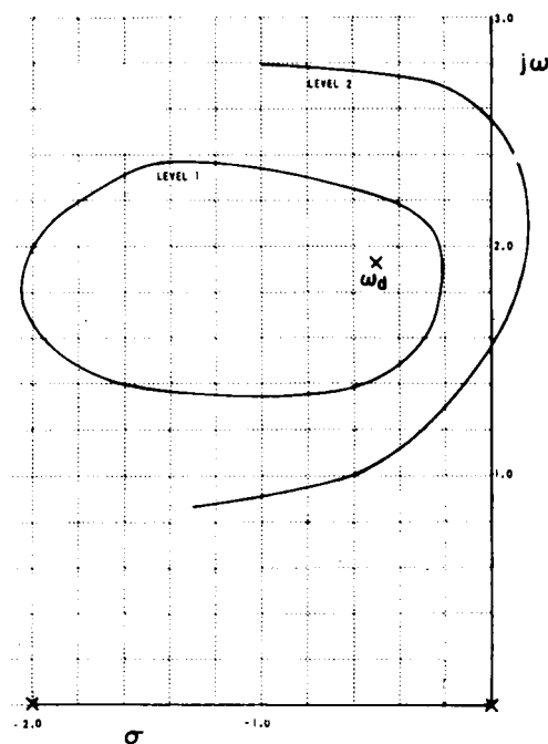
b) \omega_d = 2 \text{ rad/sec} ; \zeta_d = 0.25
