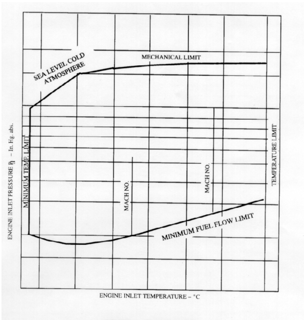
FIGURE 1. Operating limits.
