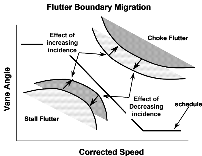
FIGURE 9. Flutter boundary margin.
