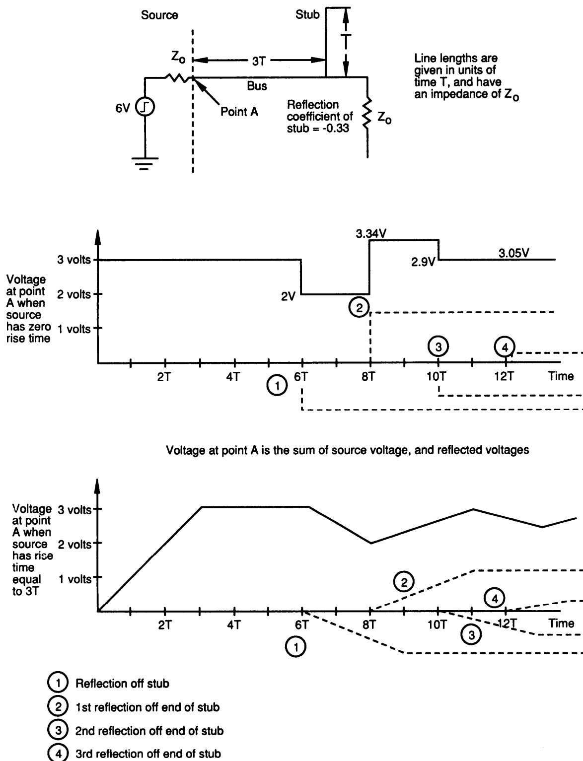
Figure 40-10. Reflective Distortion Caused by a Direct-Ccoupled Stub(Lossless Case)
