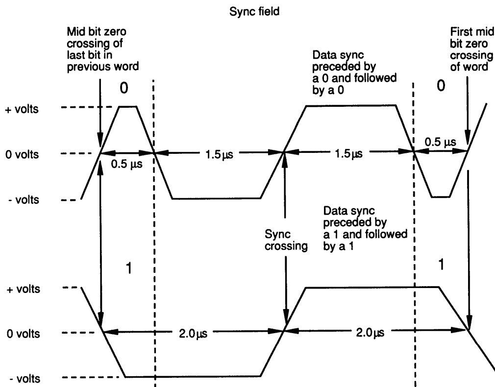
Figure 40-4. Data Sync
