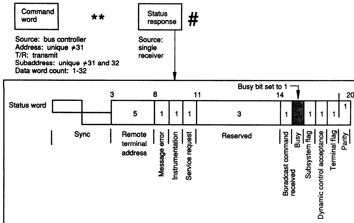
Figure 20-4. Busy Bit
