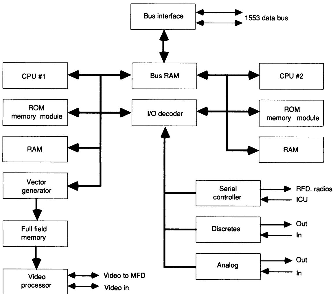
Figure 70-9. MCPU Architecture
