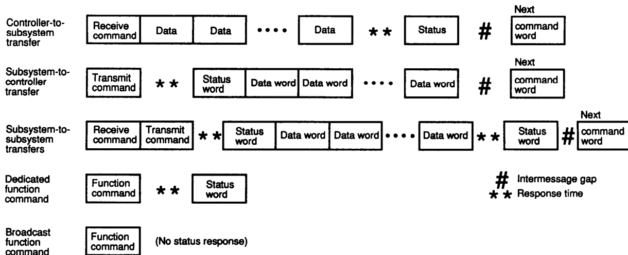
Figure 70-20. F-16 1553 Message Formats
