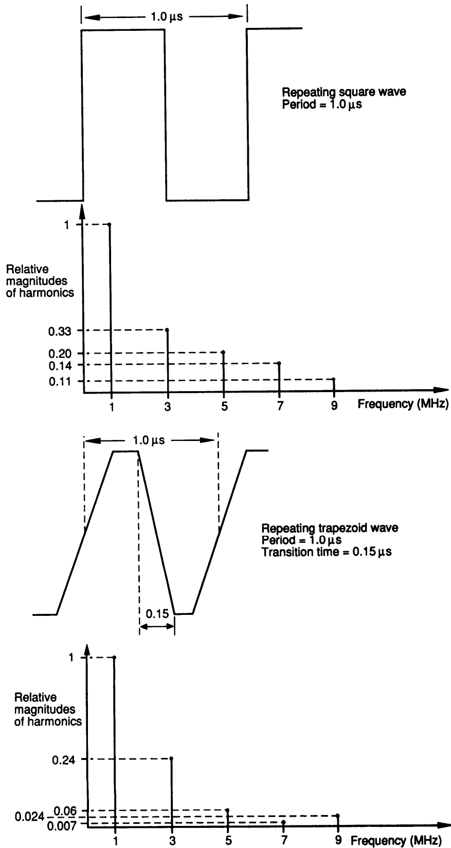
Figure 40-7. Harmonics of Square Wave Versus Trapezoid Wave
