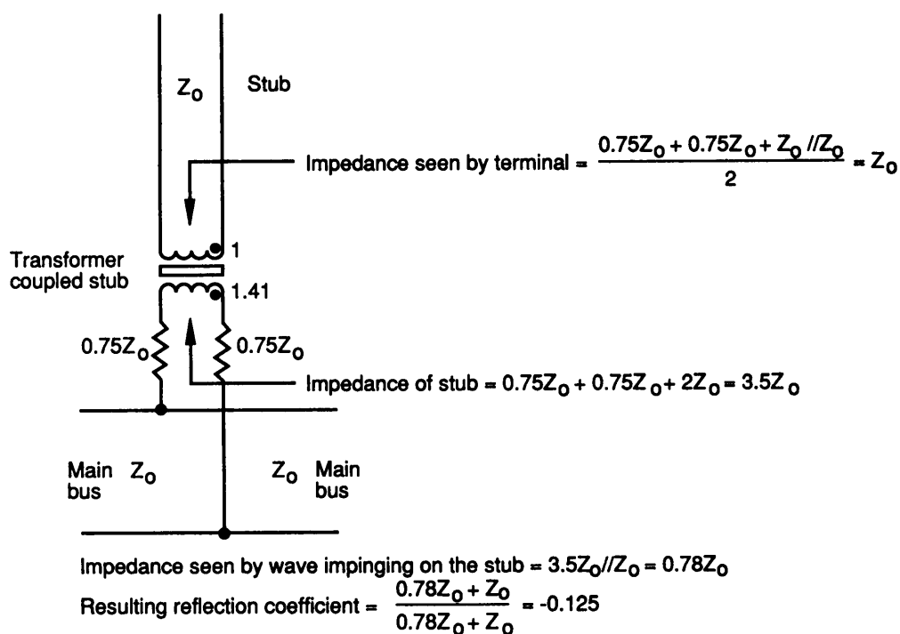
Figure 40-8. Impedance Calculation for Transformer-Coupled Stub
