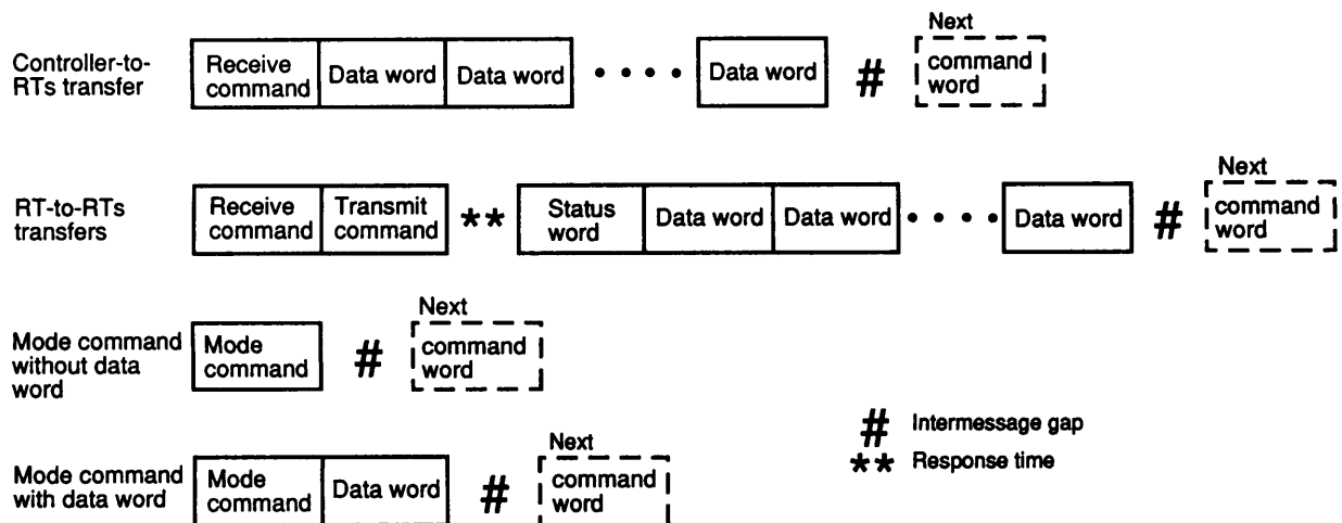
Figure 7 of 1553B. Broadcast Information Transfer Formats
