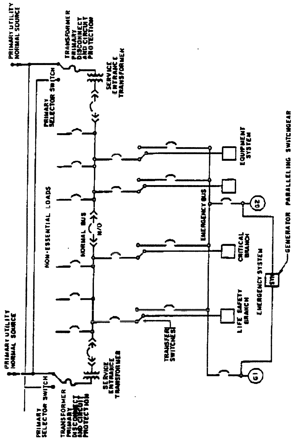
FIGURE 10--EMERGENCY OUTLINE DIAGRAM
