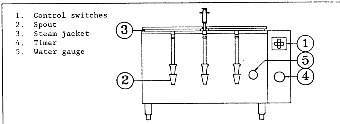
Figure 7 Major Urn Components
