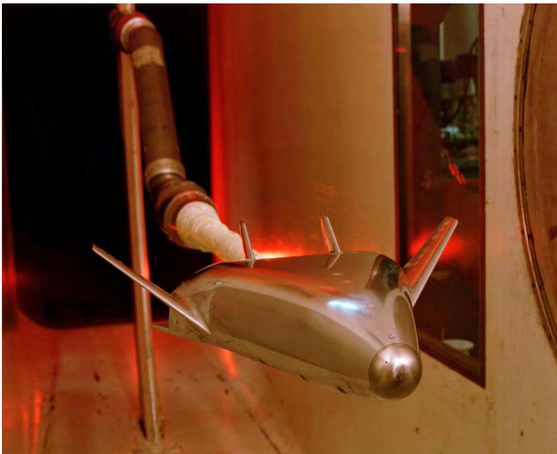
Figure 3-42. The photo shows a metal model of the X-33 reusable launch vehicle (about 15 inches [38 centimeters] long by 15 inches wide) being tested for the Lockheed Martin Skunk Works in Langley's Low-Turbulence Pressure Tunnel. The subsonic tests were conducted at a speed of Mach 0.25. (NASA-LaRC photo EL-1997-00041).
