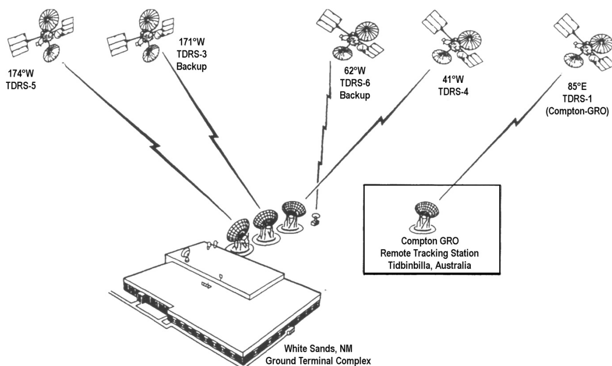
Figure 4-11. The TDRS system with five orbiting satellites (two operational satellites and three backups) after the launch of TDRS-6 (F) in 1993 (STS-54 press kit).
