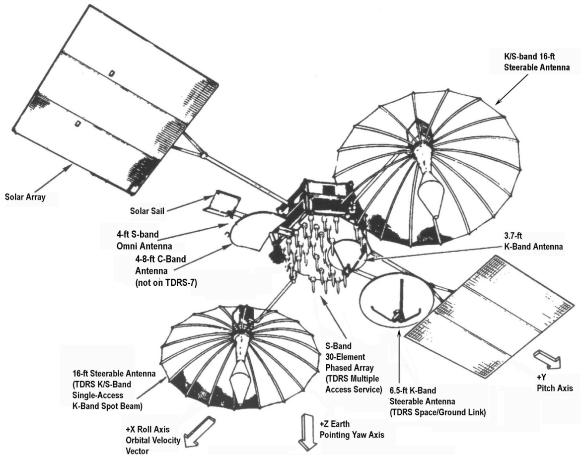
Figure 4-12. TDRS on-orbit configuration (Derived from STS-43 press kit).
