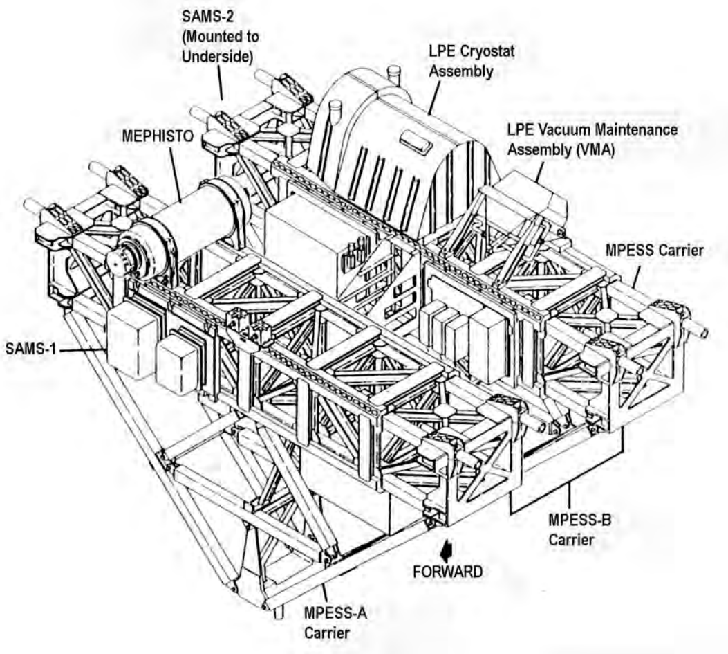
Figure 2-35. The USMP carrier consists of two Mission Peculiar Equipment Support Structures (MPESSs) that support the Lambda-Point Experiment, MEPHISTO, and Space Acceleration Measurement Systems apparatus (STS-52 Press Kit).
