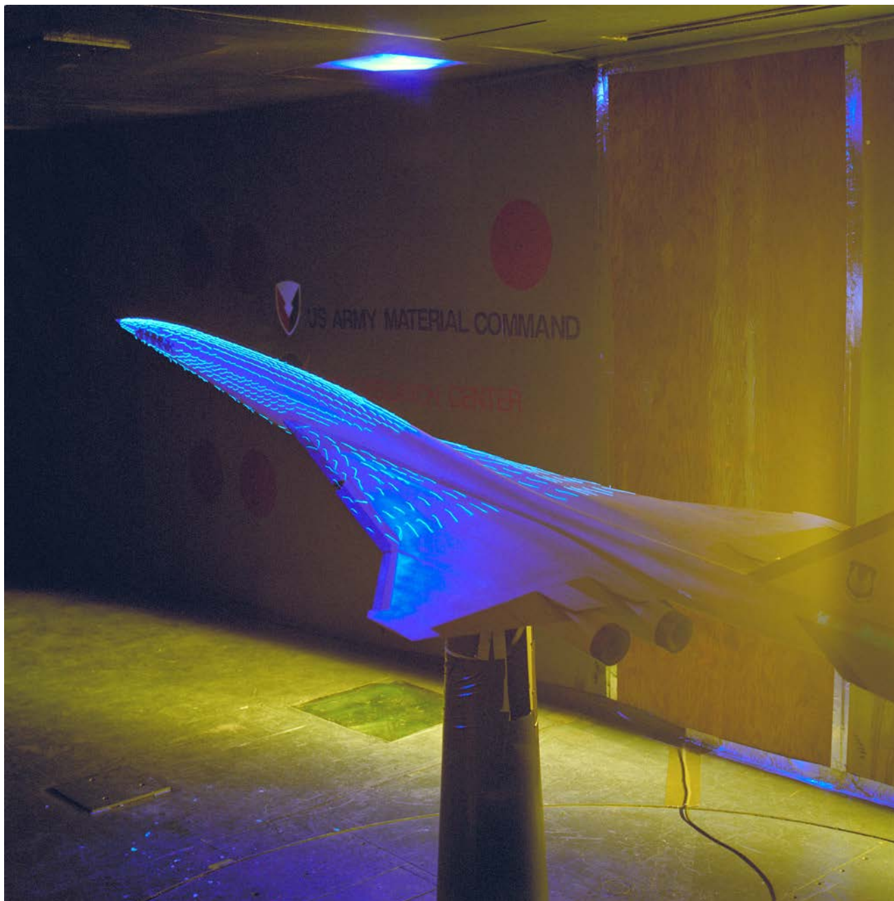
Figure 3-33. This photo shows the Boeing High-Speed Civil Transport being tested in ultraviolet light with tufts in the no. 1 7- by 10-foot wind tunnel. (NASA-ARC photo AC96-0047-47).
