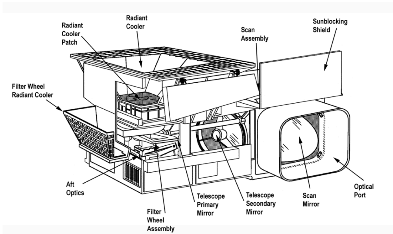
Figure 2-23. GOES Sounder (NASA GOES Project).
