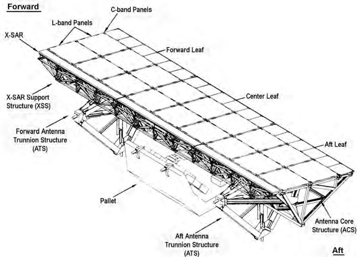
Figure 2-37. The SIR-C and X-SAR located on a Spacelab pallet in the Shuttle's payload bay on STS-59 (STS-59 Press Kit).
