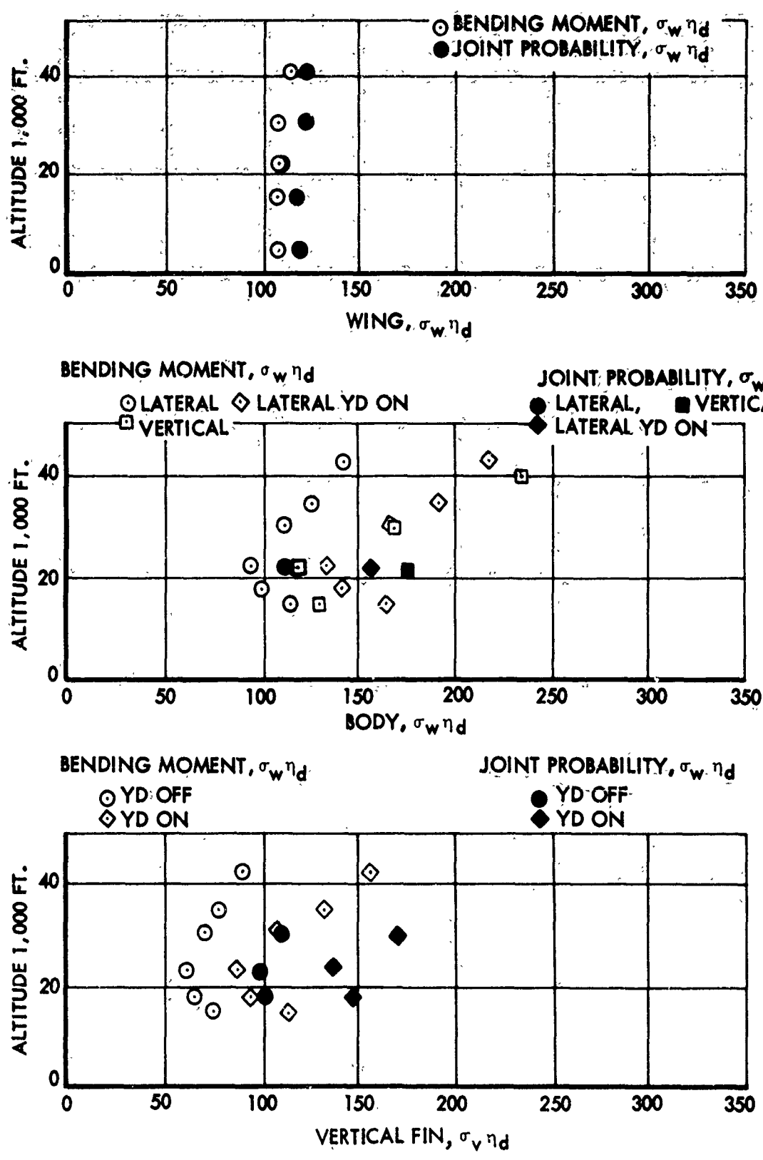
FIGURE 85. SUMMARY OF CRITICAL VALUES OF \sigma_w \eta_d
