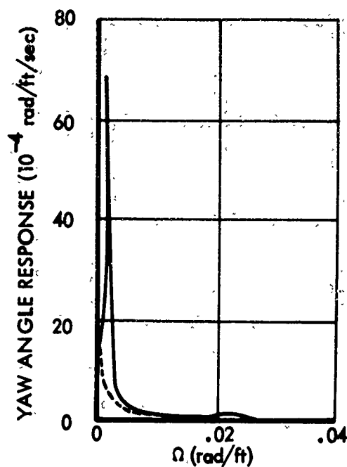
FIGURE 28b. FREQUENCY RESPONSE, AIRPLANE YAW
